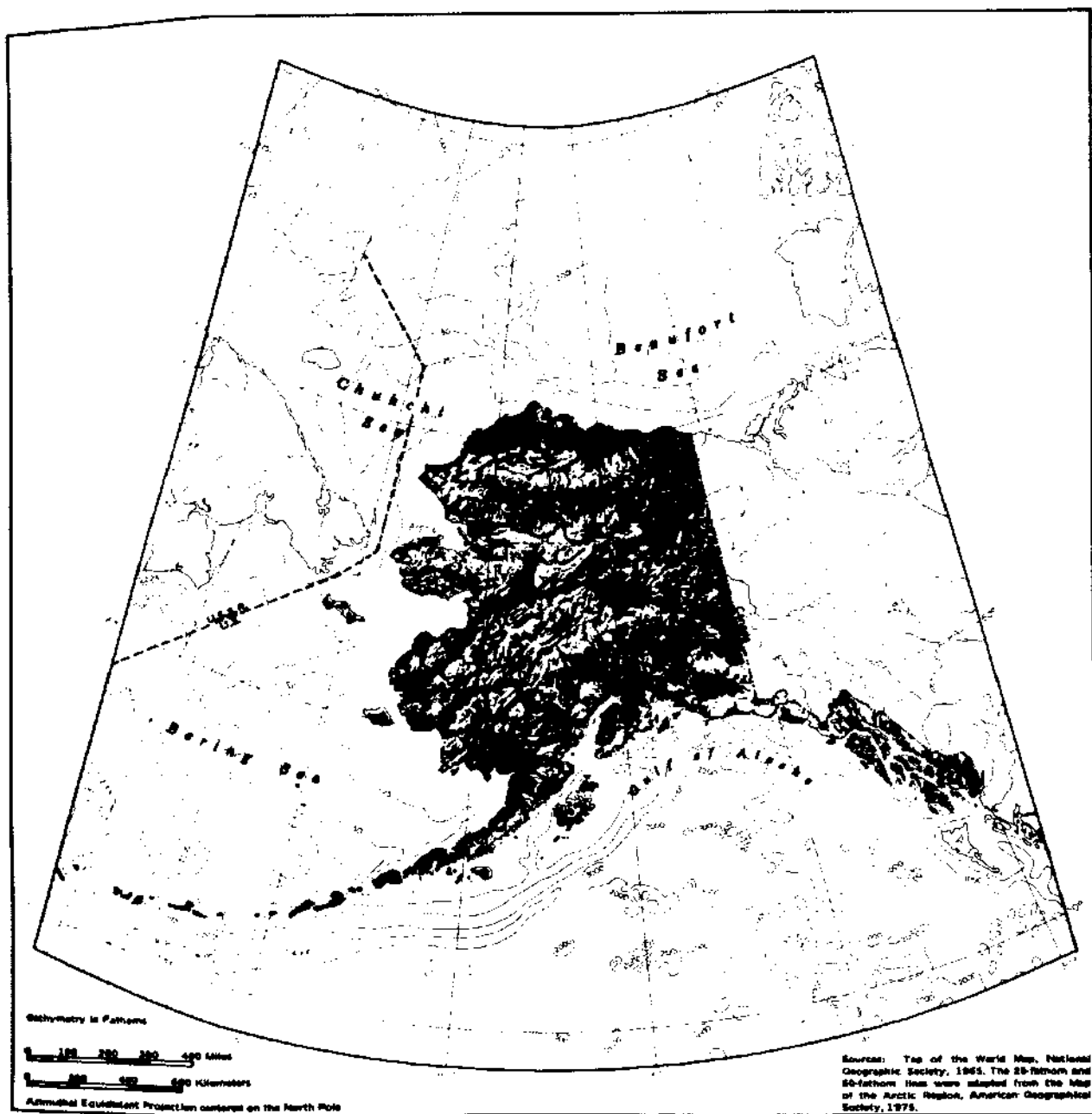
Figure 1. Alaskan continental shelf region (Brower et al. 1977).
