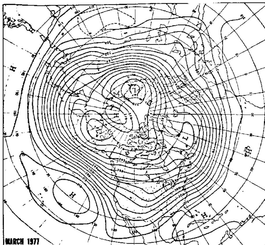
Figure 13. Mean 700 mb height contours (dam) for March 1977 (Taubensee 1977).
