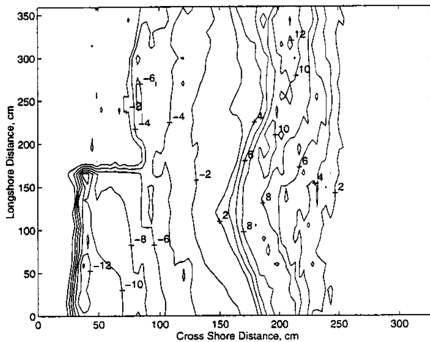
Figure 4-61: Contour plot of erosion during phase I of the wave sequence in Table 4.7. Constructed by subtracting Figure 4-53 from 4-59.
