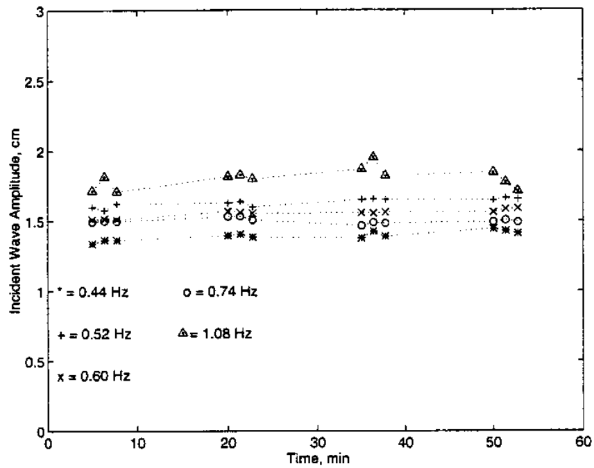
Figure 3-21: Incident amplitudes by spectral wave component on the sea wall beach for a T_{eq,norm} = 1.5 \text{ s} , H_{eq,norm} = 8.0 \text{ cm} wave.
