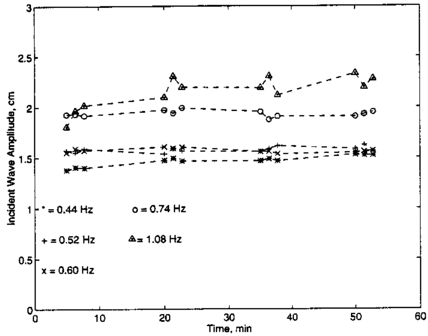
Figure 3-20: Incident amplitudes by spectral wave component on the dune beach for a T_{eq,norm} = 1.5 \text{ s} , H_{eq,norm} = 8.0 \text{ cm} wave.
