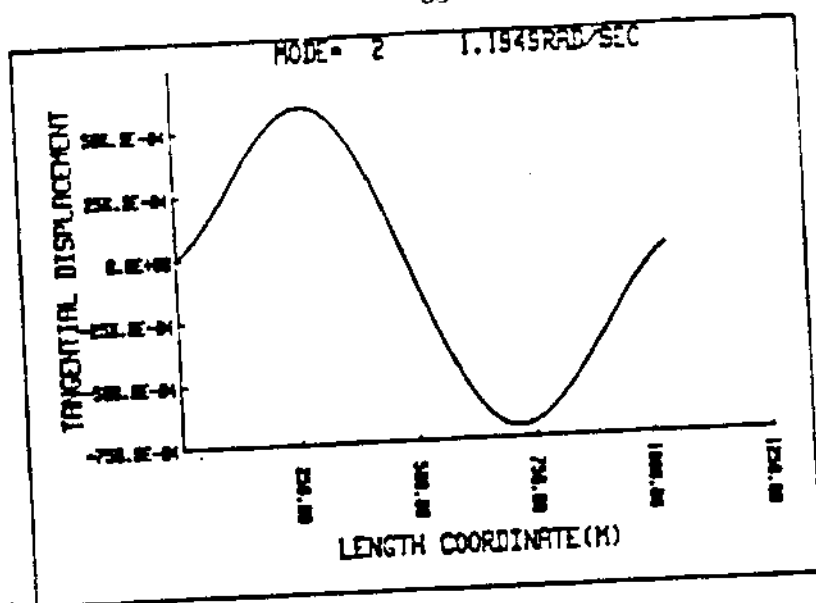
Figure 1-17: Second Mode of a Guy: Tangential Displacement
