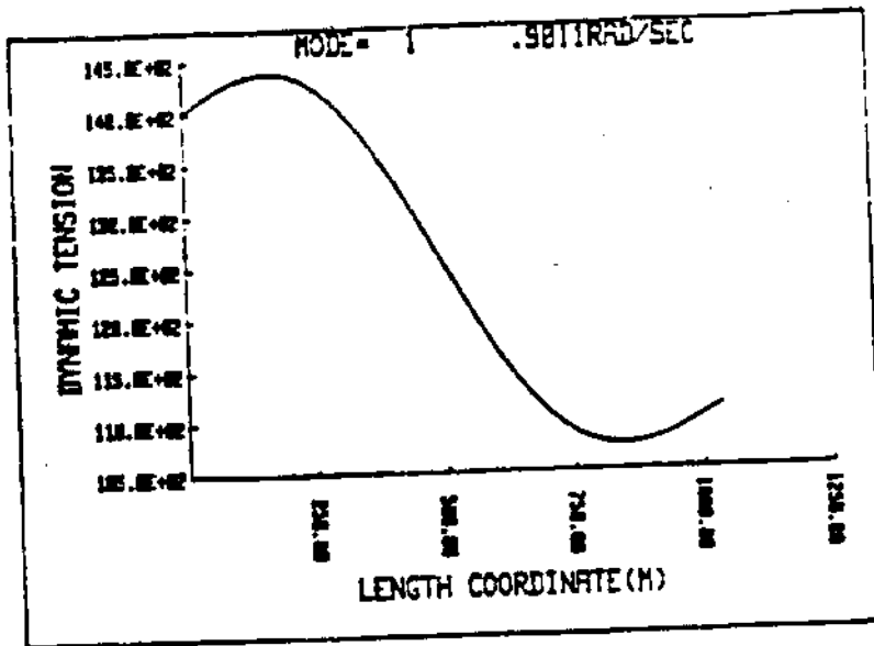
Figure 1-15: First Mode of a Guy: Dynamic Tension
