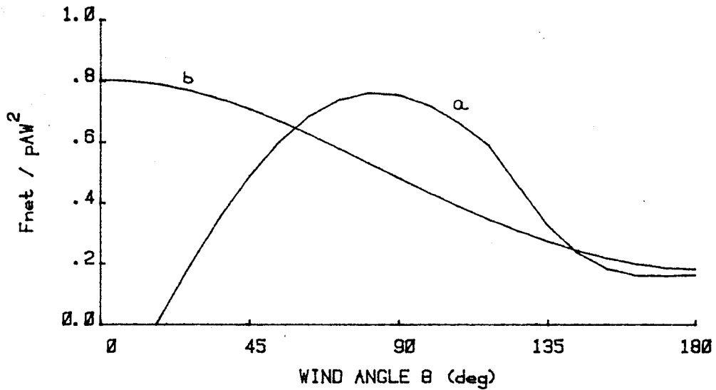
Normalized net forward force versus wind angle \theta for an aerofoil sail (a) and a windmill thruster (b). The boat is travelling at u = 0.5W .
