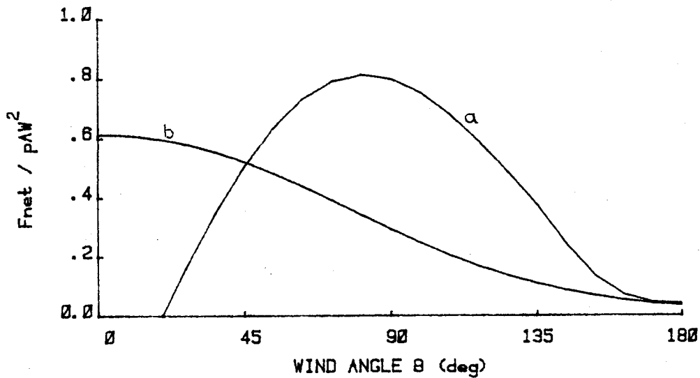
Same as Fig. (4), but with u = 0.75W .
