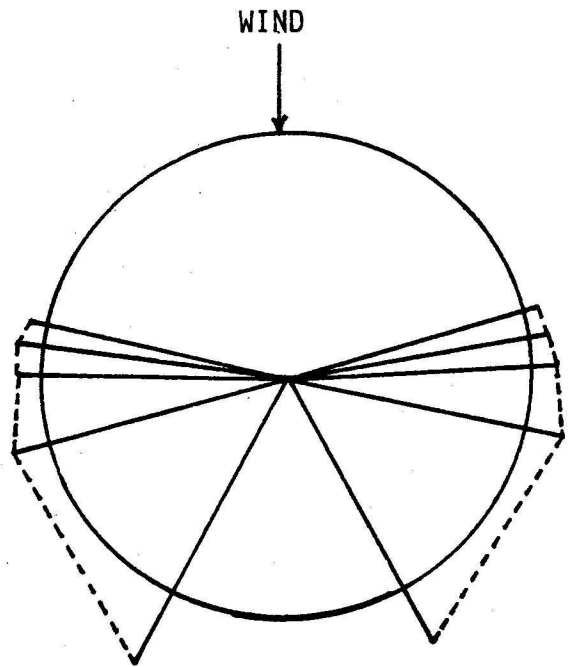
Figure 11. RPM = 1300 Power Alone (Ave.) = 5.1 knots Wind Velocity = 4.3-6.2 knots
