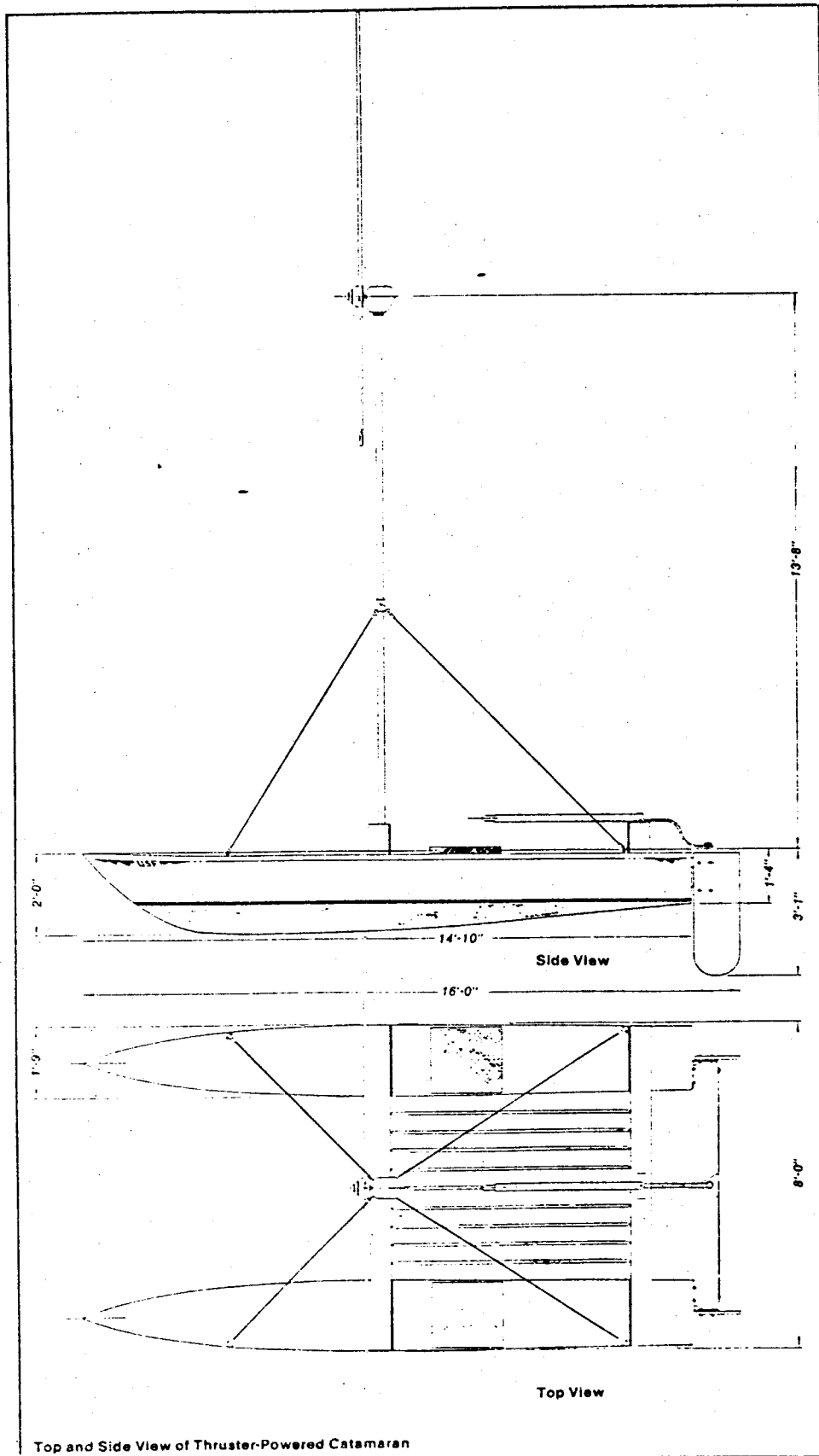
Top and Side View of Thruster-Powered Catamaran
