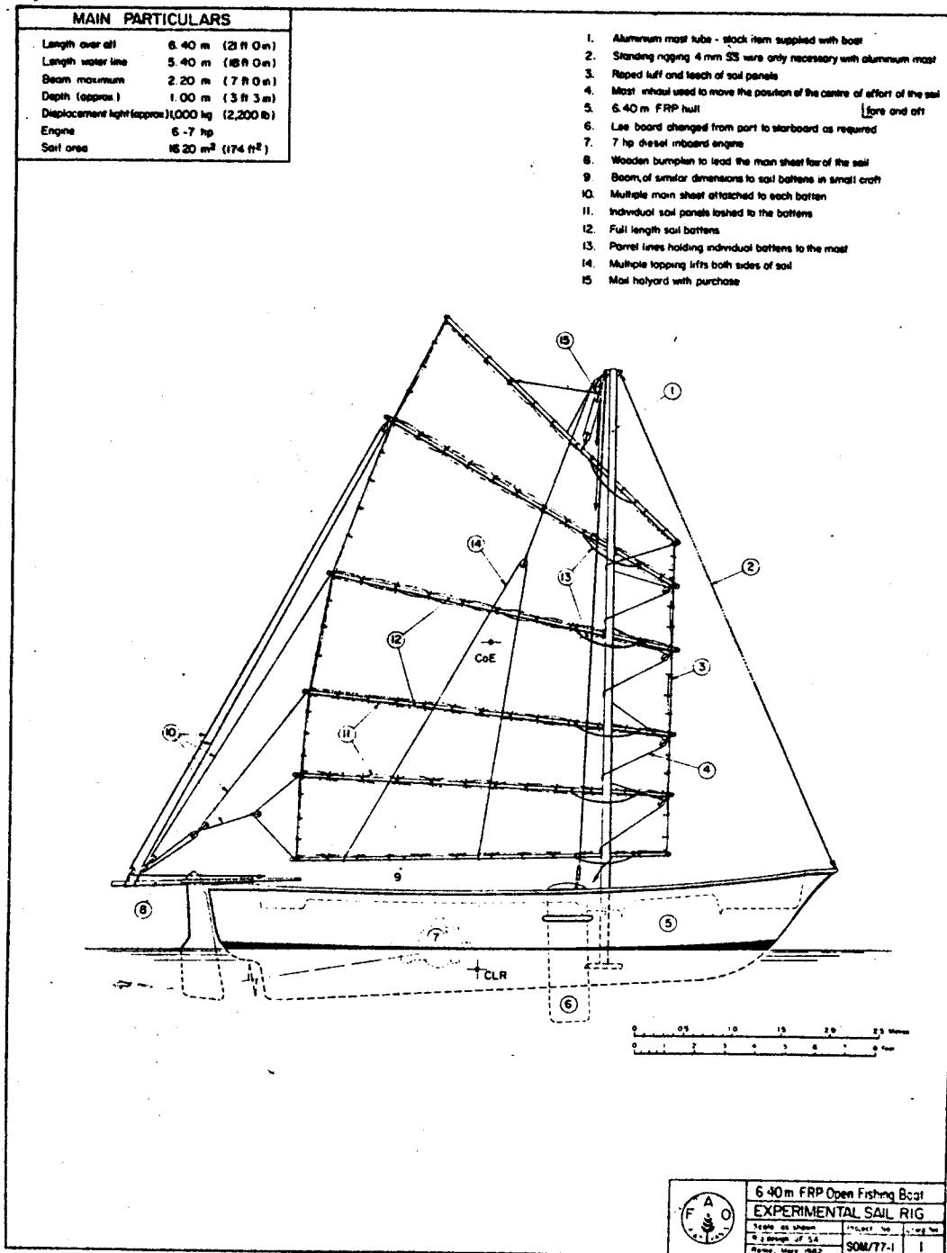
Arrangement and sail plan
