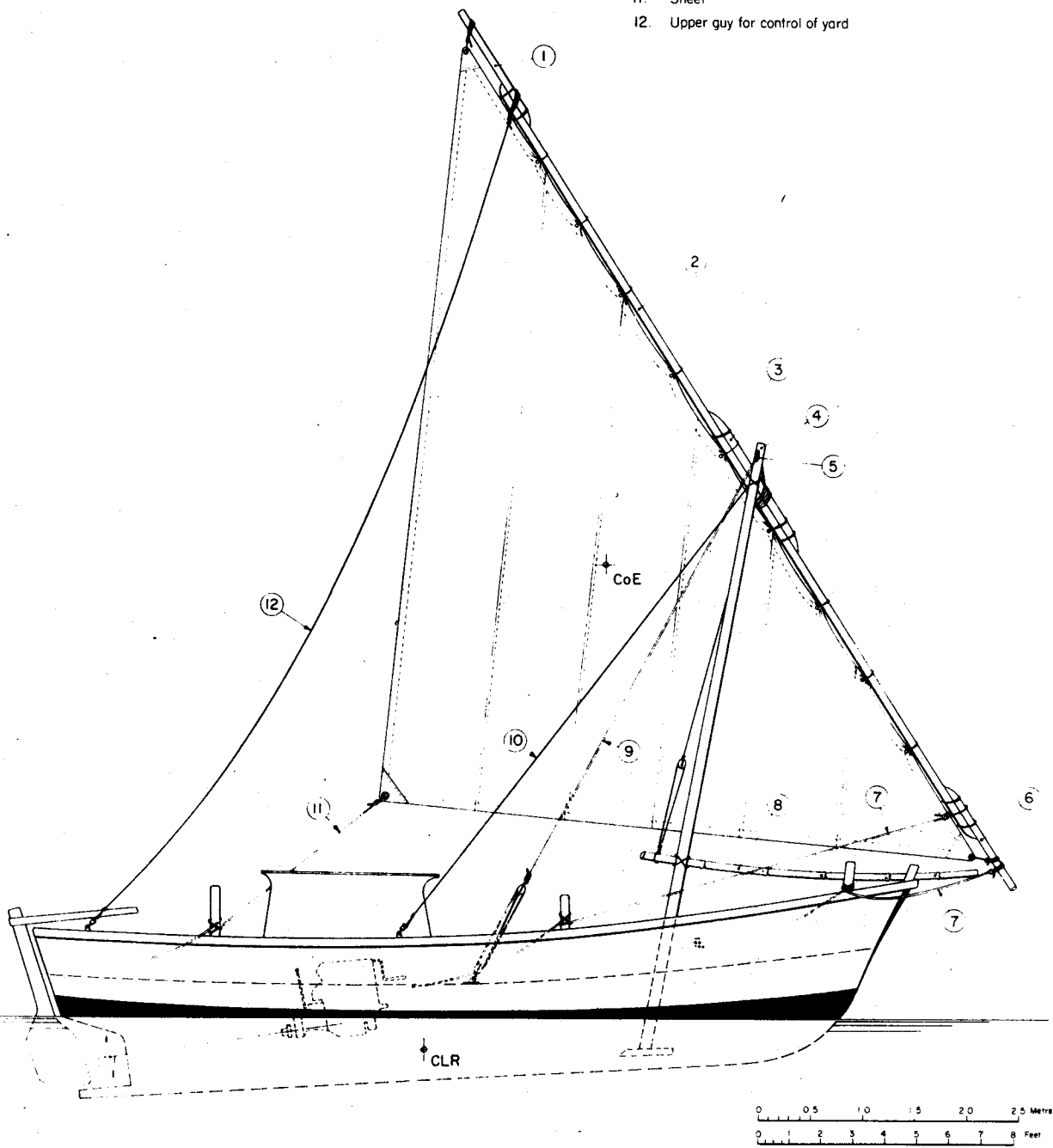
Fig. 16. Lateen rig fitted to the same hull as that of Fig. 9.
