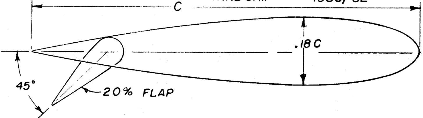
WIND SHIP 1980/82
