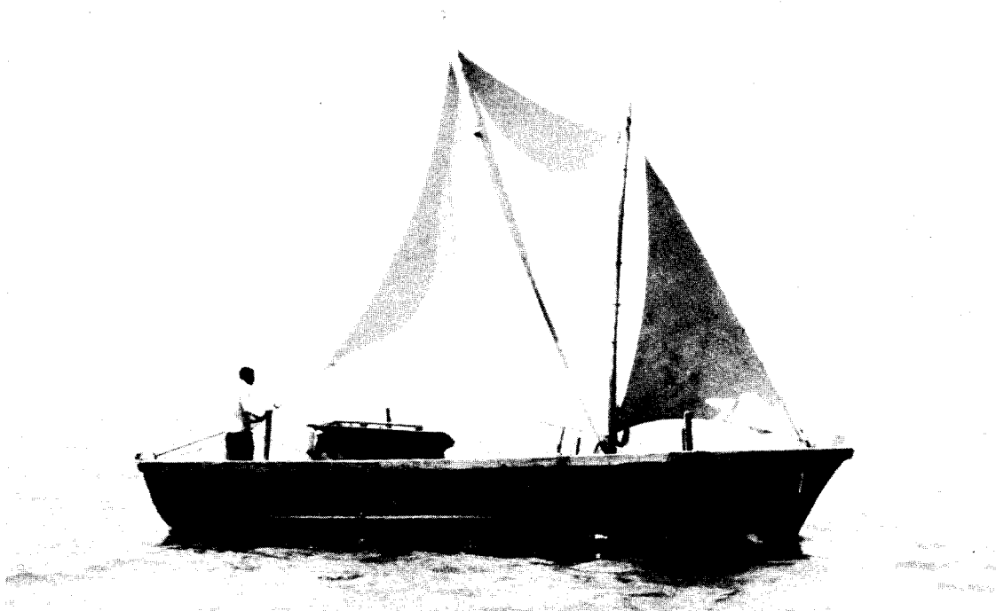
Fig. 7. 8.5 m (28 ft) fishing boat with sprit sail rig in Somalia
