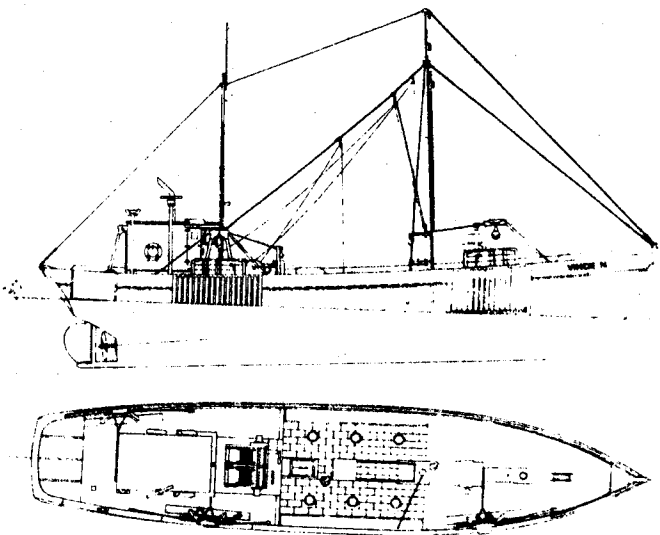
Outboard profile and deck plan of 86' side trawler Vincie N.
