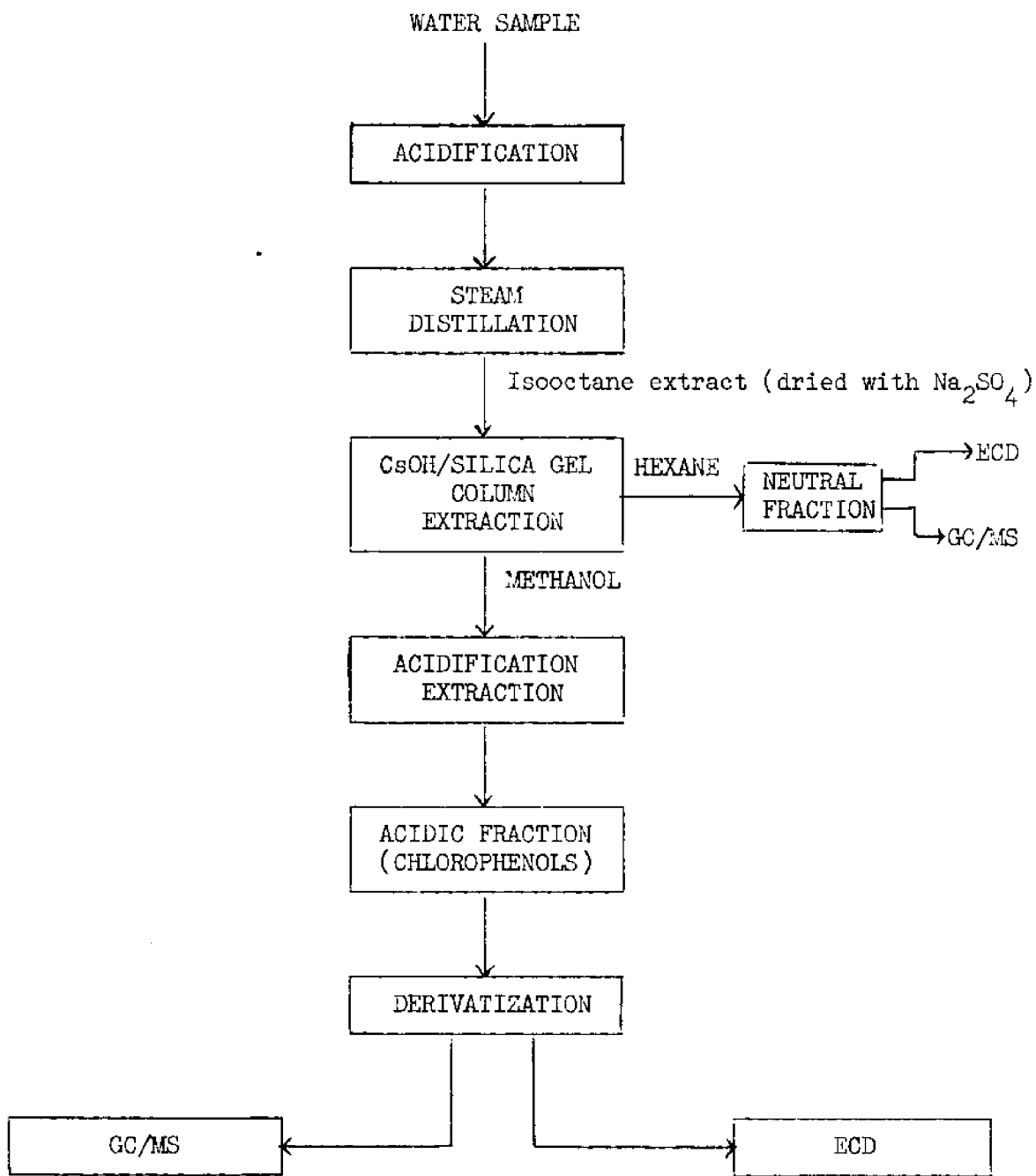
Figure 4 Schematic of the analytical procedure used for the identification of chlorinated organics in water.
