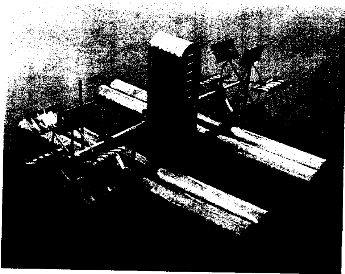
Figure 9. A 1-hp paddlewheel aerator. The impellers (paddle wheels) are welded into one piece. The floats are plugged PVC pipes. All exposed metal parts are stainless steel.
