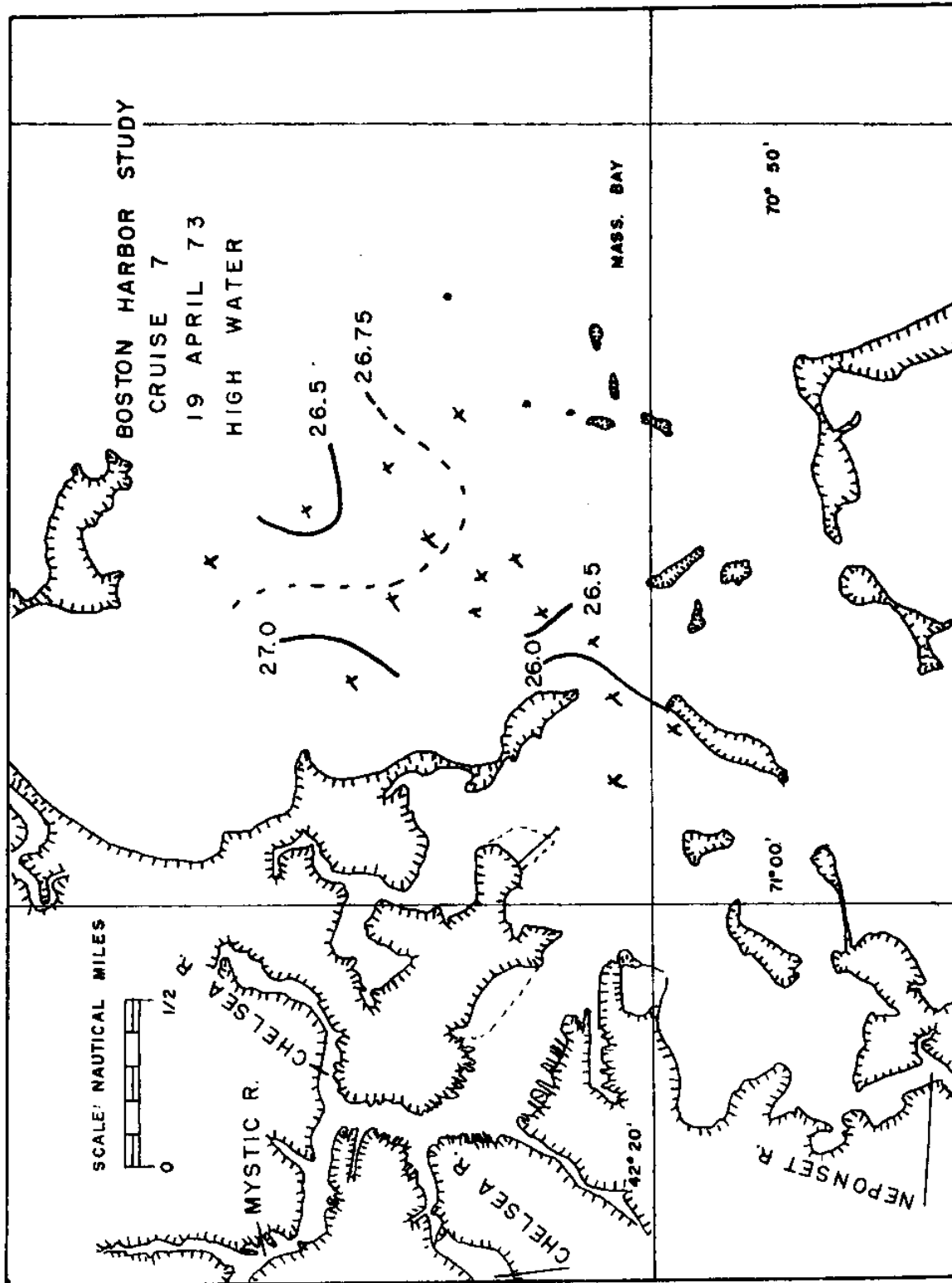
Figure 32 I.0 METER SIGMA - T
