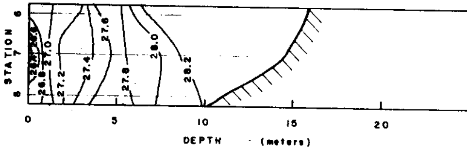
Figure 29 Times refer to hours after high water, Boston. Scale: 1 cm = 500 meters vertical distortion 250:1 0 hrs. 11 min. 12 hrs. 29 min.
