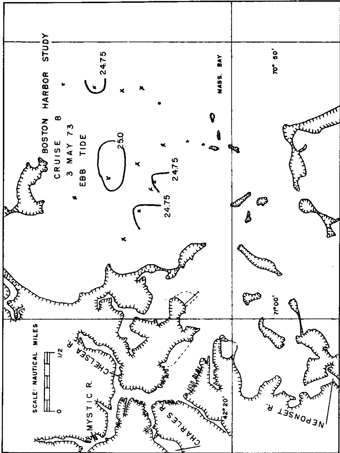
Figure 38 I.0 METER SIGMA-T
