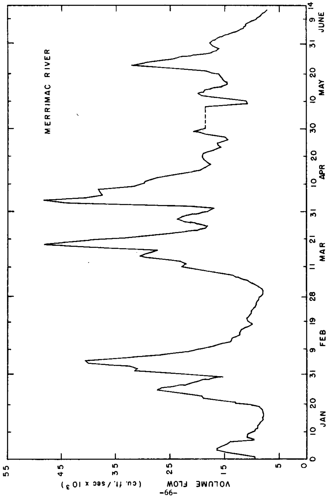
Figure 4.9: Daily Volume Flow of Merrimac River
