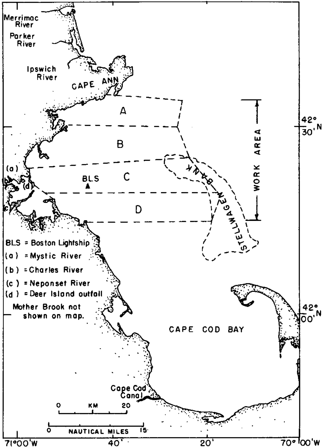
Figure 4.1: Map of Massachusetts Bay showing Region of Work and Sections into which Bay was divided to compute the Volume of Fresh Water
