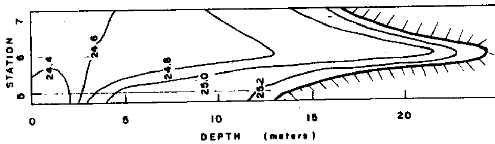
Figure 42 Times refer to hours after high water, Boston. Scale: 1 cm. = 500 meters 10 hrs. 56 min. 11 hrs. 9 min. vertical distortion 250:1
