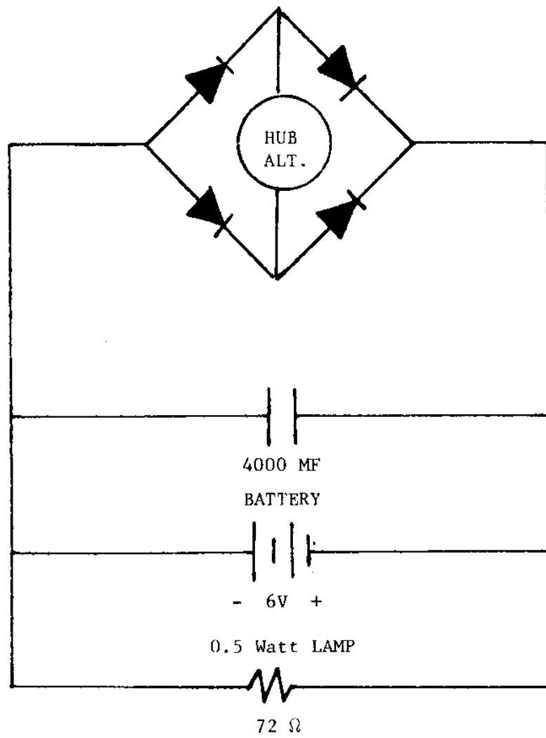
FIGURE 2.2.2.9 BATTERY CHARGING CIRCUIT
