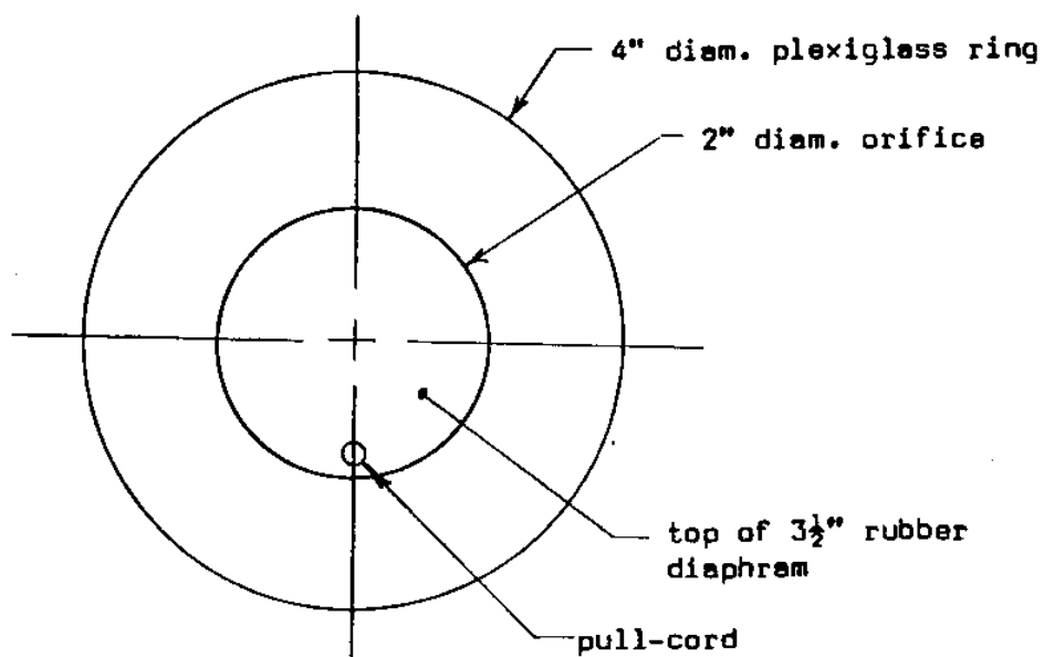
Fig. 2.9.3 Bleed-Off Valve
