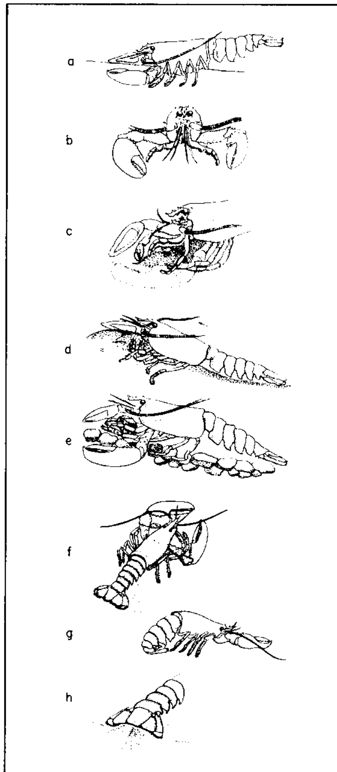
Figure 14. Burrowing behavior of the lobster. A-D) "bulldozing." E) "rock moving." F-G) "backwards dig." H) "pleopod fanning." From Cobb (23).
