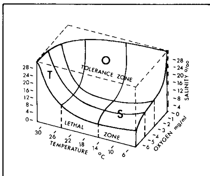
Figure 12. Three-dimensional graph of the tolerance of lobsters to oxygen, salinity, and temperature. Any point in the graph represents a specific combination of oxygen, temperature, and salinity. Redrawn from McLeese (95).
