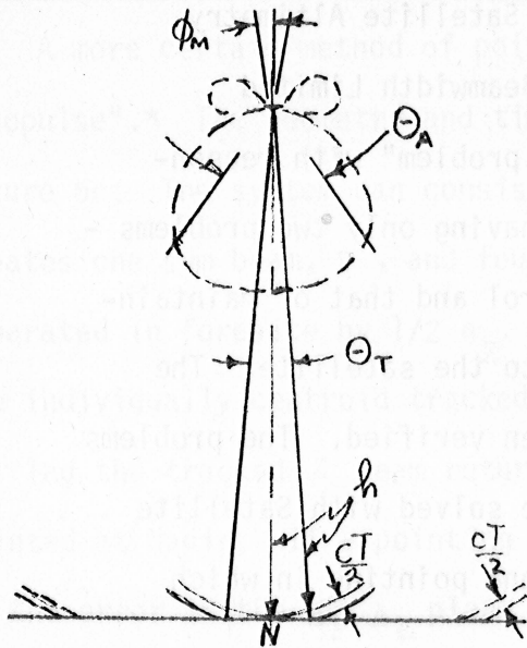
a. - PULSE ALTIMETER GEOMETRY
