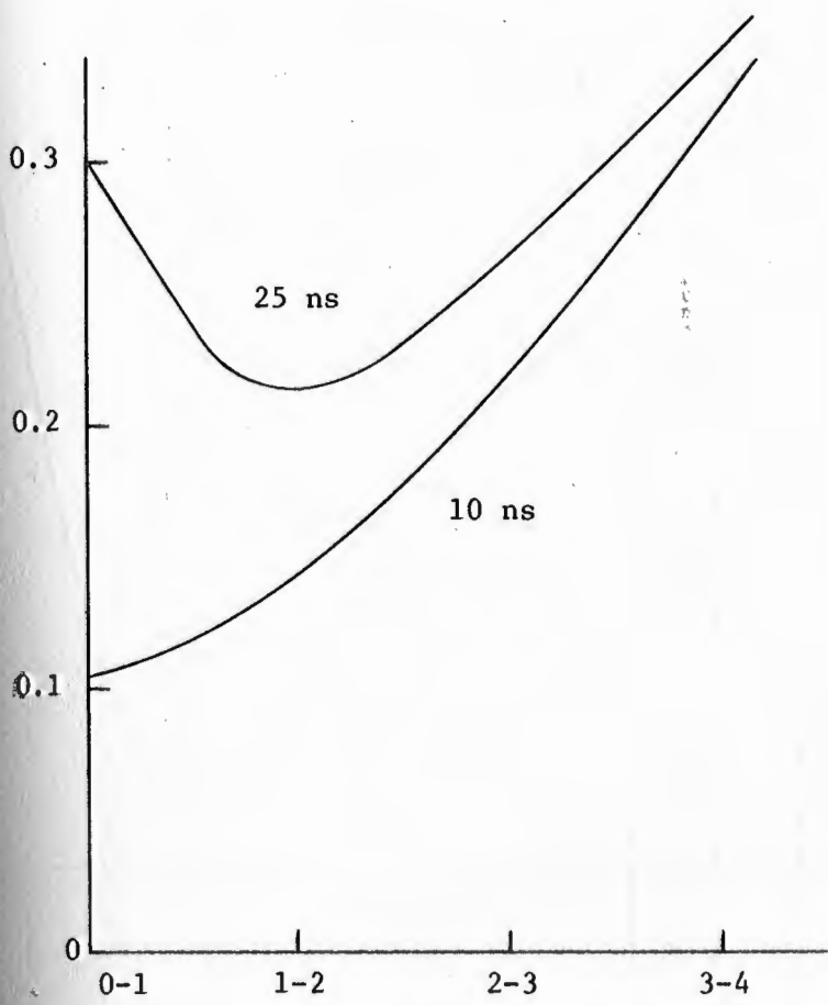
Figure 6. Calculated surface roughness measurement precision as a function of pulse length and sea conditions.
