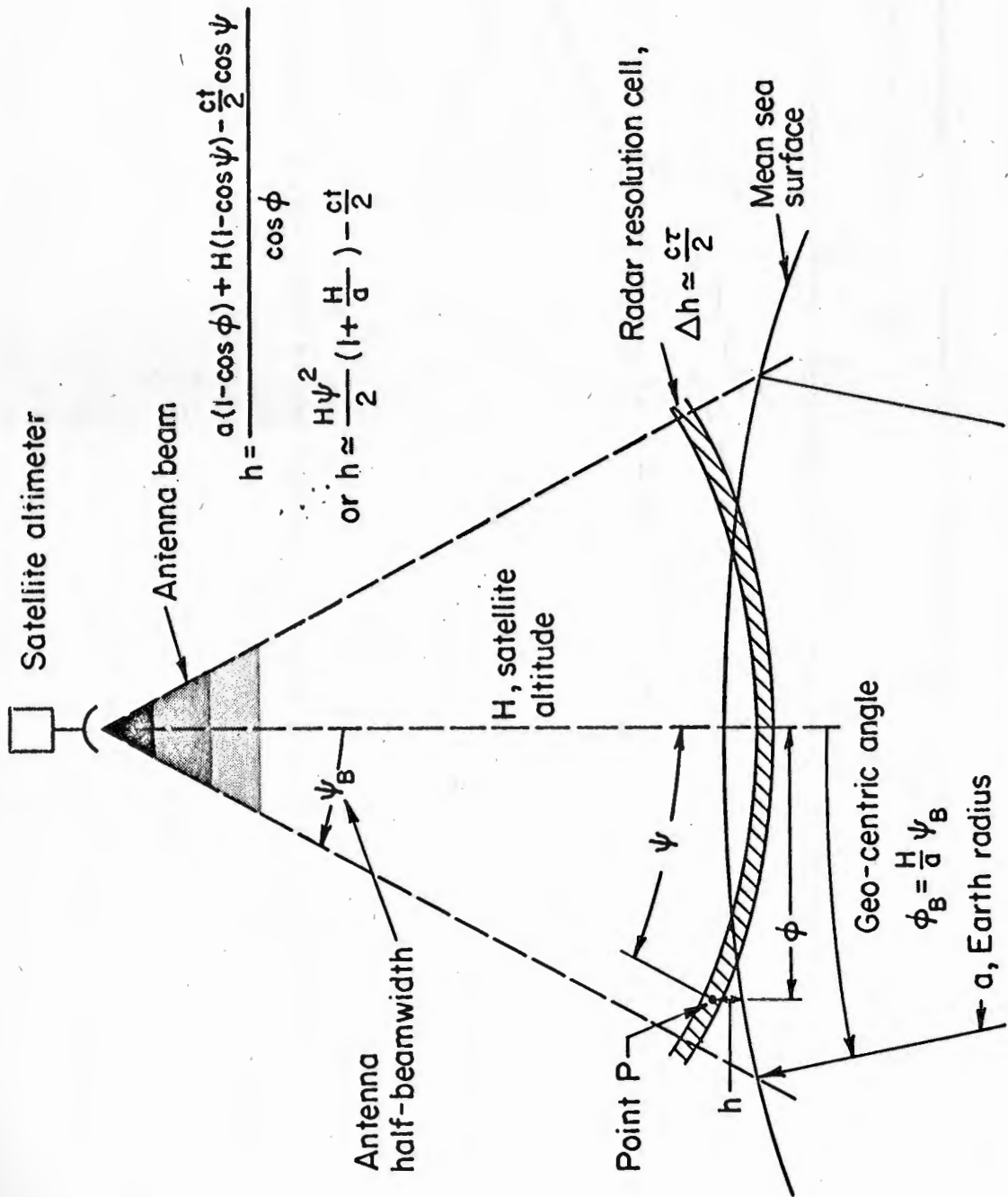
Figure 2. Geometry of Satellite Altimeter
