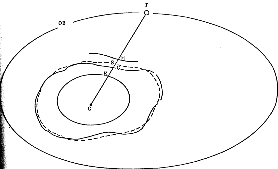
FIGURE 4. REPRESENTATION OF SURFACES ASSOCIATED WITH SATELLITE ALTIMETRY
