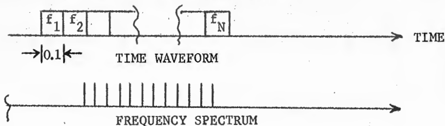
FIG. 2 STEP FREQUENCY PULSE COMPRESSION
