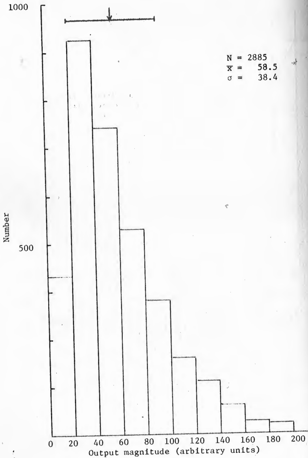
Figure 7. Histogram of simulated video filtered waveforms,
