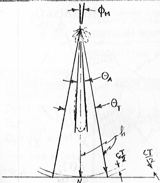
a. - PULSE ALTIMETER GEOMETRY
