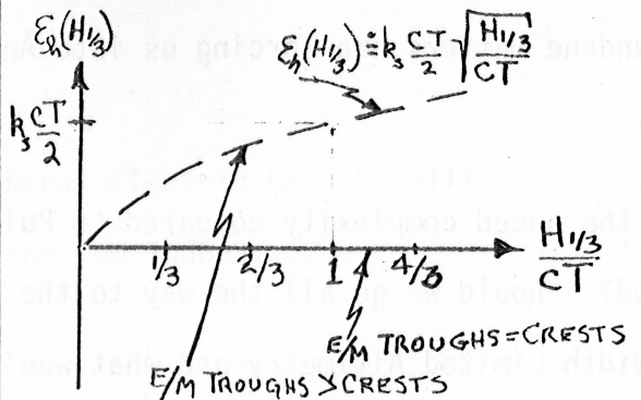
d. - SEA STATE DISPERSION
