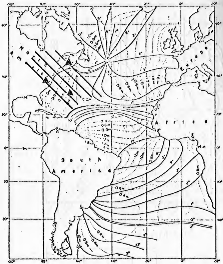
Theoretical tides of Atlantic Ocean. Full lines: co-tidal lines referred to moon's transition through meridian of Grw., dashed lines: co-range lines of the semi-diurnal tide M_2 in m (according to Hansen).
