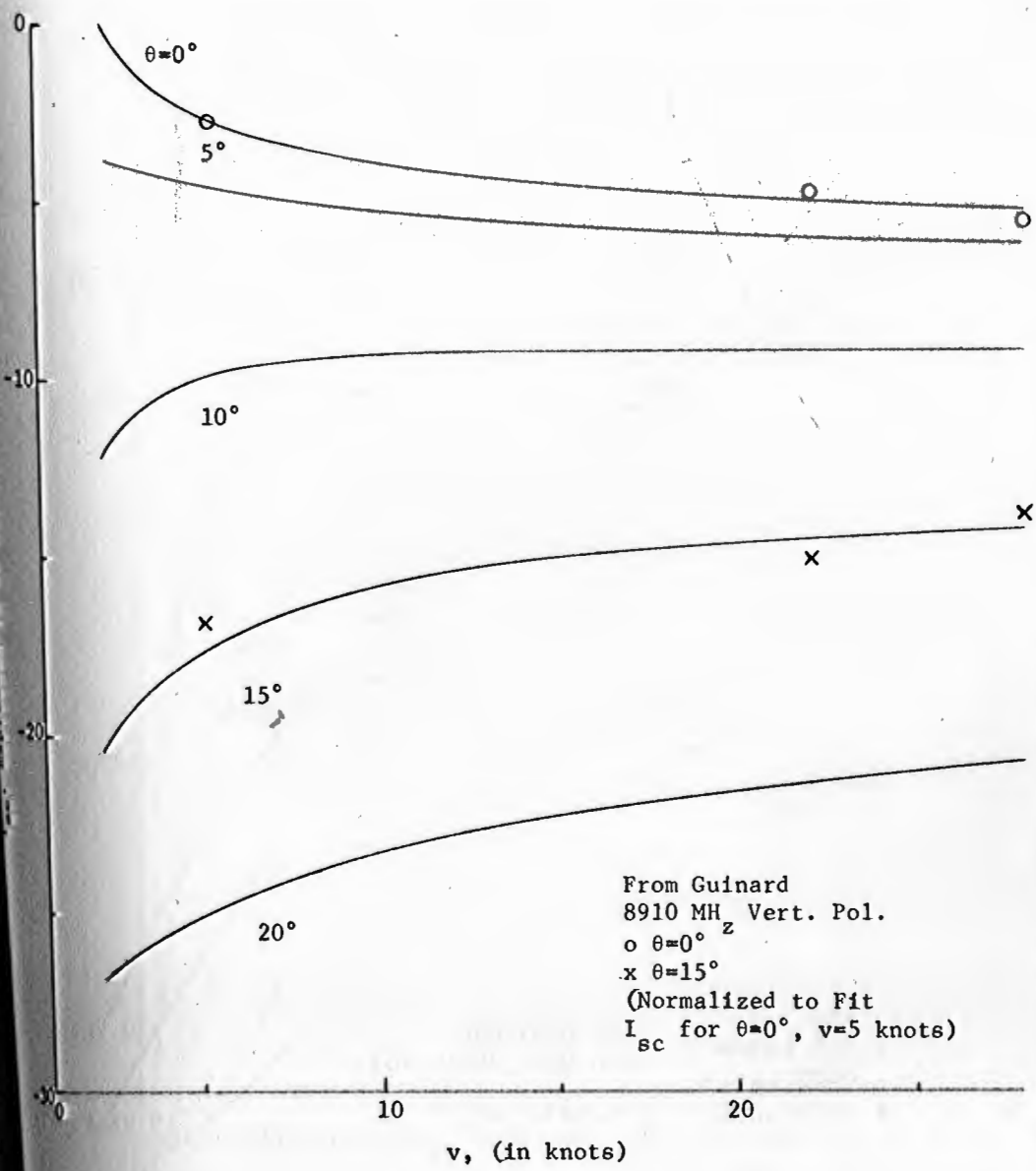
Figure 10. The scattering integral as a function of wind speed ( \lambda_{rf} = 3 cm.).
