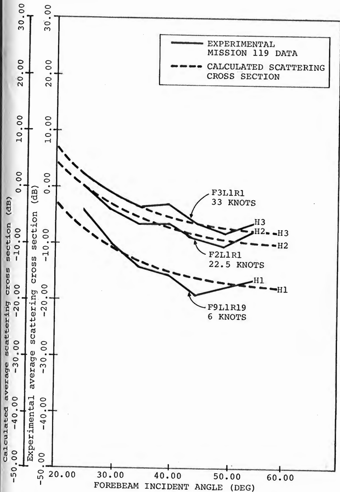
Figure 4. - Comparison of calculated and experimental scattering cross section for Mission 119.
