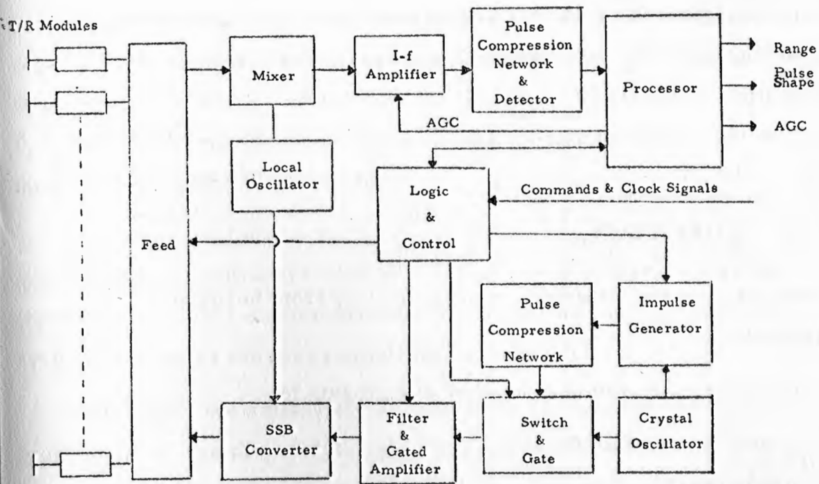
Figure 2 - Block Diagram of Solid-State Module System
