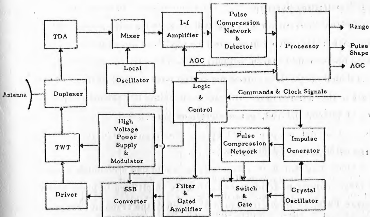
Figure 1 - Block Diagram of Single Transmitter System
