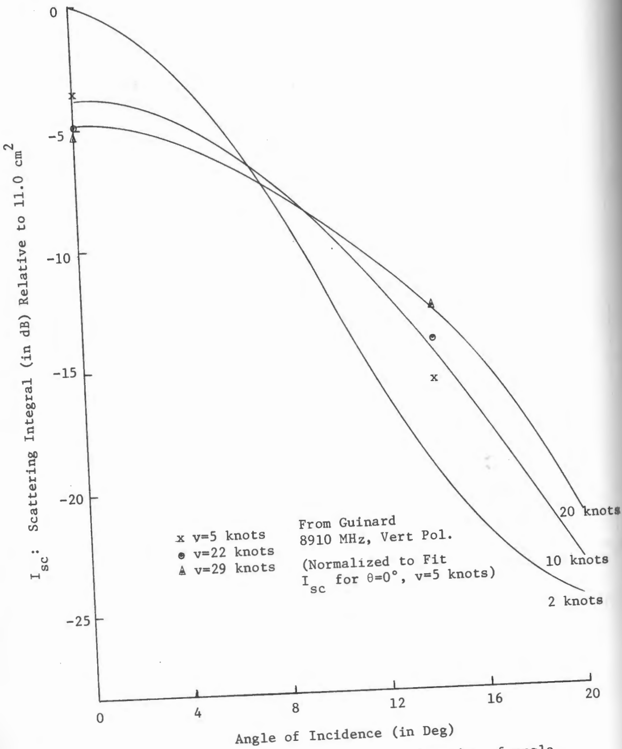
Figure 11. Scattering intergral as a function of angle ( \lambda_{rf} = 3.0 \text{ cm} )
