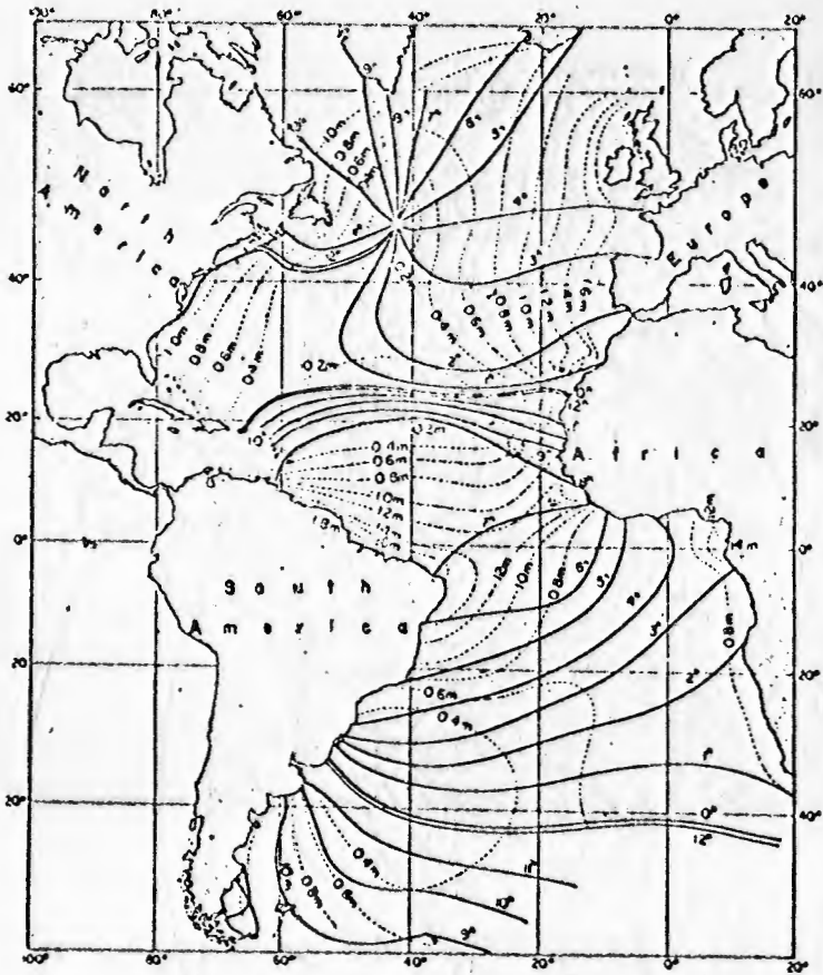
Theoretical tides of Atlantic Ocean. Full lines; co-tidal lines referred to moon-transition through meridian of Grw., dashed lines: co-range lines of the semi-diurnal tide M_2 in m (according to Hansen).
