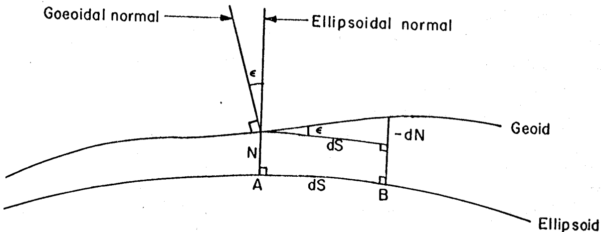
FIGURE 1. SCHEMATIC RELATION BETWEEN GEOID AND ELLIPSOID
