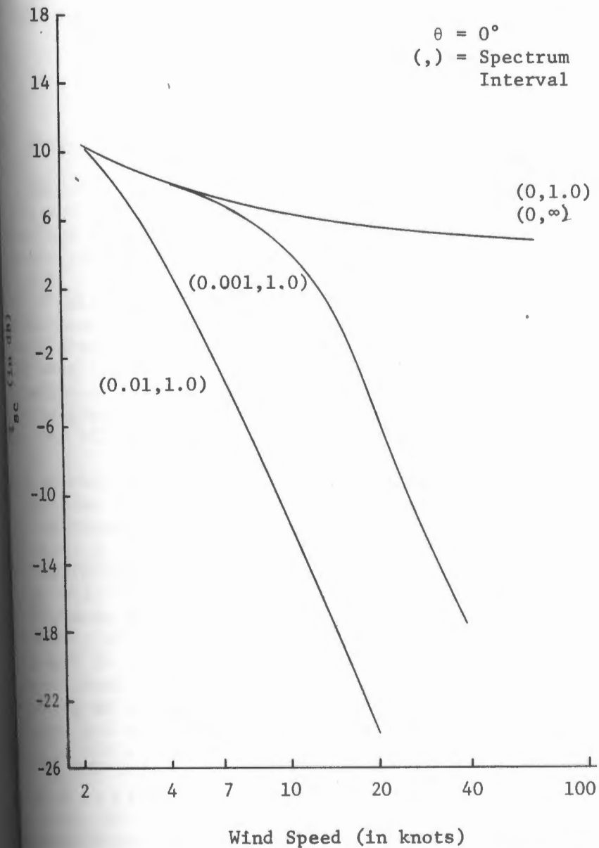
Figure 14. Behavior of scattering integral for various lower spectrum truncation points, \lambda_{rf} = 3 cm.
