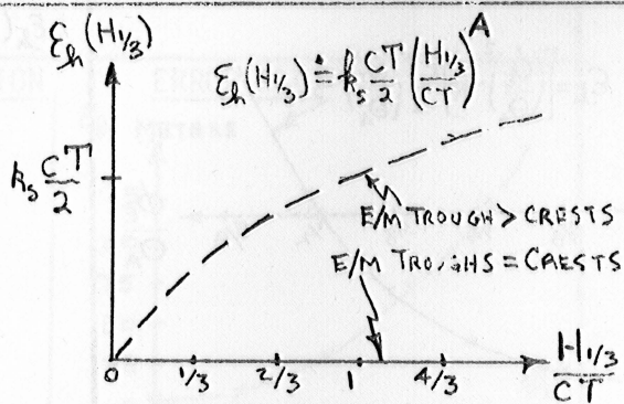
d. - SEASTATE DISPERSION
