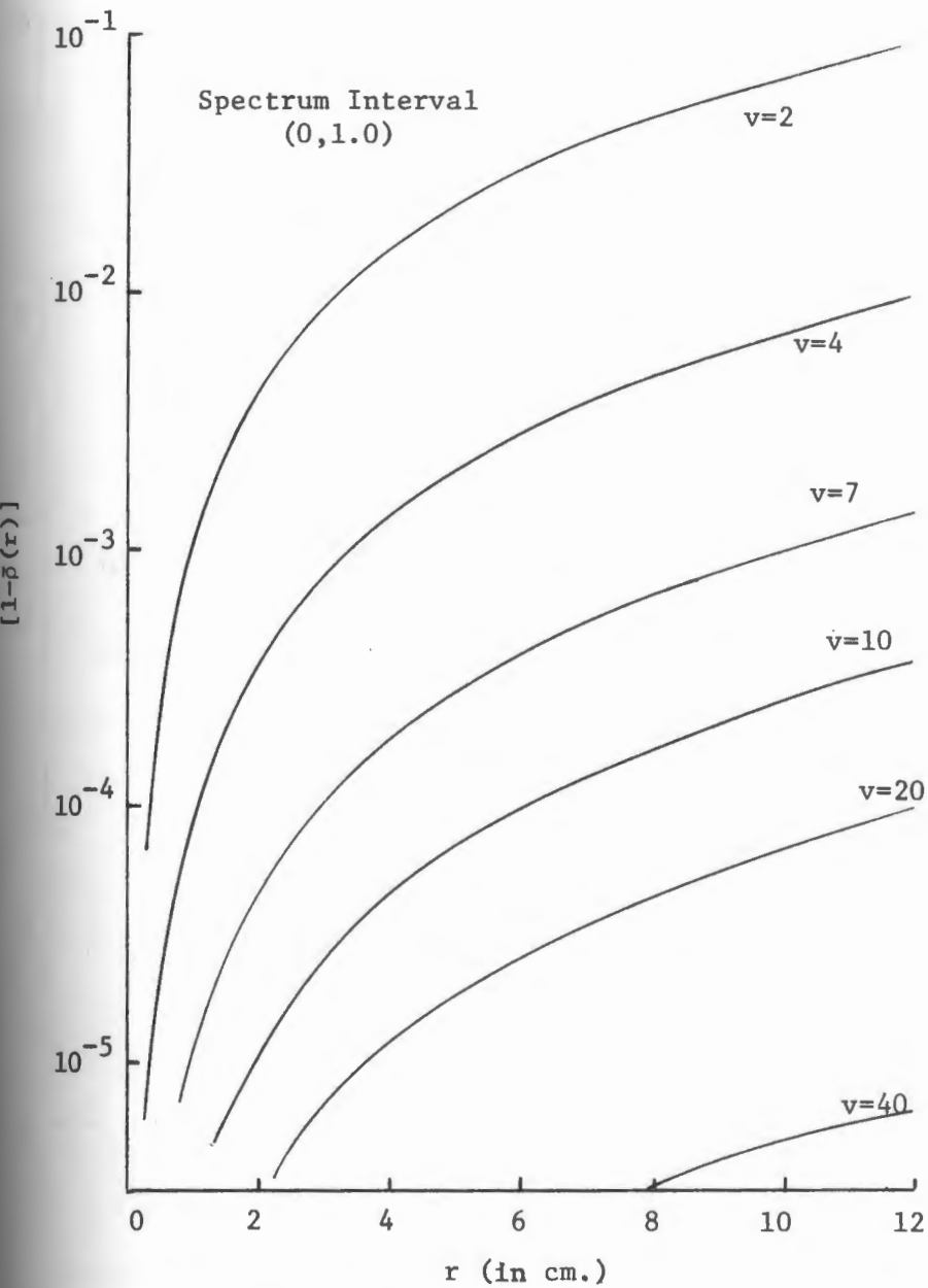
Figure 12. 1 - \bar{\rho}(r) as a function of r and v when the spectrum interval is (0, 1.0) , i.e., essentially the same as (0, \infty) .
