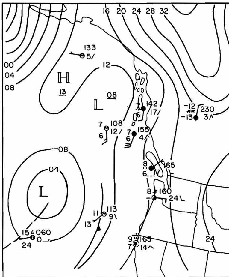
1200 GMT 1 MARCH 1980 SLP
