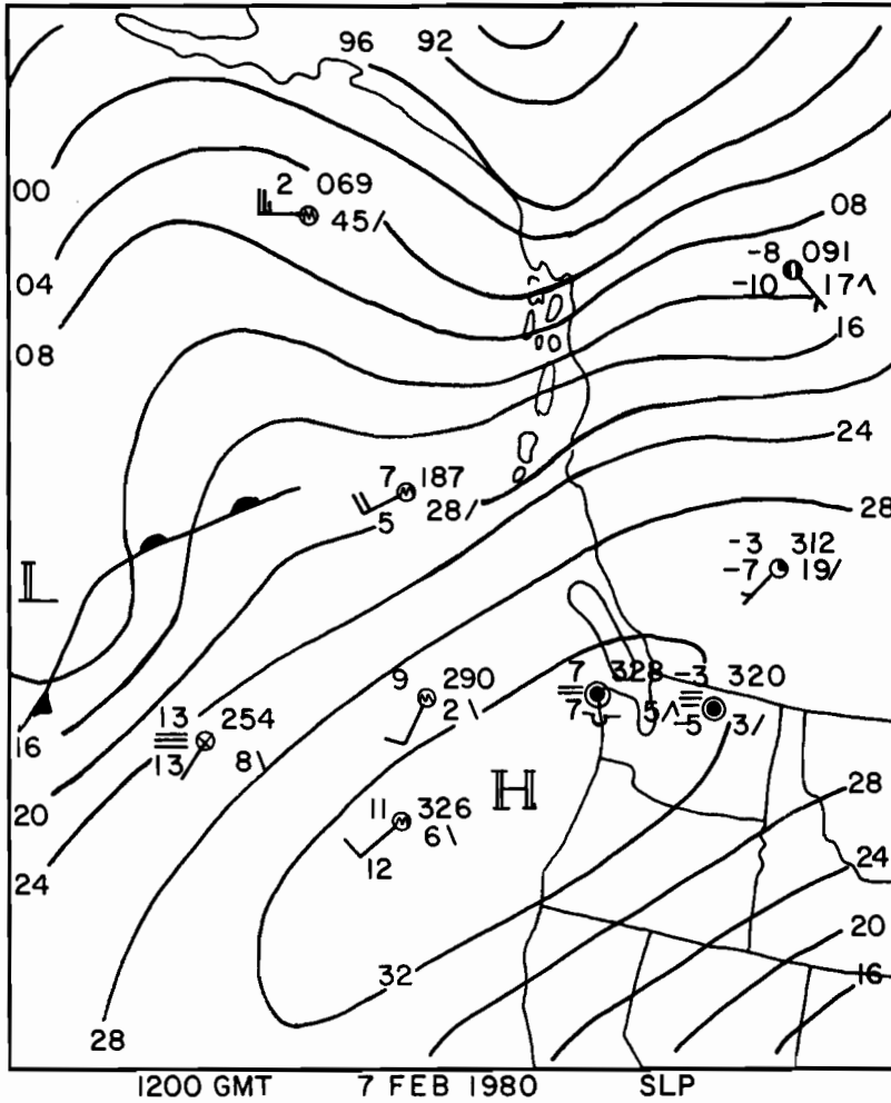
Figure 2. Sea-level pressure analysis and 850-mb geopotential height contour analysis for 1200 GMT 7 February 1980.
