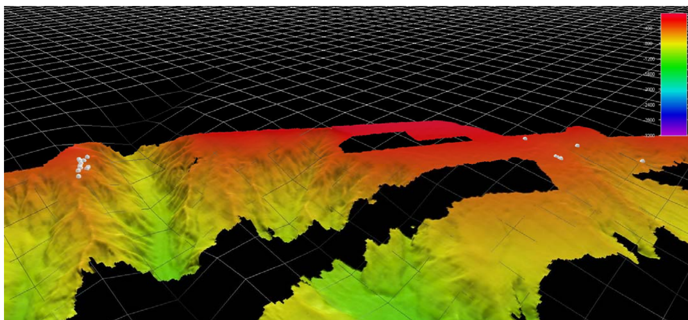
Figure 4. New seeps discovered near Washington Canyon, indicated by white spheres. Background data: Okeanos Explorer EM 302 bathymetry collected during EX-13-02 and Sandwell and Smith satellite altimetry. Color scale bar indicates Okeanos data depths in meters. Image created in Fledermaus v7.
