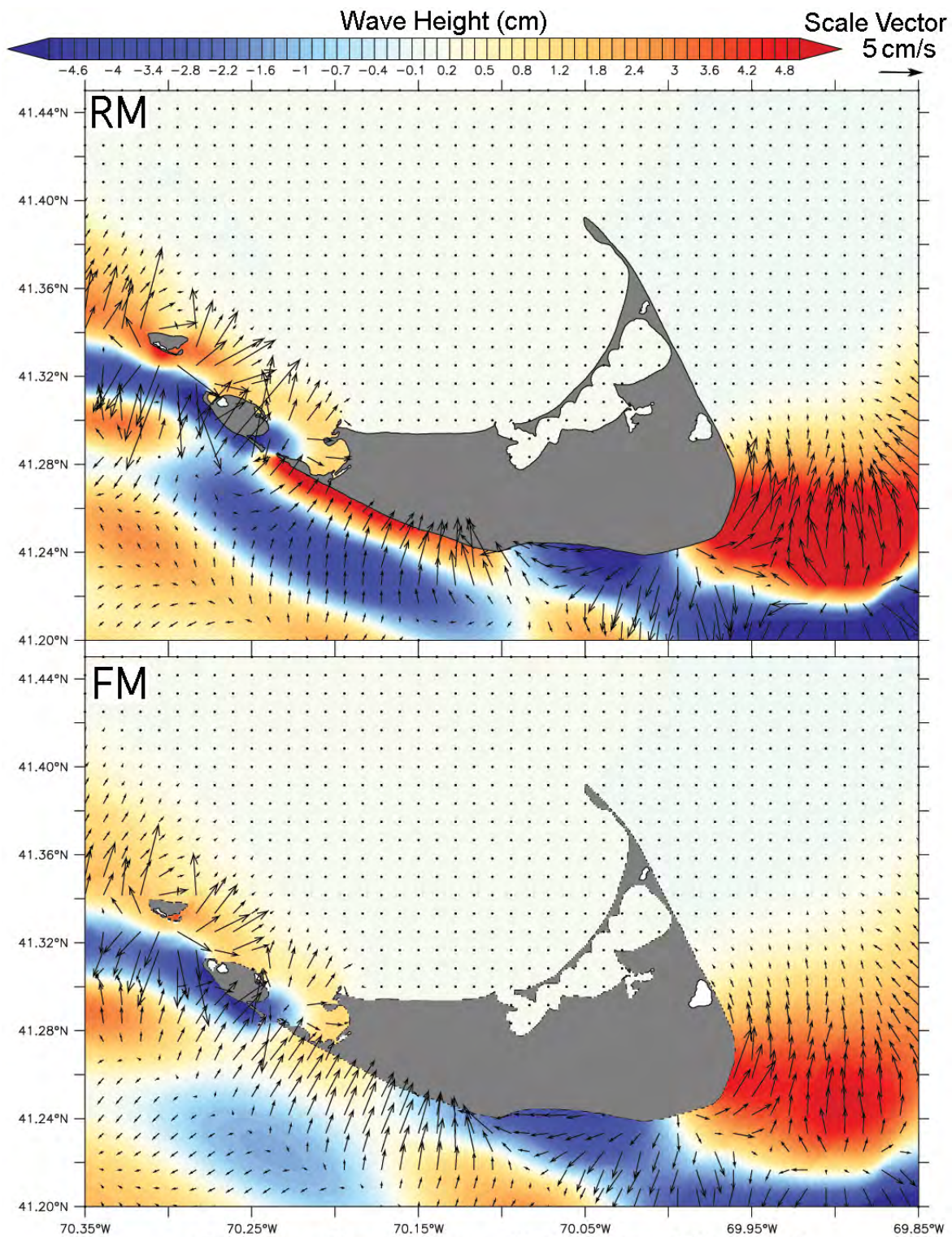
Figure 52: Comparison of the reference (RM, upper panel) and forecast (FM, lower panel) model wave height (cm) and vector current speed (cm/s) of the innermost C grid for the ATSZ B53 scenario. Time A: the leading wave crest reaches Siasconset.
