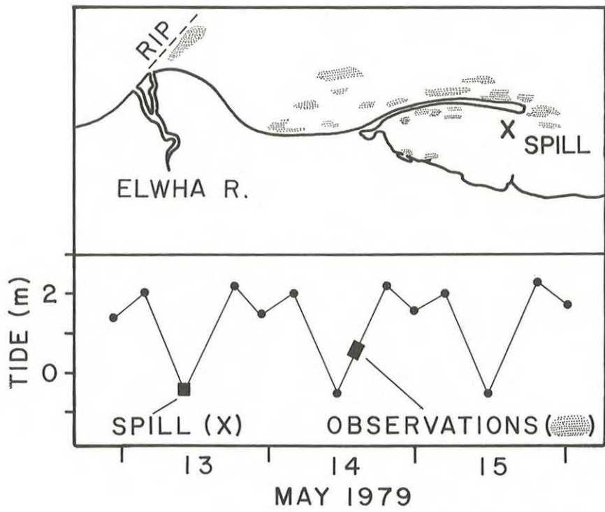
Figure 5.1. Dispersion of oil from a spill (X) on 13 May 1979 as observed (stippled) 14 May 1979. Notation: RIP, rip line associated with Elwha River discharge.
