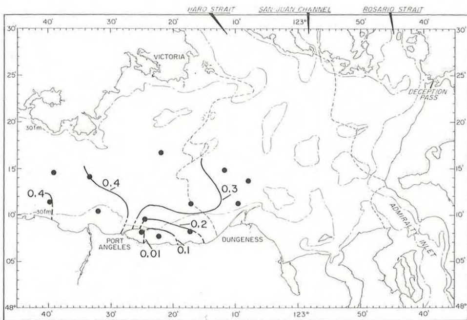
Figure 3.3. Plan view of variance near the surface (approximately 5 m depth) of longer period current meter records. Note change in contour interval between 0.1 and 0.01 m^2 s^{-2} . Notation: dashed lines, selected sills.
