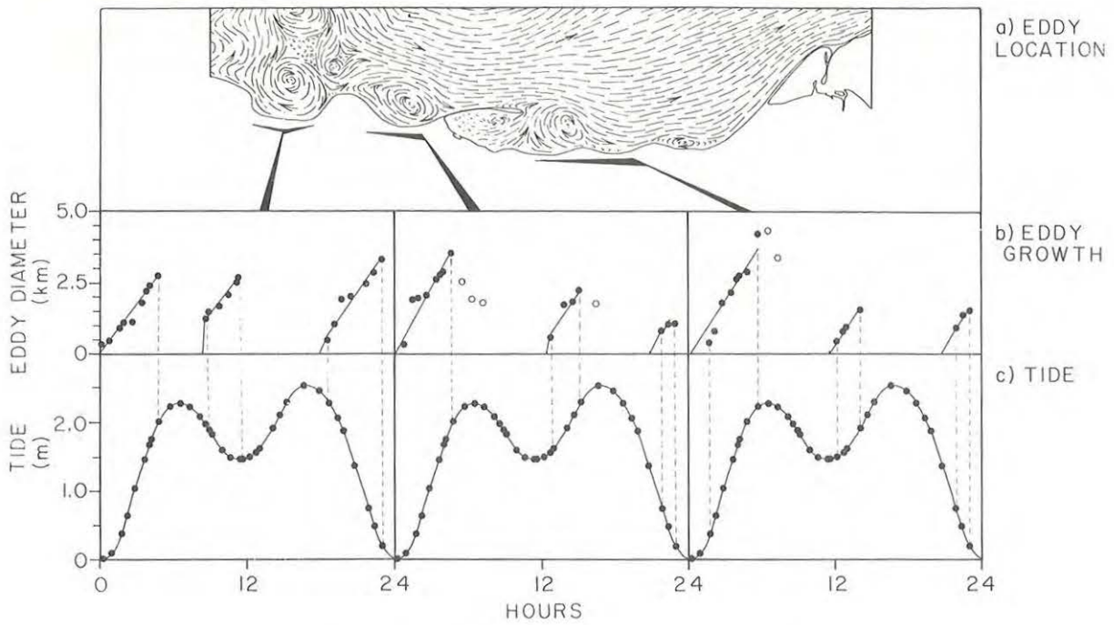
Figure 3.7. At three sites (a) growth of tidal eddies (b) in the hydraulic tidal model. Dots and circles denote respectively diameter during eddy growth and decay. In c) tidal phases are shown by dots on tide curves.
