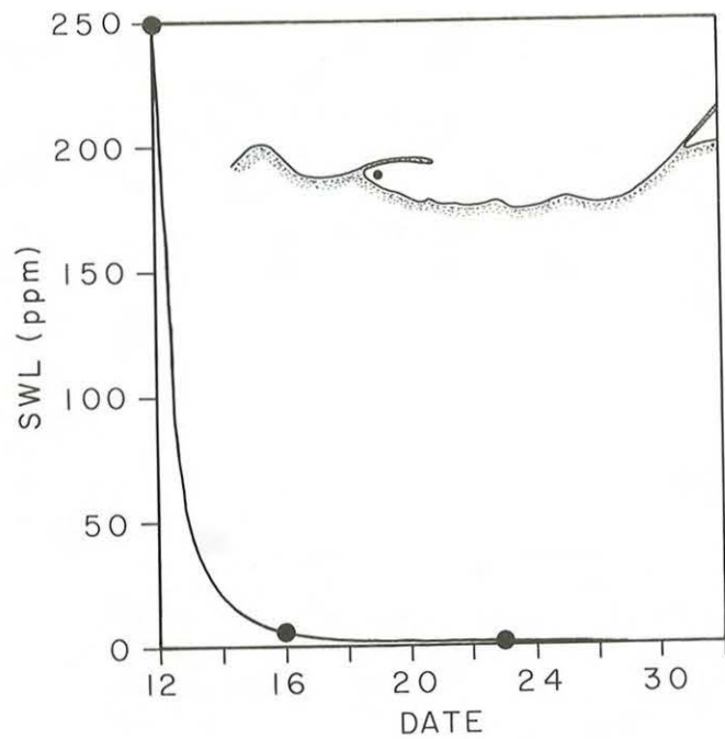
Figure 4.5. Concentration of sulfite waste liquor (dots) at the head of Port Angeles Harbor (inset) after abrupt decrease in effluent discharge on 12 November 1964 (from Ebbesmeyer et al. , 1979).
