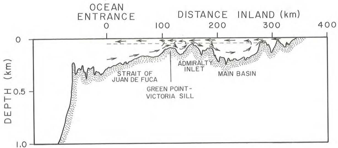
Figure 3.1. Profile view of net circulation at mid-channel in summer between the Pacific Ocean and the head of Puget Sound (adapted from Ebbesmeyer and Barnes, 1979). Notation: dashed line, depth of no-net-motion (approximately 50 m).
