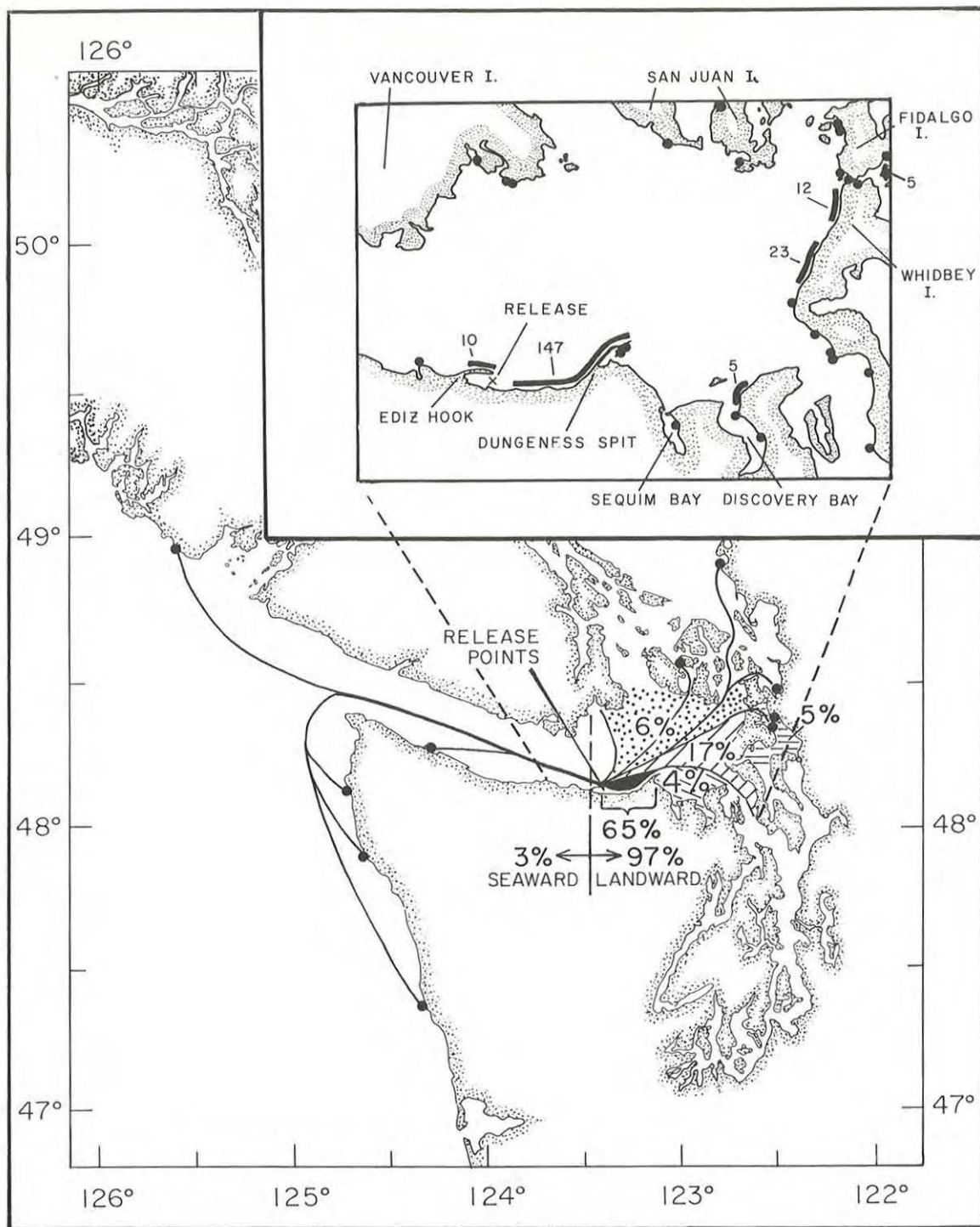
Figure 5.8. Recoveries onshore of drift cards released in Port Angeles Harbor expressed as percentage of 240 recoveries (adapted from Ebbesmeyer et al. , 1978). Notation: dots, single recoveries; stippling, hatched, and blackened areas, multiple recoveries expressed as percentages of total recoveries. Inset shows the number of recoveries in the inner Strait of Juan de Fuca.
