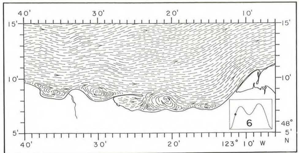
Appendix C.4-C.6. Surface tidal current patterns.
