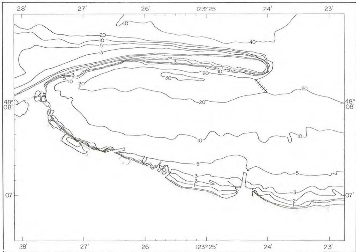
Figure 1.3. Bathymetry (fathoms) within the study area (top) and Port Angeles Harbor (bottom). Notation: hatched lines, Green Point-Victoria sill (top) and Harbor entrance sill-like feature (bottom); dashed line, lateral constriction of the Strait of Juan de Fuca. Conversion factor: 1 fathom = 1.83 m.
