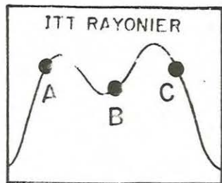
Figure 5.6. Photographs of dye injected into the hydraulic tidal model at ITT Rayonier, Inc. and Crown Zellerbach, Inc. outfall locations (adapted from Ebbesmeyer et al. , 1979). Insets at bottom show tidal phases.
