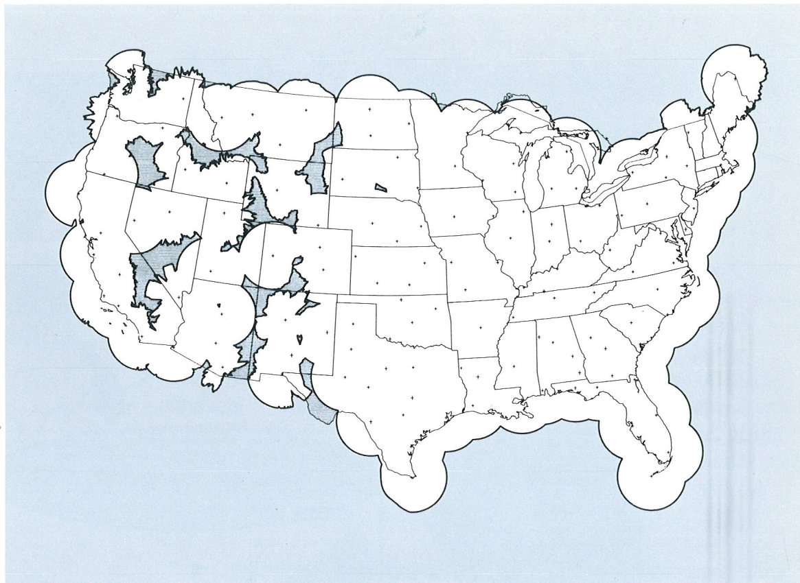
Depiction of the Total Coverage (at 10,000 Ft. Elevation) Provided by the Completed National NEXRAD Network.
