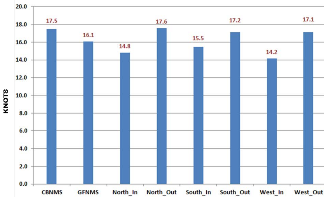
Figure 13: Cargo Vessels Mean Speed in Each Lane
