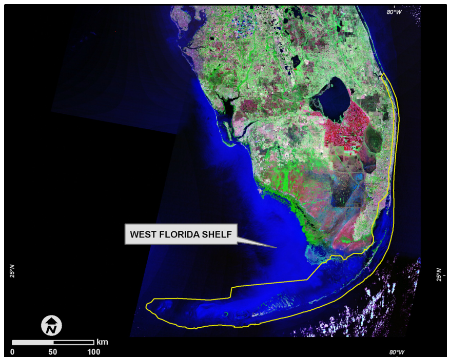
The yellow polygon delineates the approximately 13,000 sq km priority shallow-water benthic habitat mapping area of southern Florida.
