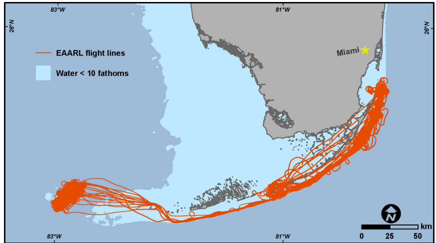
The locations where NASA EAARL (Experimental Advanced Airborne Research LIDAR) data have been collected in southern Florida.
