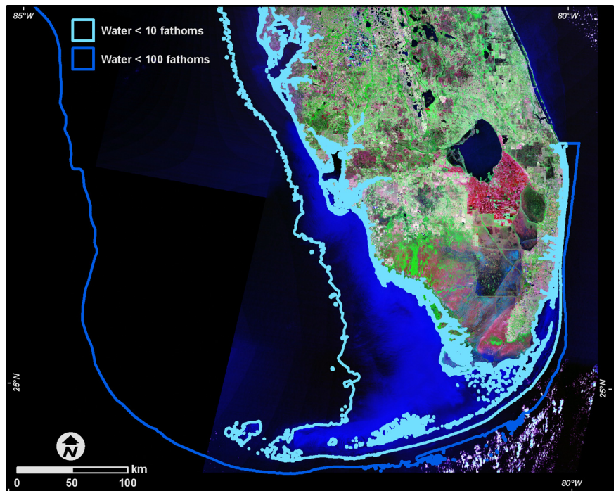
The location of the 10 fm (~18 m) and 100 fm (~183 m) depth curves in southern Florida.
