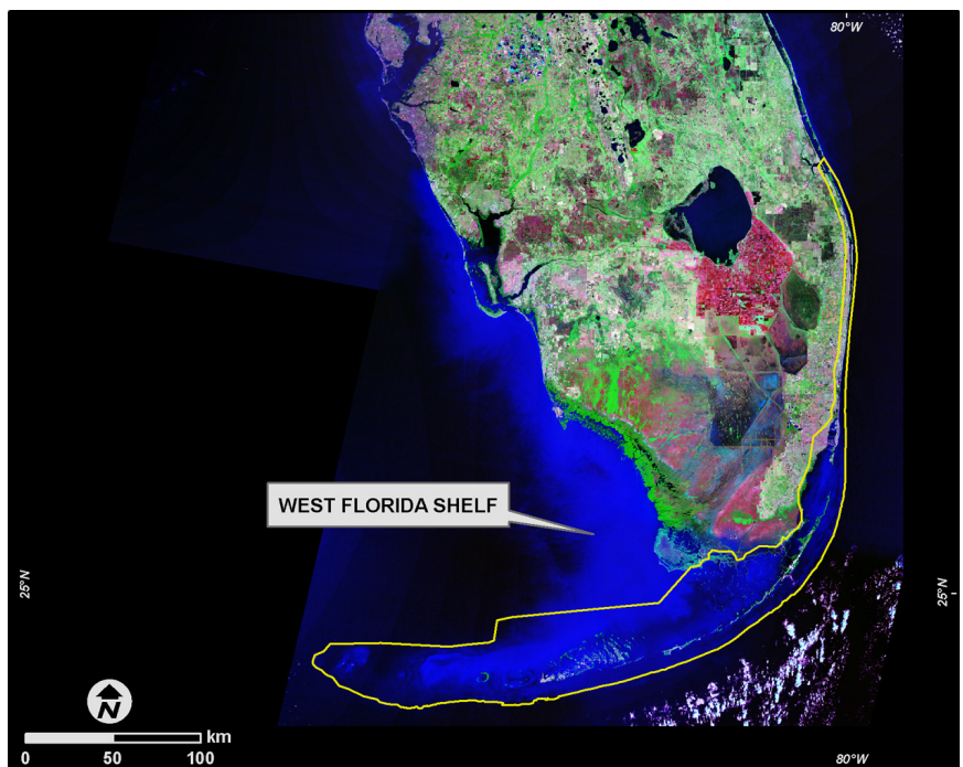
Figure 1. The yellow polygon delineates the approximately 13,000 sq km priority shallow-water benthic habitat mapping area of southern Florida.
