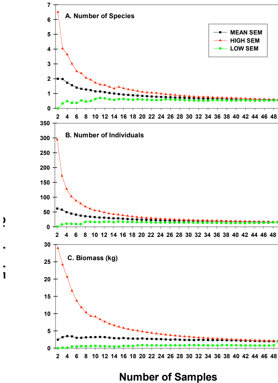
Figure B-4: Sample size optimization of data from sample size analysis project at Tektite Reef, July 1999, for number of species, number of individuals, and biomass. Relationship between standard error of the mean (SEM) and sample size. Monte Carlo simulation procedure for sample size optimization described by Bros and Cowell (1987). (Friedlander et al. 1999)
