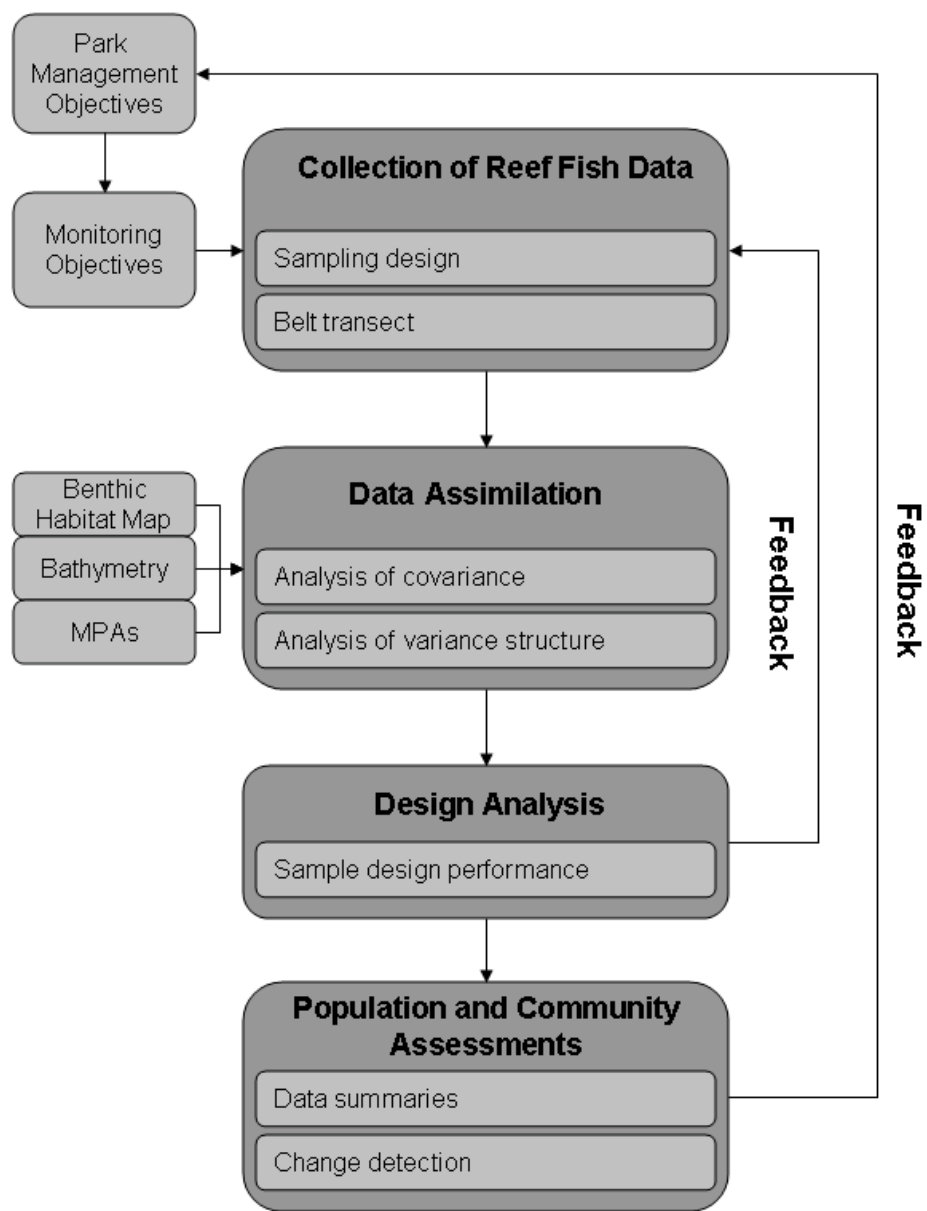
Figure A-2: A conceptual model of the Biogeography Team Coral Reef Ecosystem Monitoring Program (CREMP). Note the feedback loops.
