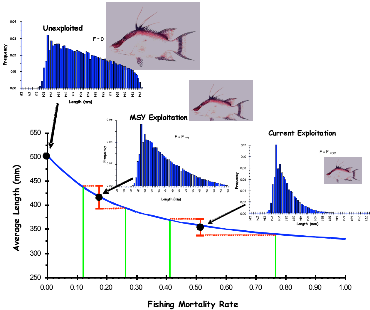
Figure C-3: Relationship of \bar{L} in the exploited phase and fishing mortality F for hogfish, and the variation in F estimates (dotted horizontal bars) resulting from variation in \bar{L} (dashed vertical bars). Insets show representative population length frequency compositions at F_0 , F_{msy} , and F_{2001} .
