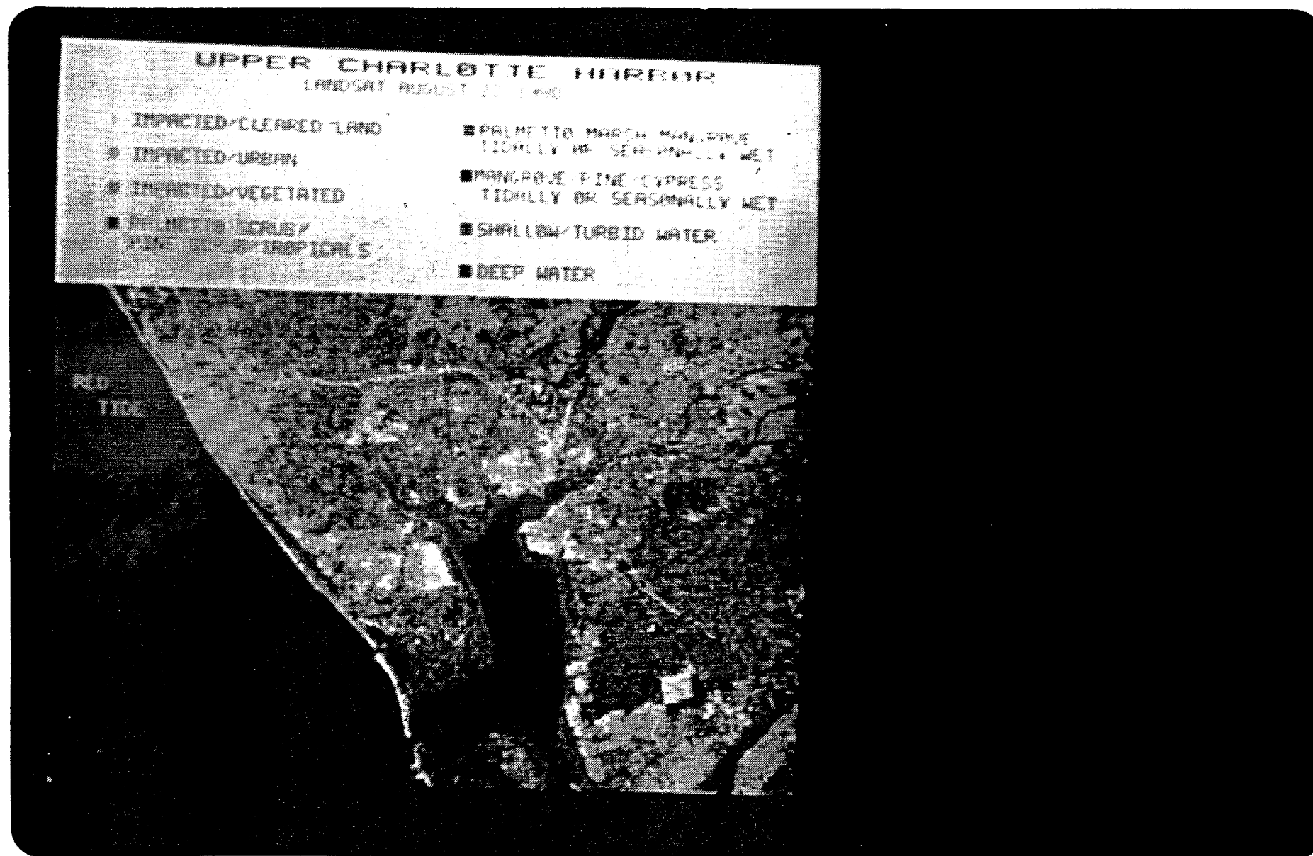
Figure 30. General LANDSAT classification of Upper Charlotte Harbor.
