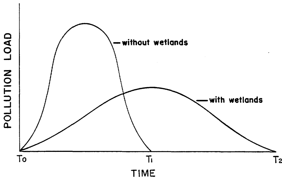
Figure 4. Rate of pollution loading to the receiving water body (after Park and Batie 1979).
