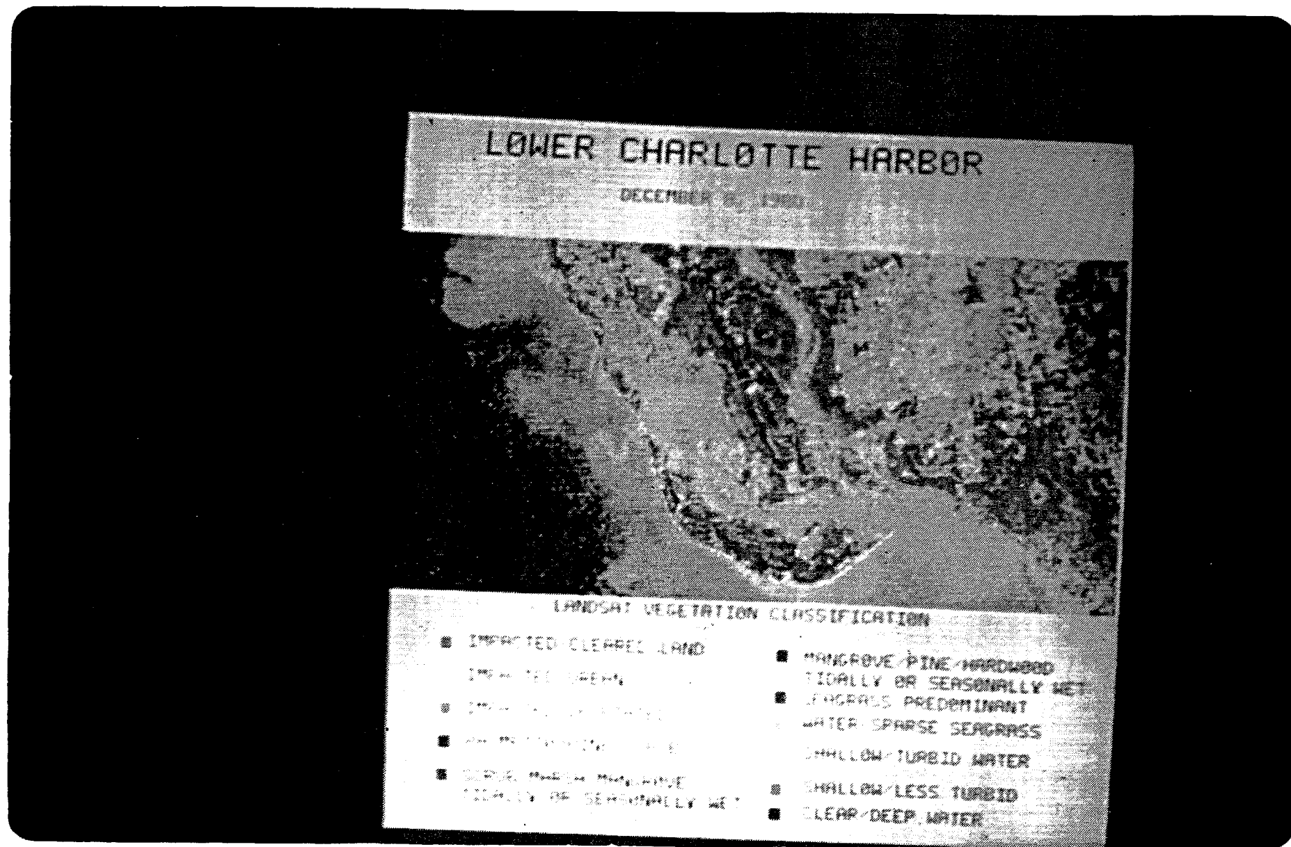
Figure 31. General LANDSAT classification of Lower Charlotte Harbor.
