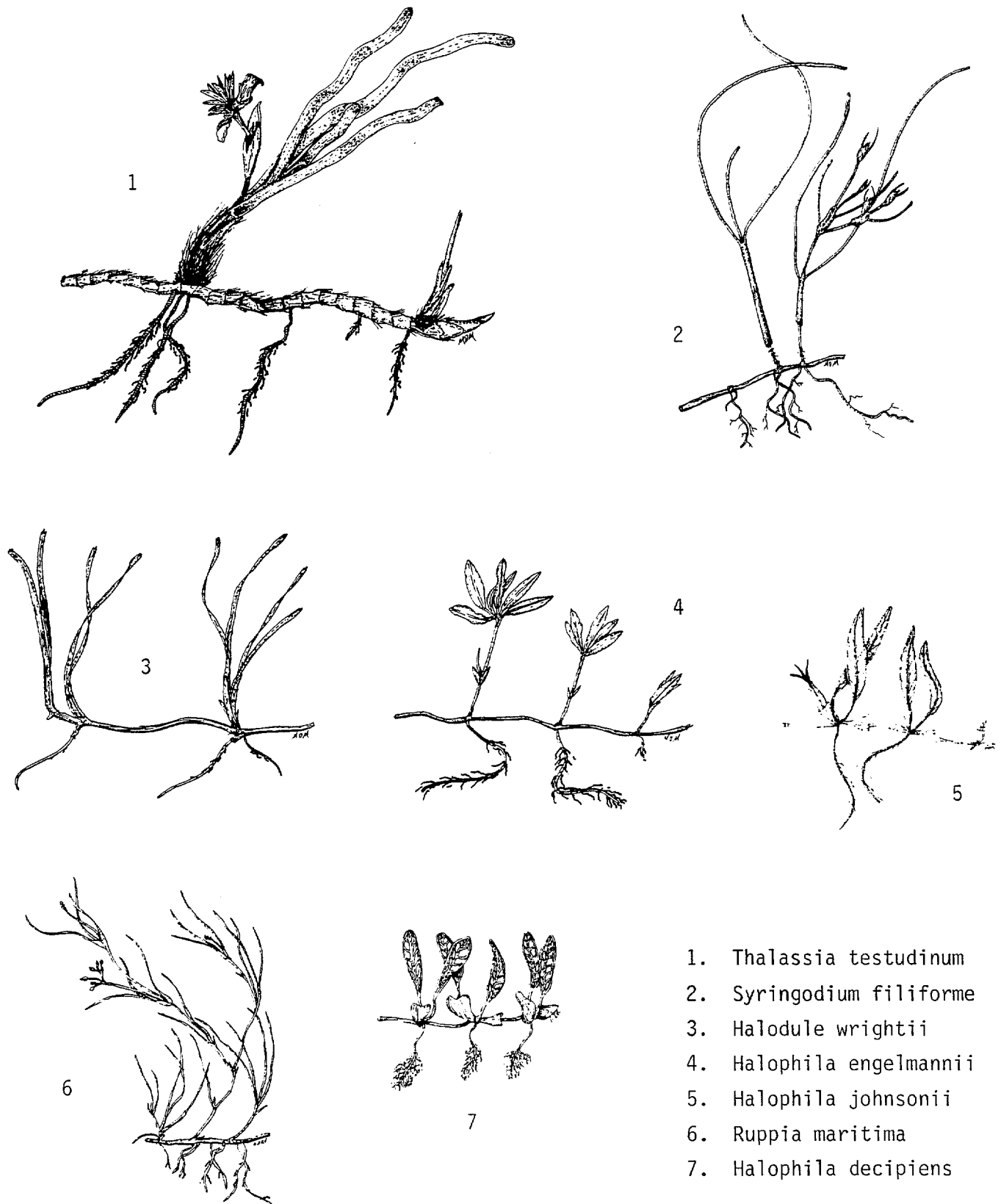
Figure 3. Seagrasses of Florida.
