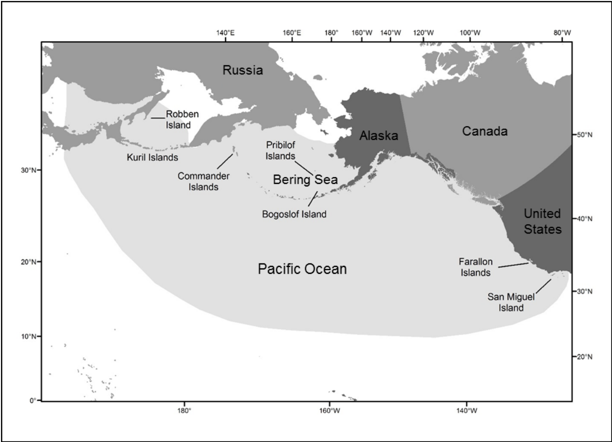
Figure 1. -- Range of northern fur seals and locations of their breeding colonies.
