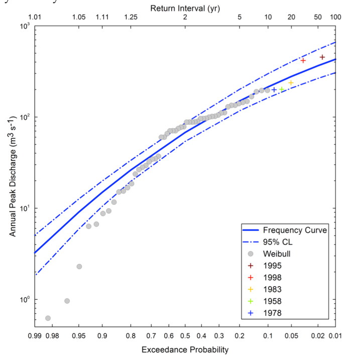
Figure 7. Carmel River flood frequency curve at the Robles Del Rio stream gage (USGS 11143200) derived from annual peak flow data for the 1956-2014 water years (three low outliers omitted from Log Pearson Type-III analysis).
