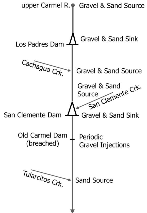
Figure 13. Schematic of gravel sources and sinks in Carmel River in vicinity of San Clemente Dam prior to the re-route.
