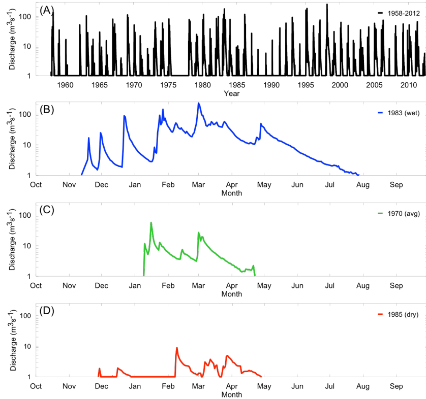
Figure 6. Mean daily discharge on the Carmel River at the Robles Del Rio stream gage (USGS 11143200). Flow data is shown for: (A) period of record (1958-2012), as well as for individual (B) wet, (C) average and (D) dry water years.
