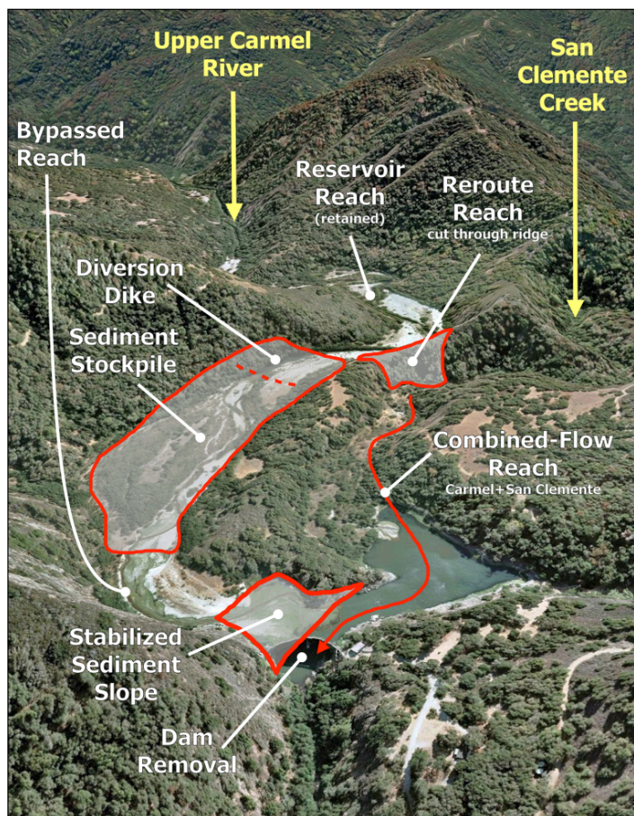
Figure 2. Main components of Carmel River Reroute and Dam Removal project (CRRDR), superimposed on the pre-removal channel configuration. ( http://www.sanclementedamremoval.org ). Not pictured is removal of the Old Carmel River Dam downstream of the main site. Image from AMBAG Oct 2007 and Google Earth.
