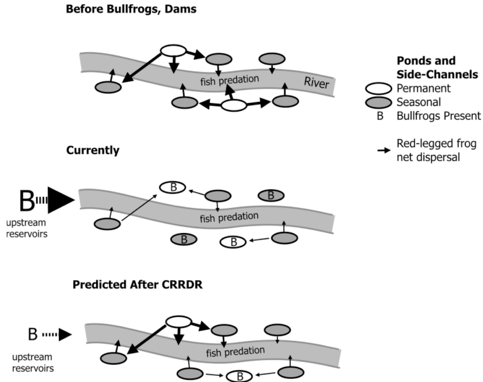
Figure 10. Conceptual model for source-sink dynamics in breeding/tadpole habitat of California red-legged frog ( R. draytonii ), along the middle and lower Carmel River.
