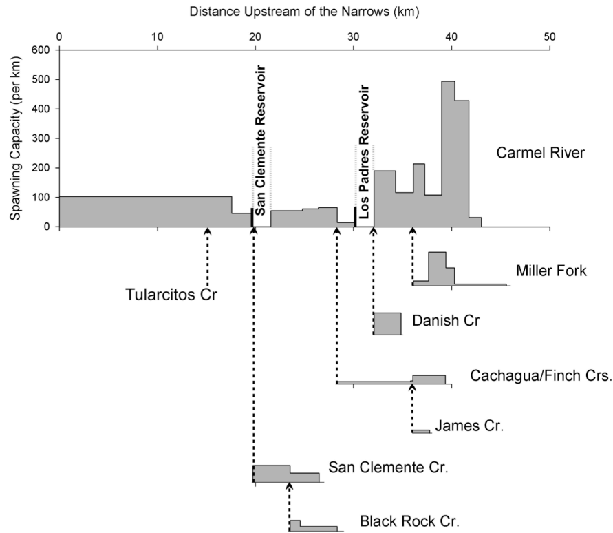
Figure 12. Distribution of spawning habitat in Carmel River and selected tributaries, from 1989 surveys by MPWMD (Daly et al. 1994). Spawning capacity estimated from area of stream channel with suitable gravel size.
