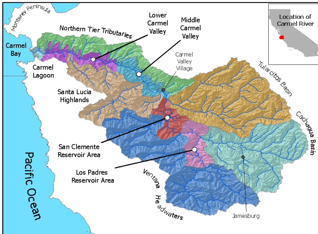
Figure 1. Carmel River system, its major landscape domains and tributaries
