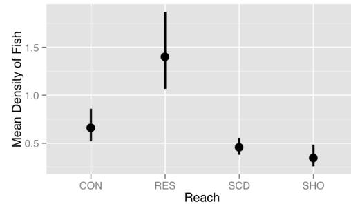
Figure 14. Estimated density ( \text{m}^{-2} ) of juvenile O. mykiss from first sampling occasion at Priority 1 sites (bars = 50% CI). CON=Control site in section C; RES=Reservoir site in section I0; SCD=I site directly below San Clemente Dam site; SHO=I site near Sleepy Hollow. Estimates are from mark-recapture.
