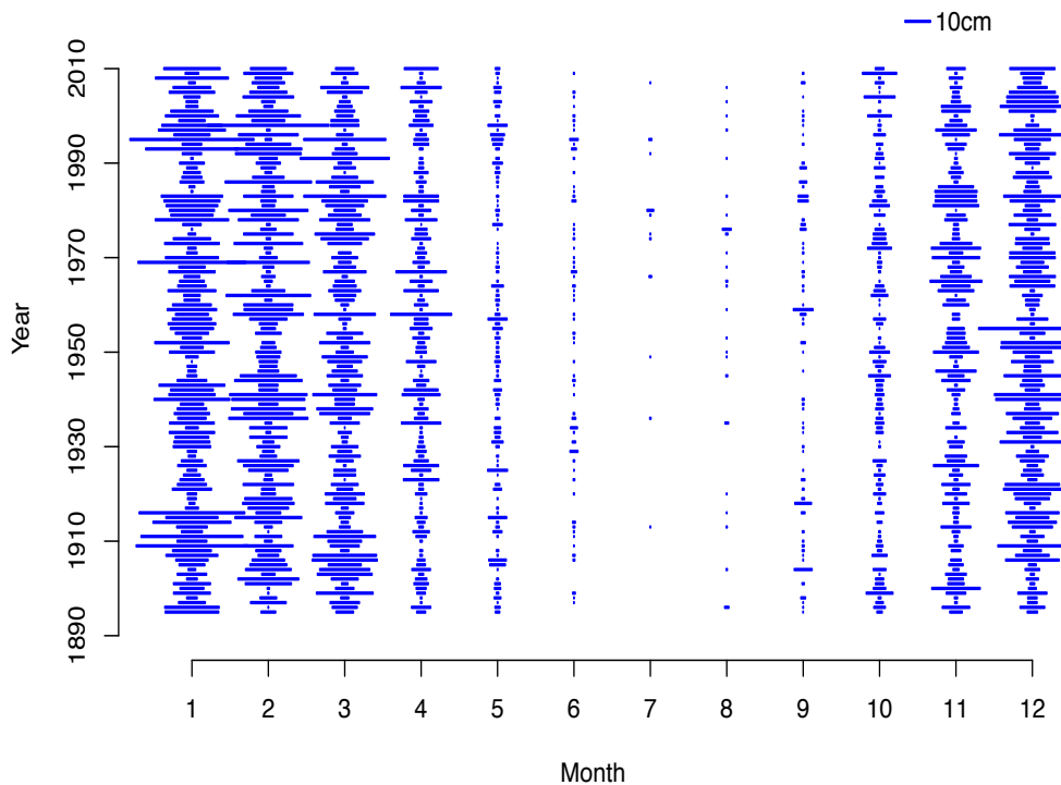
Figure 4. 116 years of seasonal and annual variation in monthly rainfall within the catchment of the Carmel River, from the PRISM dataset (Daly et al. 1994).
