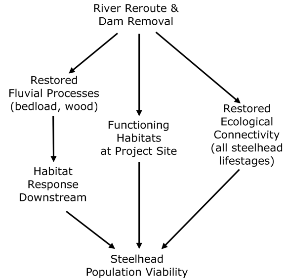
Figure 3. Conceptual model of the predicted ecological effects of the CRRDR project on steelhead population viability
