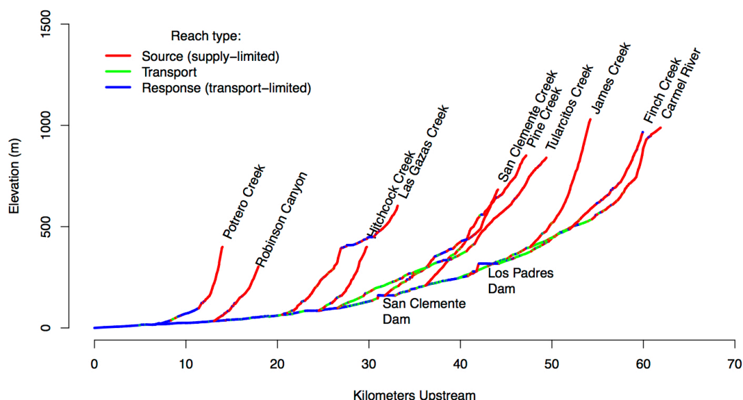
Figure 8. Longitudinal profiles of the Carmel River and principal tributaries, classified as source, transport, and response reaches according to sediment-transport scheme of Montgomery and Buffington (e.g. data summary in ENV5 660 [CSUMB Class] et al. 2012) and classifier algorithm of Flores et al. (2006).
