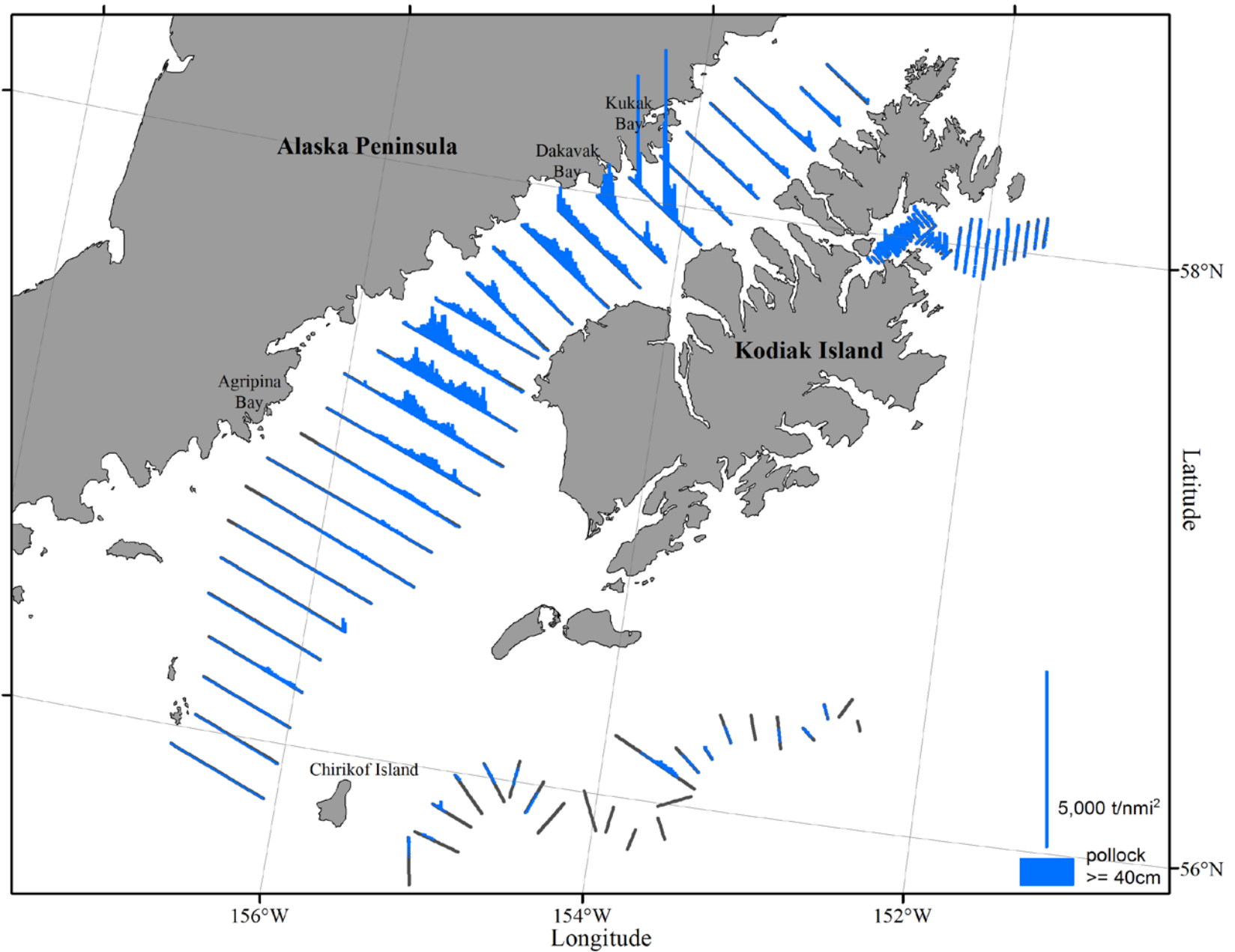
Figure 24a. -- Biomass ( t/nmi^2 ) attributed to walleye pollock \geq 40 cm FL (vertical lines) along tracklines surveyed during the winter 2015 acoustic-trawl survey of Shelikof Strait, Chirikof shelf break, and Marmot Bay.
