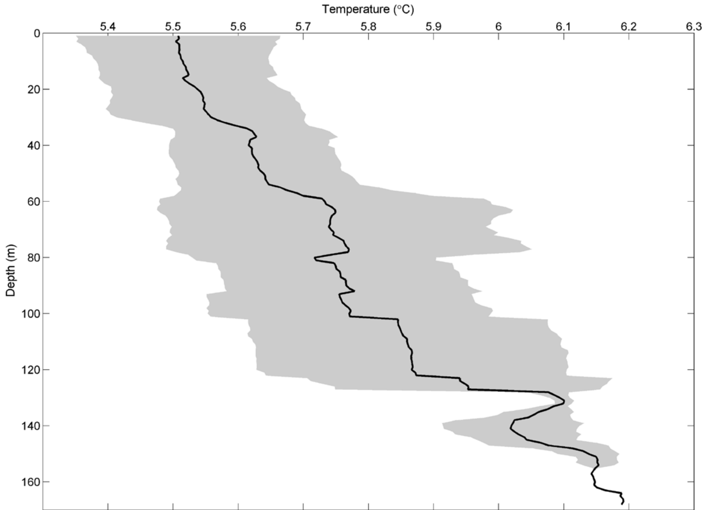
Figure 3. -- Mean water temperature (°C; solid line) by 1-m depth intervals for the eight trawl haul locations for which temperature data were collected during the winter 2015 acoustic-trawl survey of walleye pollock in the Shumagin trough, W. Nagai Strait, Unga Strait, and Stepovak Bay. Shaded area represents one standard deviation.
