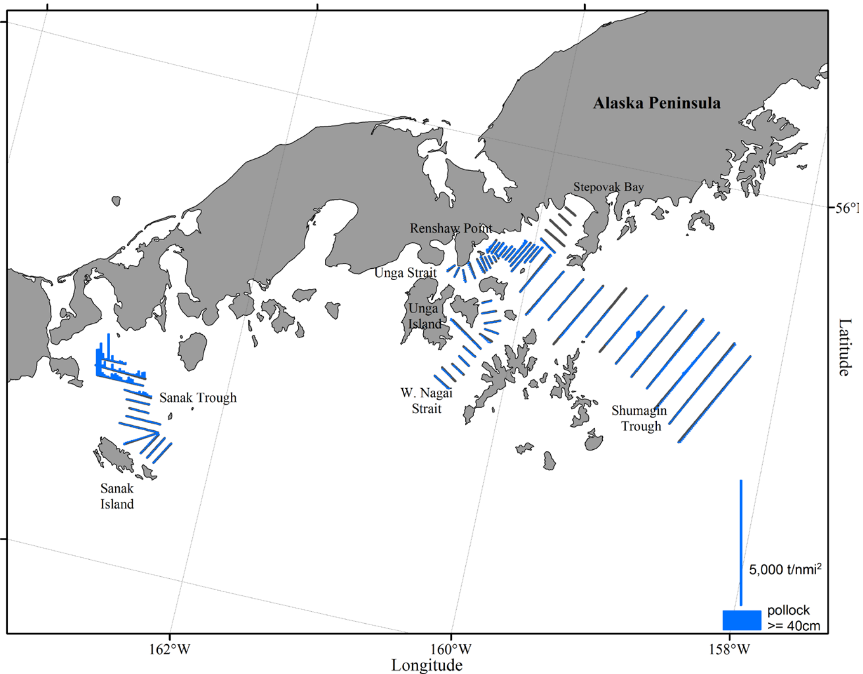
Figure 7a. -- Biomass ( t/nmi^2 ) attributed to walleye pollock \geq 40 cm FL (vertical lines) along tracklines surveyed during the winter 2015 acoustic-trawl survey of the Shumagin Islands and Sanak Trough.
