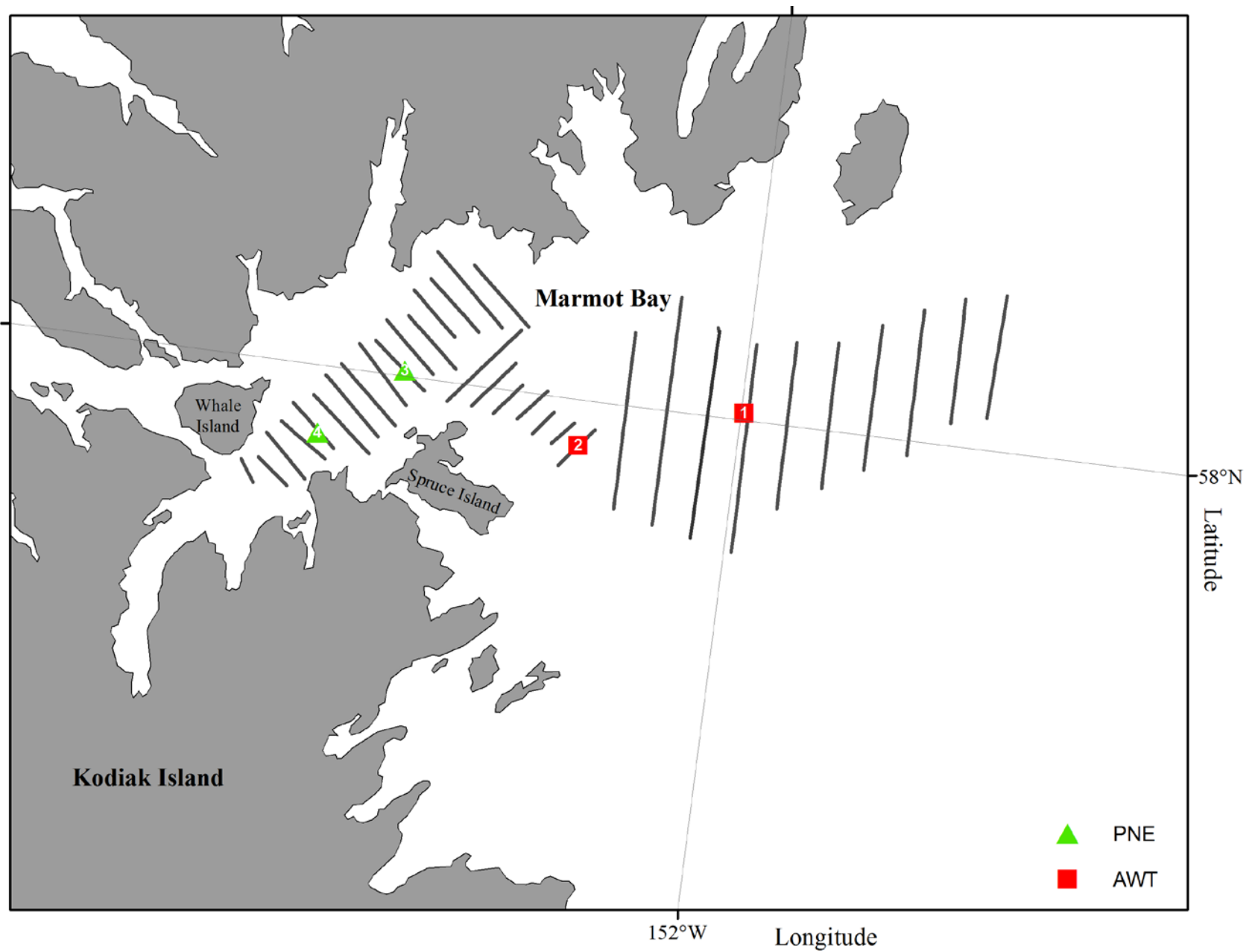
Figure 31. -- Transect lines and locations of Aleutian-wing trawl (AWT) and poly-Nor'eastern trawl (PNE) hauls during the winter 2015 acoustic-trawl survey of walleye pollock in Marmot Bay and Izhut Bay. Figure represents area enlarged from Figure 17.
