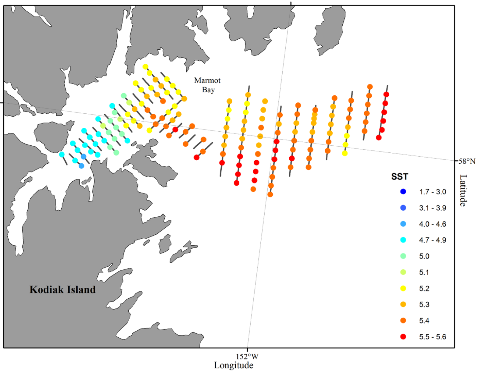
Figure 32. -- Surface water temperatures ( ^{\circ}\text{C} ) during the 2015 acoustic-trawl survey of Marmot Bay and Shelikof Strait recorded from the ship's Furuno T-2000 temperature probe located 1.4 m below the surface.
