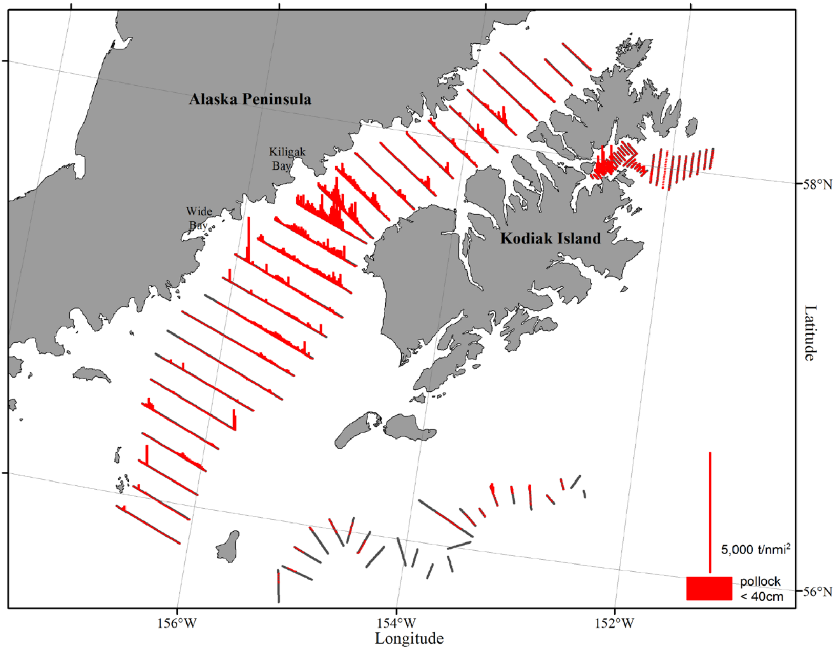
Figure 24b. -- Biomass (t/nmi 2 ) attributed to walleye pollock < 40 cm FL (vertical lines) along tracklines surveyed during the winter 2015 acoustic-trawl survey of Shelikof Strait, Chirikof shelf break, and Marmot Bay.
