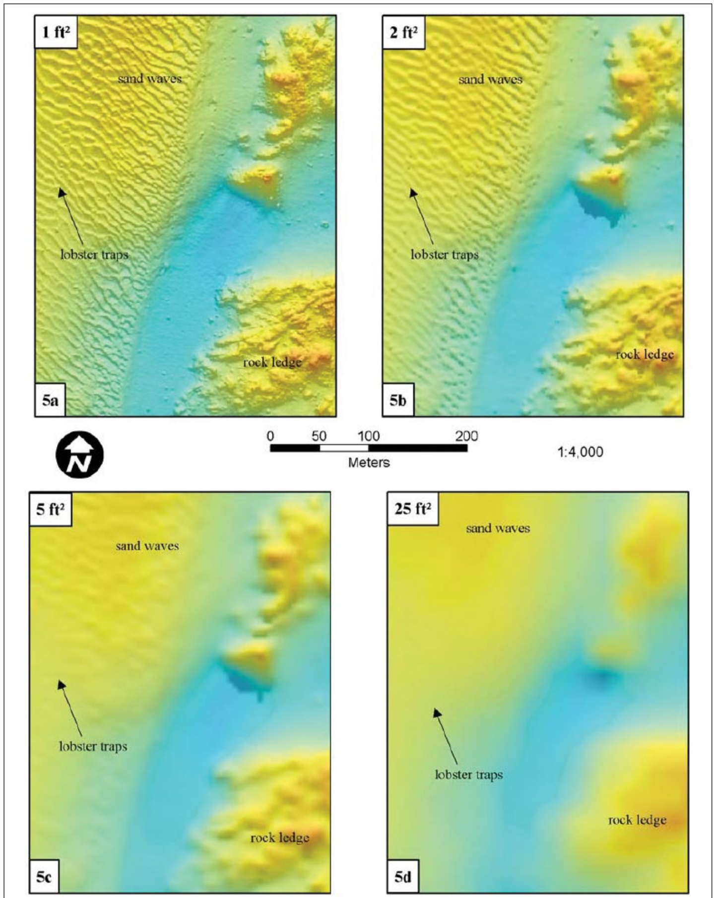
Figure 5. Multibeam data showing effect of data resolution on visualizing seafloor habitat at different spatial scales (Andrews, 2003).
