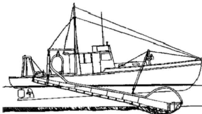
FIGURE 3. ESCALATOR DREDGE (Kyte and Chew 1975)
