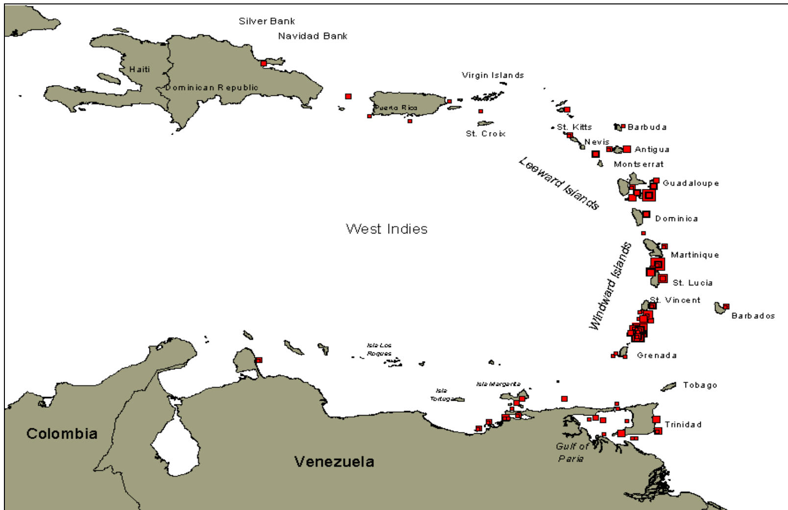
Figure 1. Location of historical catches of humpback whales based on American whaling logbooks (square symbols).
