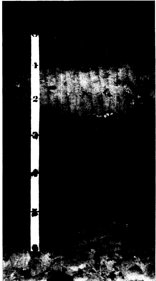
Figure 6.—Typical profile of Coosaw loamy fine sand. Note highly leached area from a depth of 1 foot to 2.5 feet and well-developed subsoil from 2.5 to 4 feet. Clay content decreases with depth to about 6 feet where the soil is underlain by stratified sand and clay.
