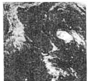
1231 GMT 10/9/80 970 MB
