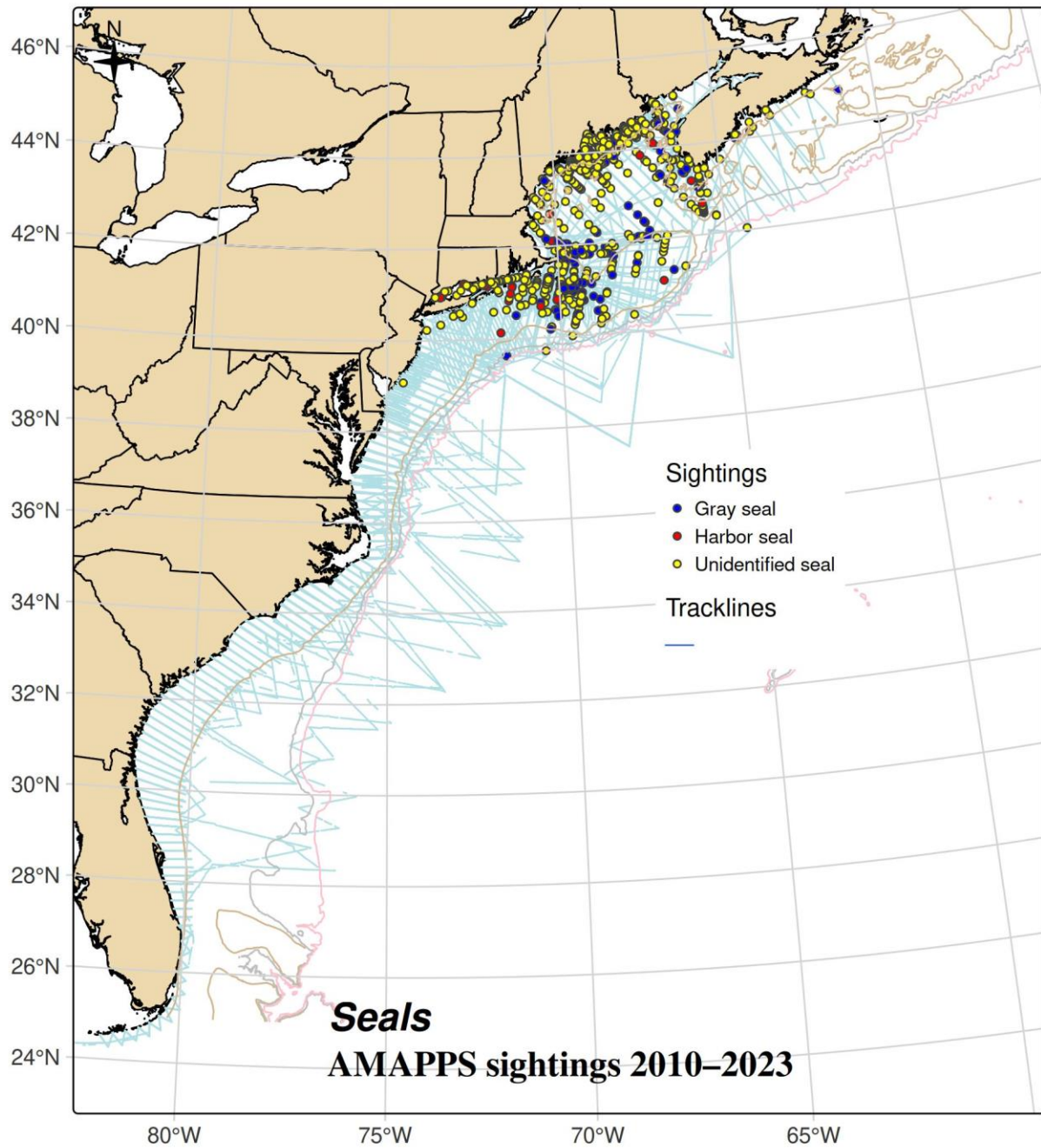
Figure E.3-1 Distribution of track lines and sightings of seals 2010 to 2023
