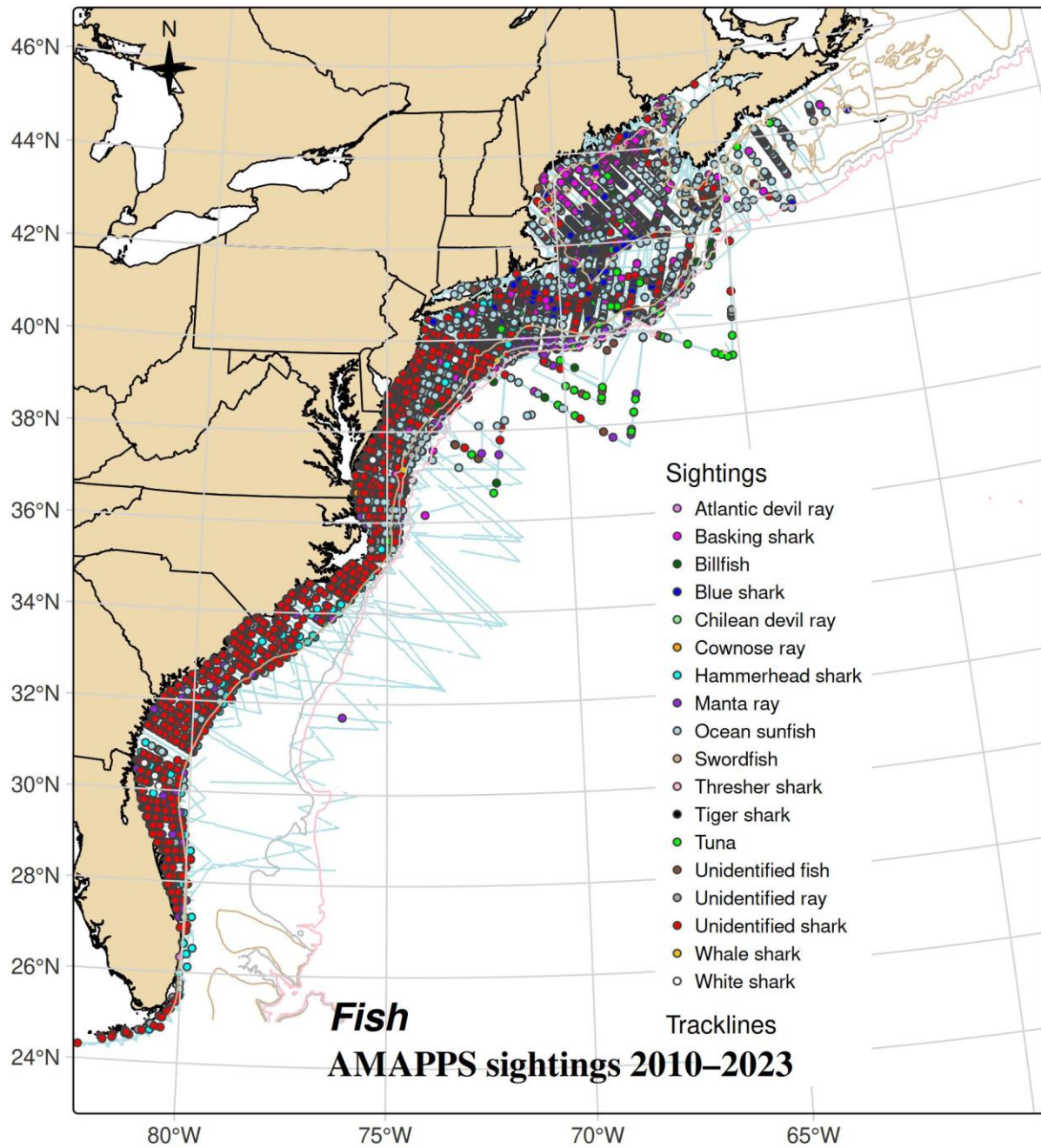
Figure E.6-1 Distribution of track lines and sightings of fish 2010 to 2023
