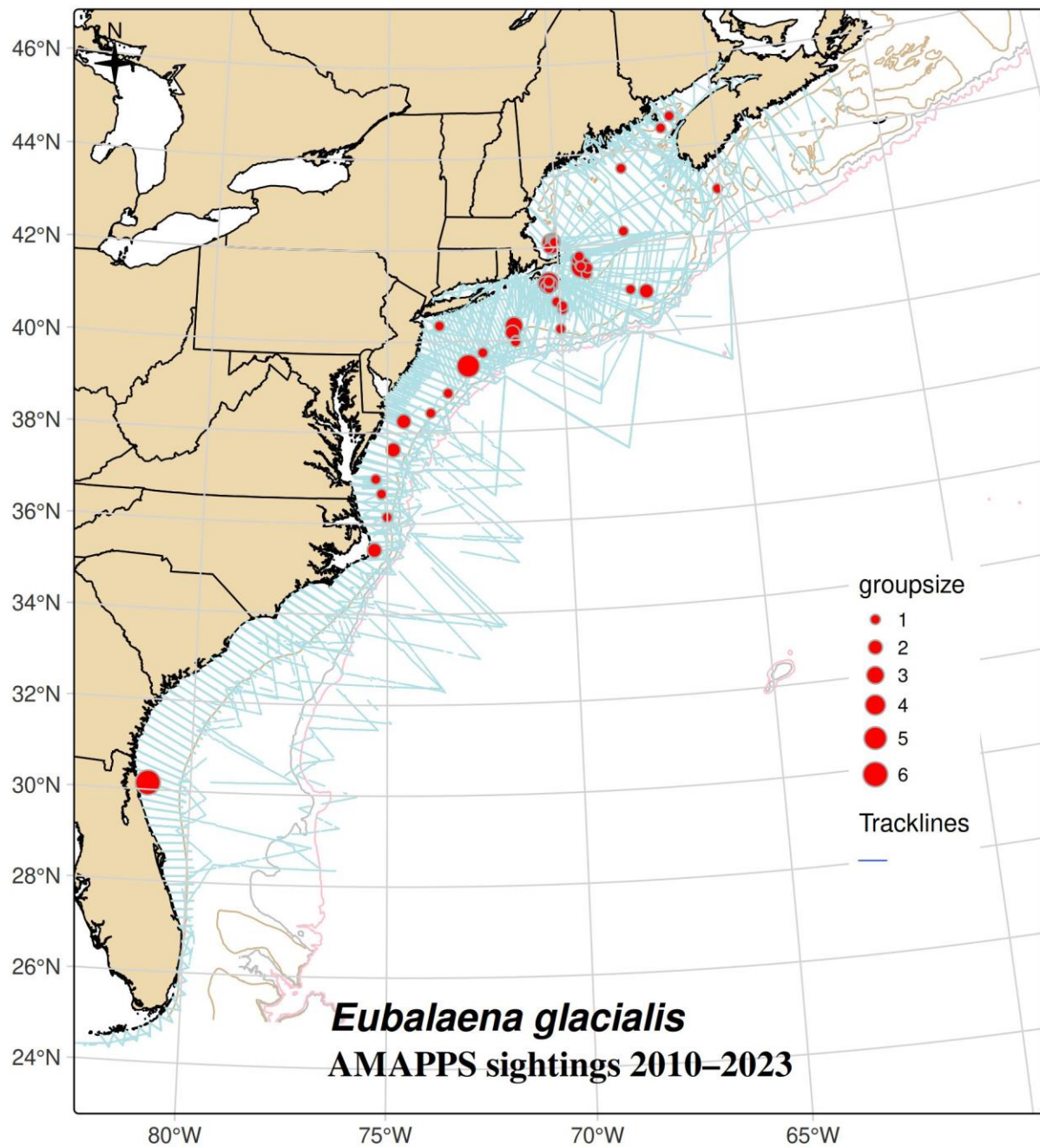
Figure E.1-1 Distribution of track lines and sightings of North Atlantic right whales 2010 to 2023
