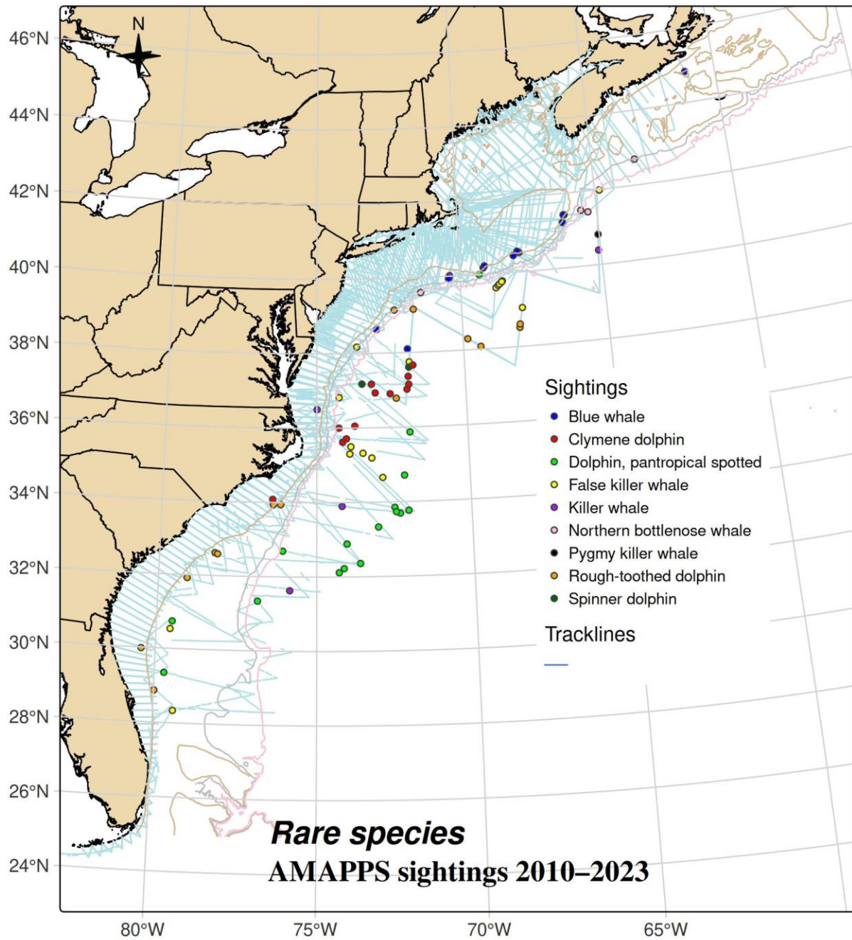
Figure E.2-1 Distribution of track lines and sightings of rarely detected cetaceans 2010 to 2023
