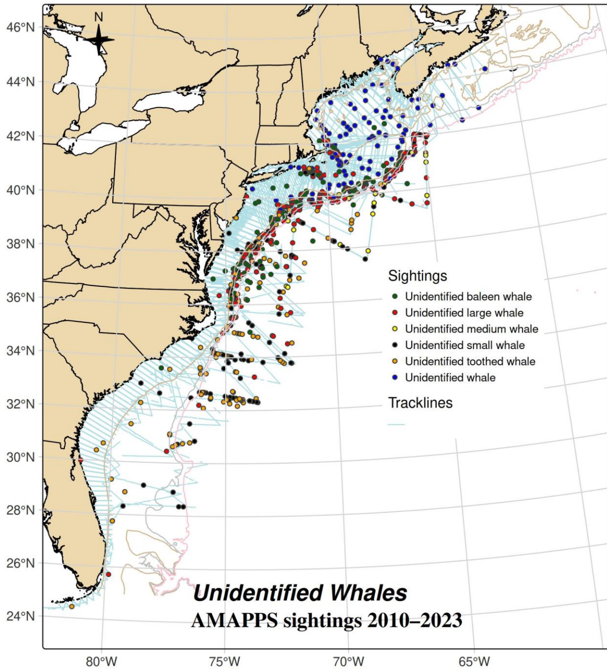
Figure E.5-1 Distribution of track lines and sightings of unidentified whales 2010 to 2023
