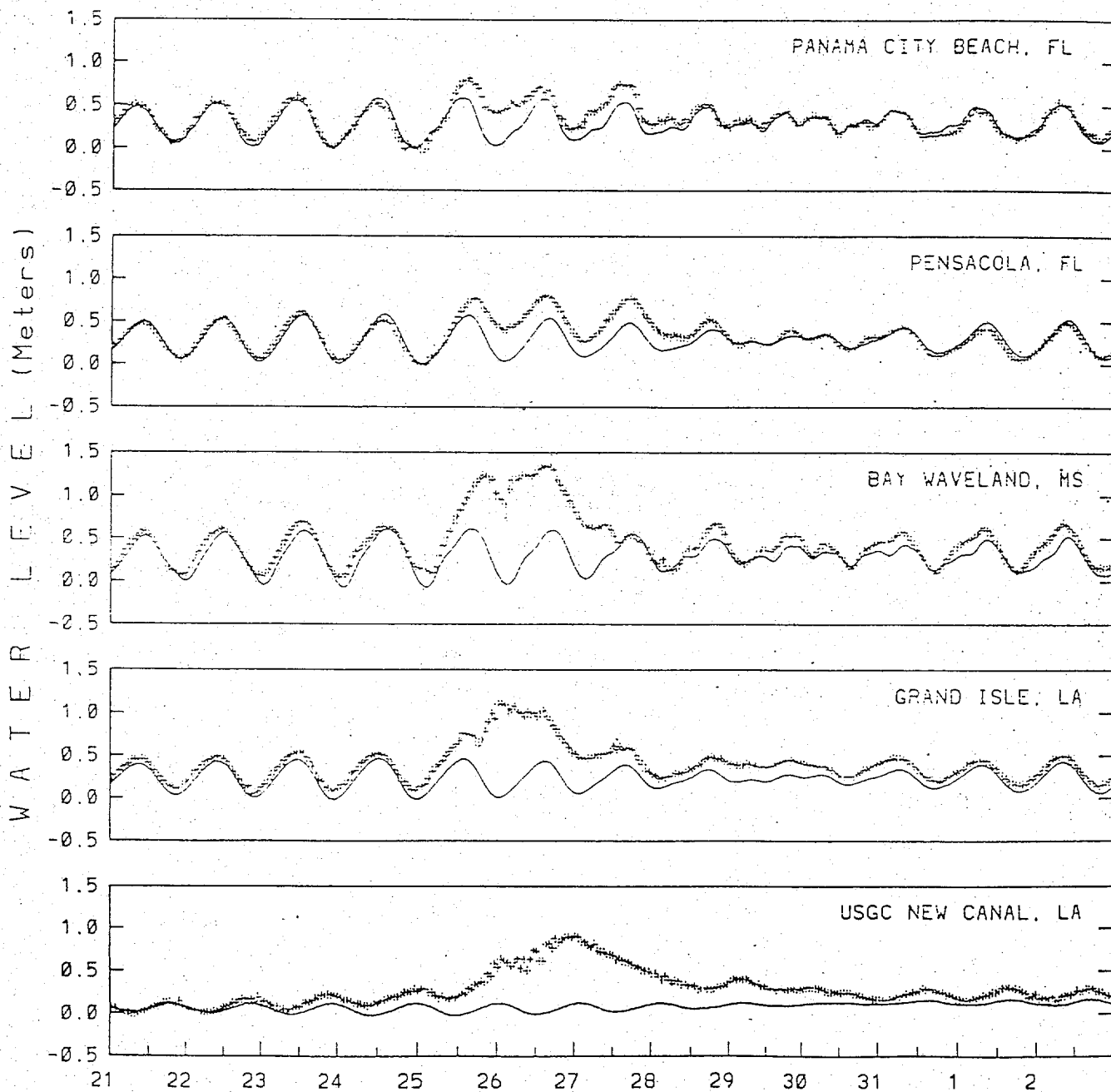
Figure 10. 21 AUGUST - 2 SEPTEMBER 1992 Observed and predicted hourly water level along the Florida panhandle and north gulf coast from 8/21/92 through 9/2/92 (see Table 4 for exact station locations).
