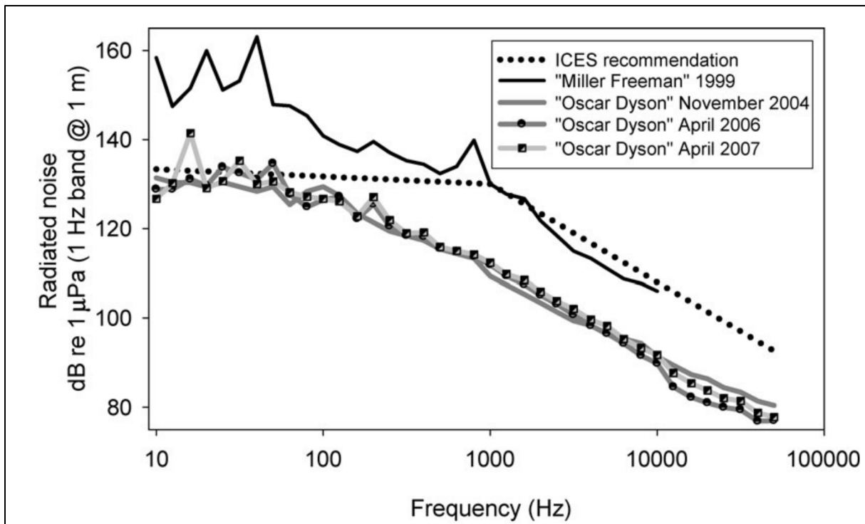
Figure 3.3-2. Underwater radiated-noise signature of the NOAA Research Vessels Miller Freeman and Oscar Dyson at speeds of 11 knots compared to the ICES recommendation for maxima for Research Vessel-radiated noise
