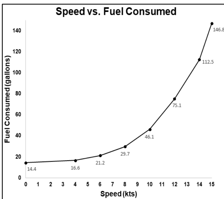
Figure 2.1-4. How Ship Speed Affects Fuel Consumption
