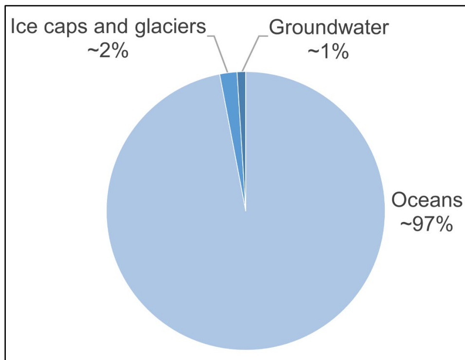
Figure 5.1-2. Global Composition of Water
