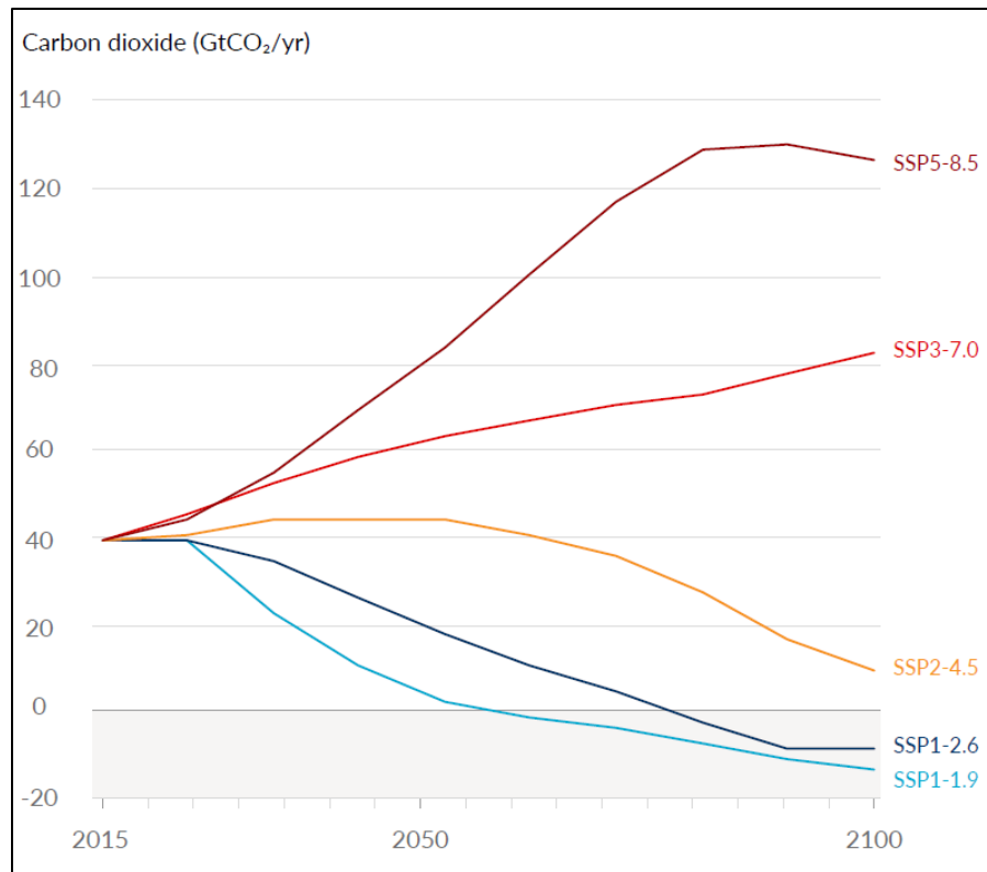
Figure 12.7-7. Future Emissions of CO 2 Under the AR6's Five Emissions Scenarios
