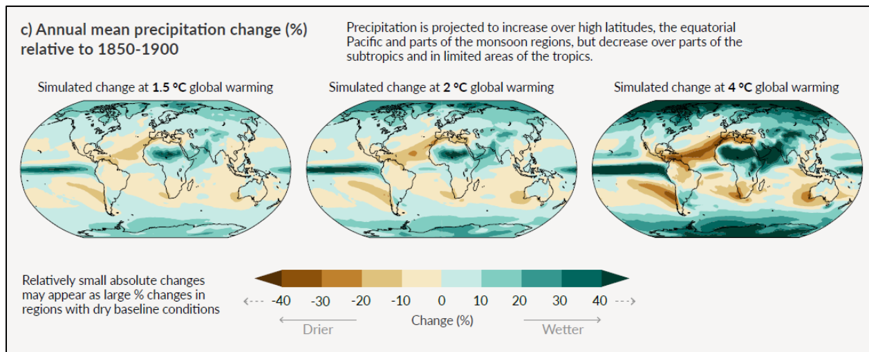
Figure 12.7-9. Change in Annual Mean Precipitation Relative to 1850-1900
