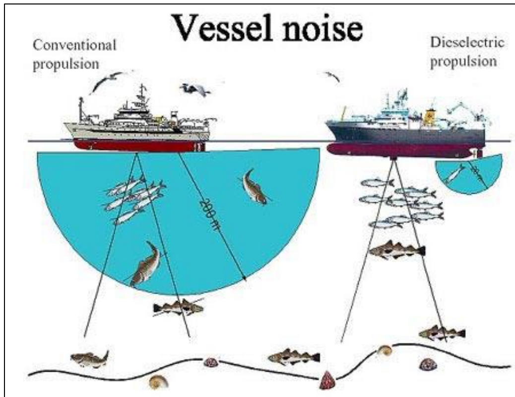
Figure 3.3-1. Underwater Radiated-Noise from Conventional versus Diesel-Electric Propulsion ( Oscar Dyson )
