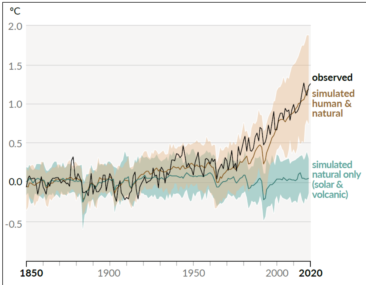
Figure 12.2-1. Global Surface Temperature Trends (1850-2020) as Observed (black) and Simulated Using Human and Natural (brown) and Natural Only Factors (green)
