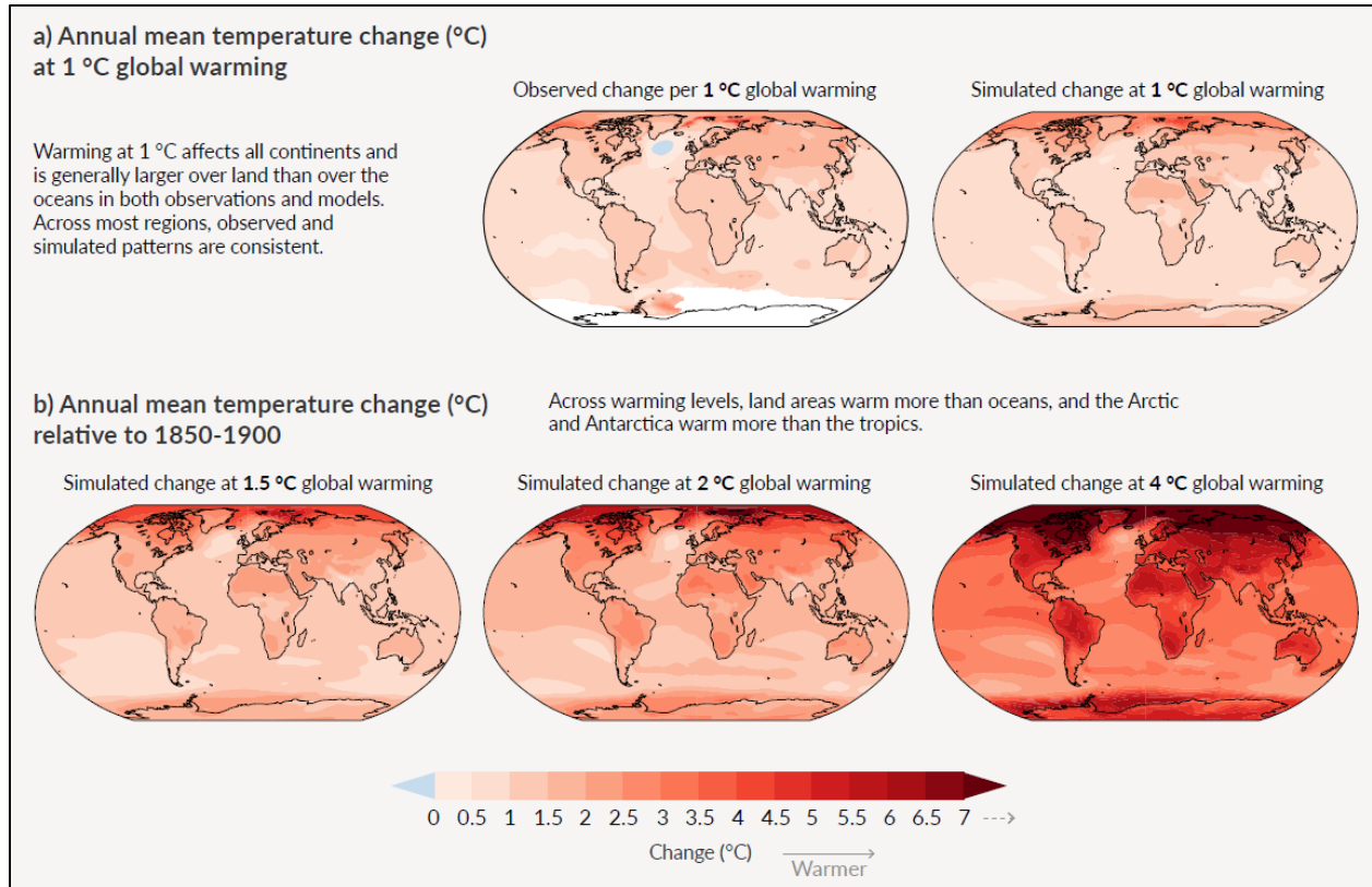
Figure 12.7-8. Observed and Simulated Mean Surface Air Temperature Change
