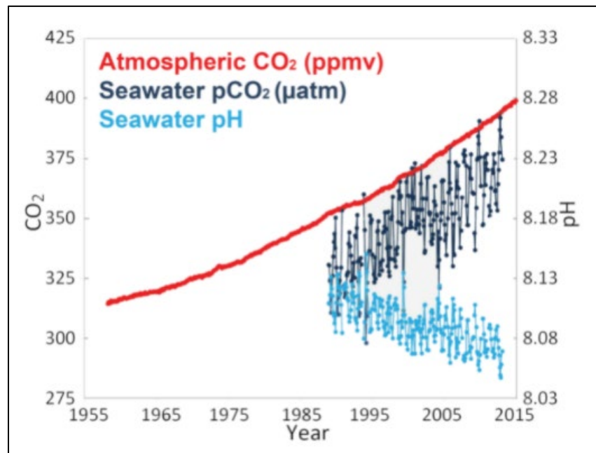
Figure 12.3-4. Time Series of Carbon Dioxide and Ocean pH at Mauna Loa, Hawaii
