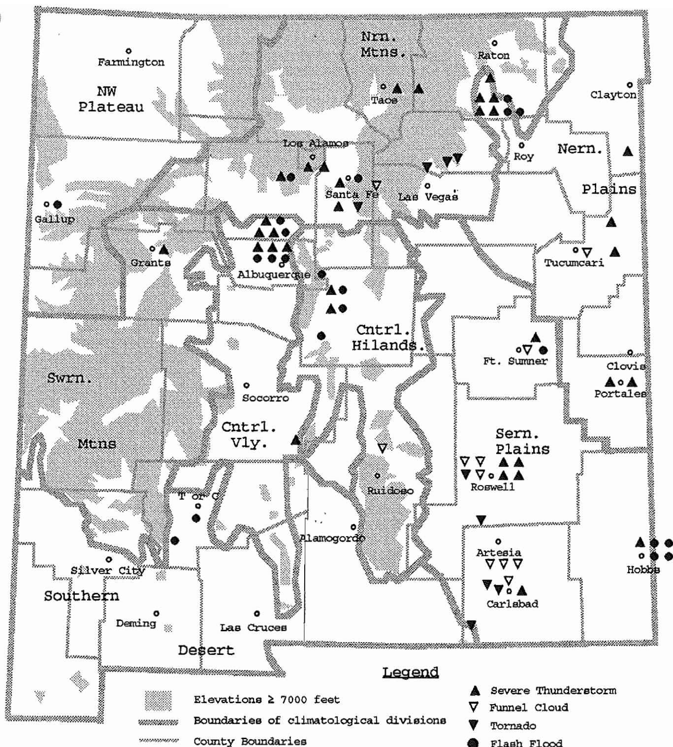
Figure 6. Location of severe storm events in New Mexico between 14 June 1990 and 26 September 1990 inclusive.
