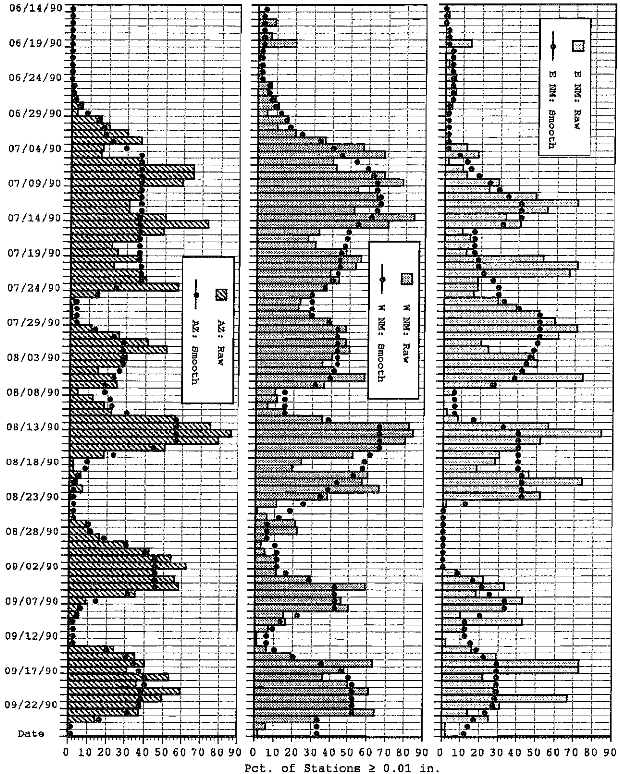
Figure 4. Bar and step charts showing the Daily Precipitation Indices from 14 June 1990 to 26 September 1990. The bar charts represent the raw DPIs in each DPI Zone, while the step charts represent smoothed DPI values.
