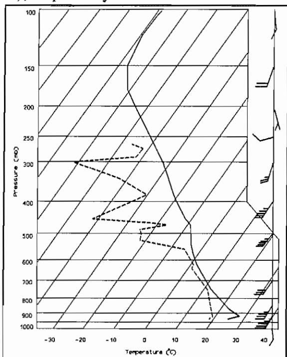
Figure 3. Oklahoma City sounding taken at 1200 UTC, 26 August 1987.
