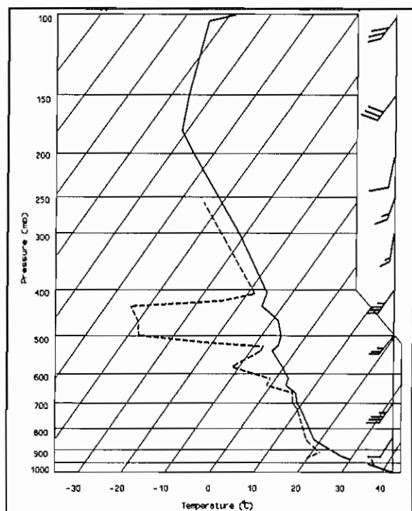
Figure 4. Oklahoma City sounding taken at 0000 UTC, 27 August 1987.
