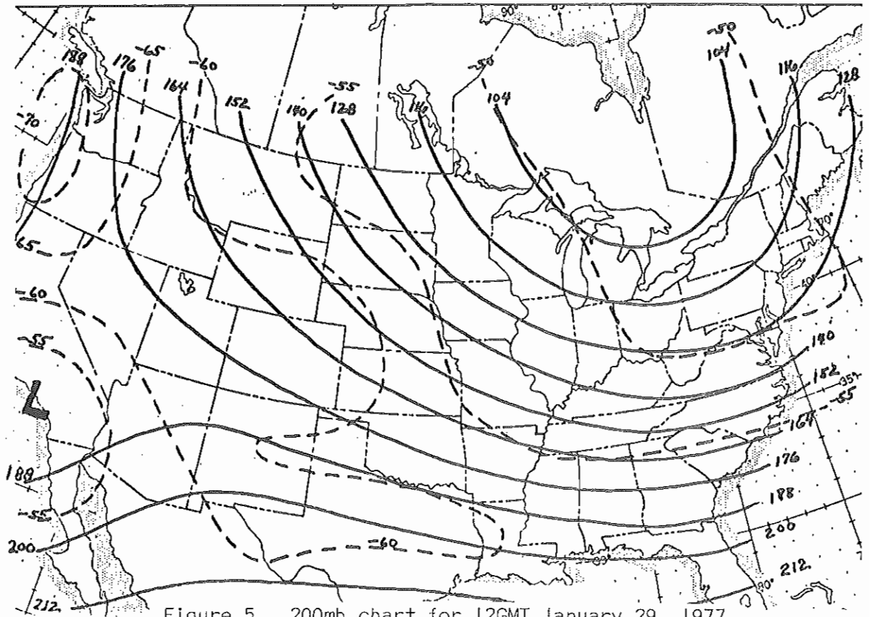
Figure 5. 200mb chart for 12GMT January 29, 1977.
