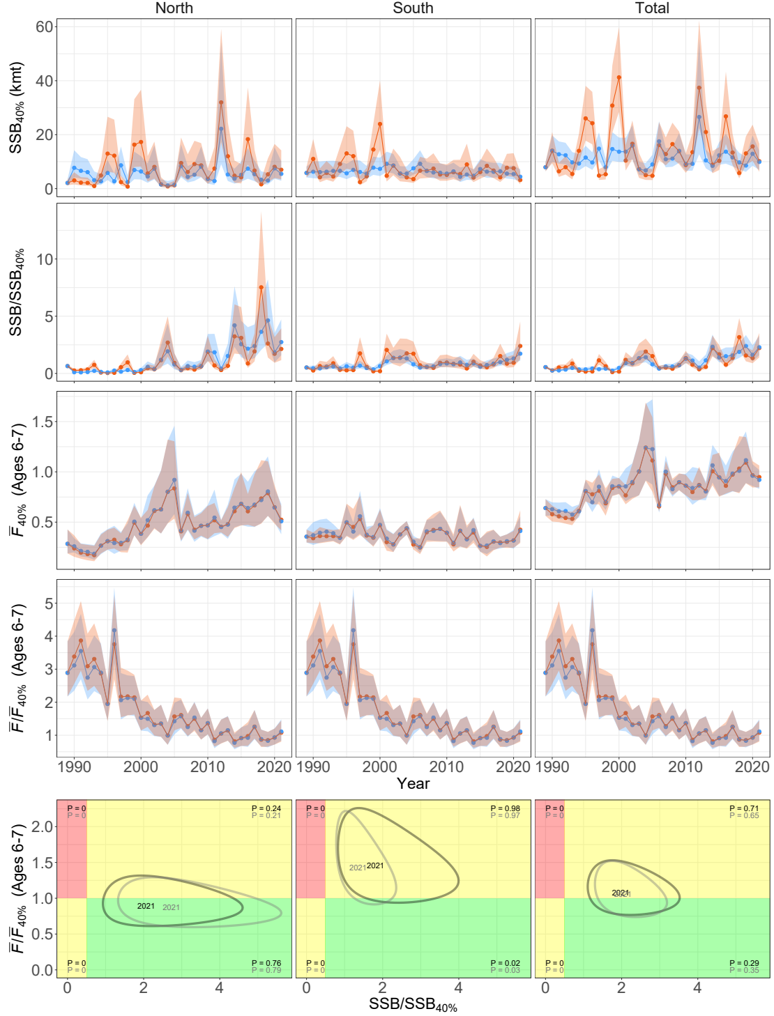
Figure 6: Estimates of average equilibrium F at ages 6 and 7 that produces the 40% spawning potential ratio ( F_{40\%} ), equilibrium SSB at F_{40\%} based on annual inputs to \phi(F) calculations, annual fishing and biomass status (ratios), and bivariate kobe plots of status in 2021 where reference points represent prevailing conditions with inputs to \phi(F) averaged over the last 5 years and recruitment is averaged over the time series. Red and blue in first 4 rows and black and gray in final row indicate alternative annual estimates of recruitment (random effect or expected). All results are based on model M_1 . Polygons represent 95% confidence intervals or regions.
