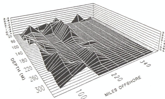
Figure 2. Three dimensional surface representation of the distribution of acoustic volume reverberation along CalCOFI line 93 which intercepts the coastline at Del Mar and proceeds at a direction of 240°, as a function of depth and distance off the coast. Each depth line is 8 meters. The amplitude of the reverberation is expressed in normal units (standard deviations above the mean). The vertical lines begin within 15 miles of the coast and are at 40 mile intervals. These lines coincide in time with the standard CalCOFI bongo tow.
