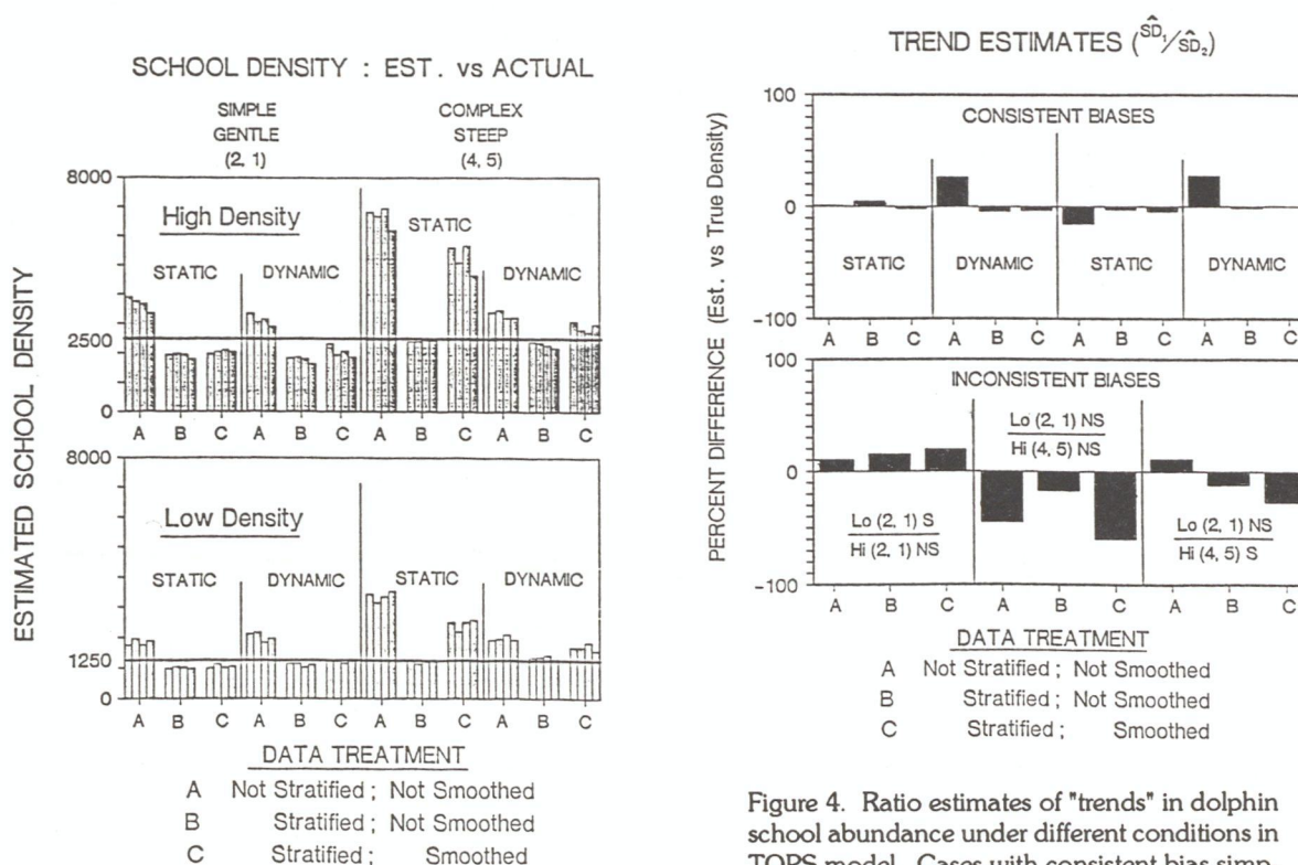
Figure 3. Estimates of school abundance under different conditions in TOPS model. Sets of four columns are replicates.
