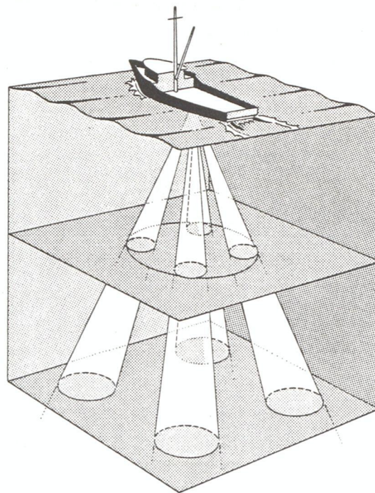
Figure 1. Diagram of the position and orientation of the 4 transducers of the acoustic doppler current profiler (ADCP) used on the New Horizon CalCOFI cruise of August 1988.
