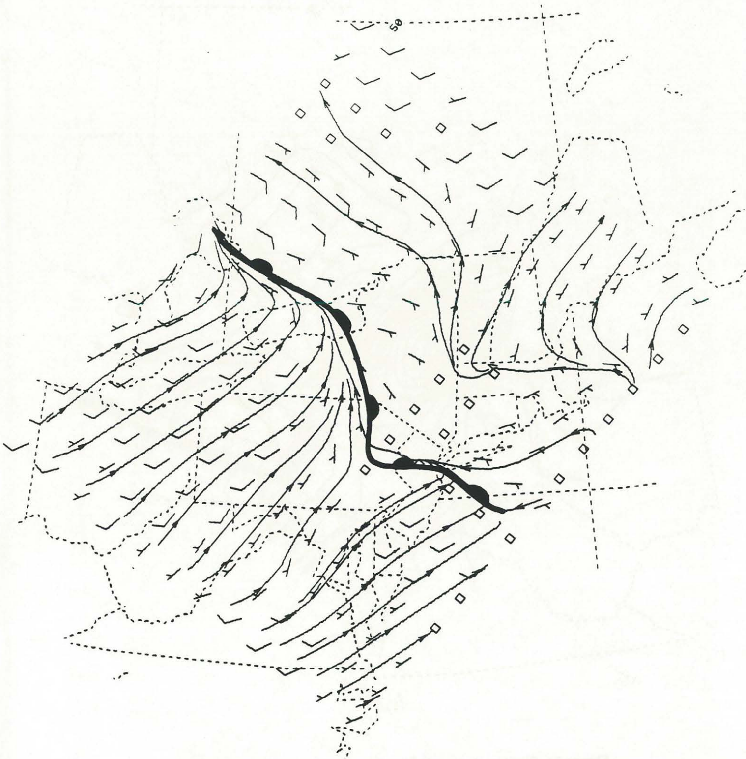
Figure 20. Surface streamlines/wind plot for 1500 UTC, June 29, 1990.
