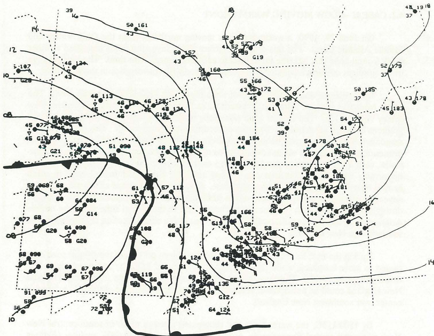
Figure 12. Surface plot and analysis for 1700 UTC, May 20, 1990.
