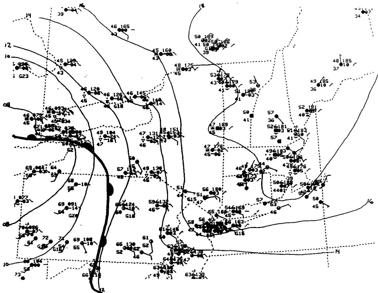
Figure 9. Surface plot and analysis for 1500 UTC, May 20, 1990.
