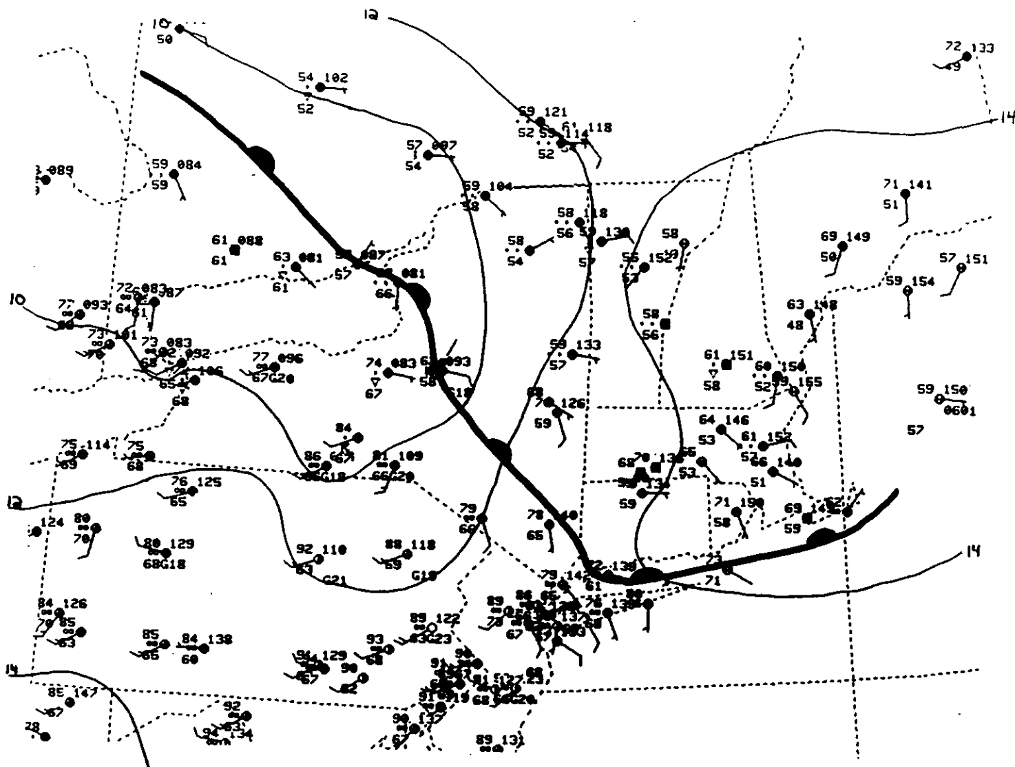
Figure 26. Surface plot and analysis for 1900 UTC, June 29, 1990.
