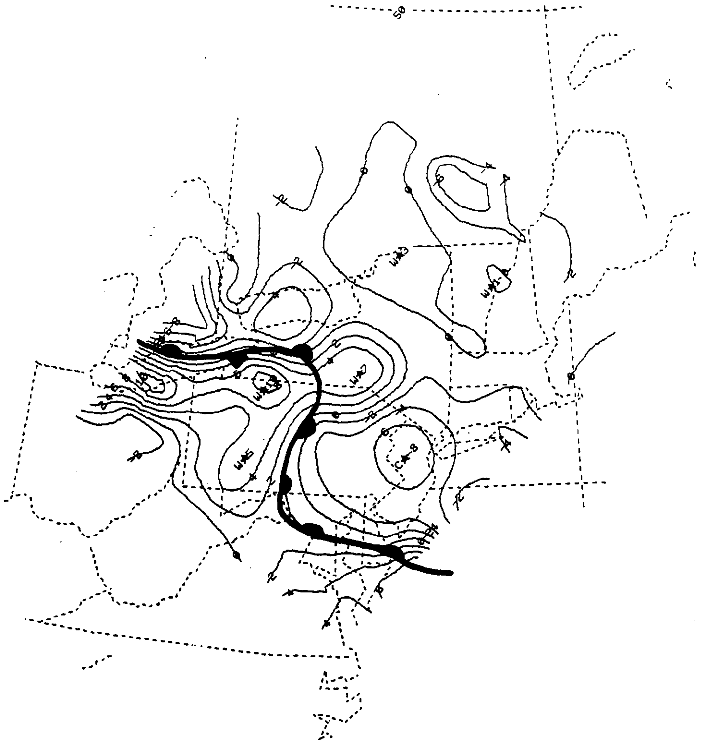
Figure 10. Surface theta advection for 1700 UTC, May 20, 1990.
