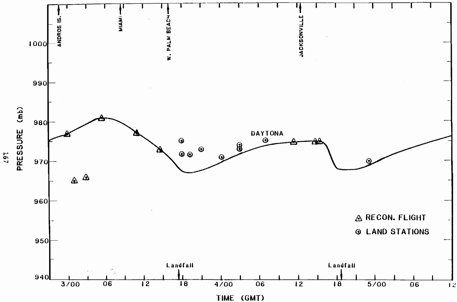
Figure A.15.--Central pressure (sea-level) for Hurricane David, September 3-5, 1979.
