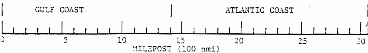
Figure 6.--Possible homogeneous regions for landfalling hurricane parameters. Shaded areas have insufficient or no data.
