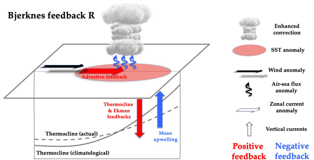
Figure 6. The Bjerknes feedback. Overview of the physical processes involved in the Bjerknes feedback loop, here for the example of a positive SST anomaly. A warm SST anomaly induces enhanced deep atmospheric convection, and westerly wind anomalies through the Gill (1980) response. This leads to negative surface heat flux anomalies (less shortwave, more evaporation), a negative feedback on the SST anomaly. The background circulation also tends to damp the warm anomaly, for instance through the mean upwelling of cold water. On the other hand, the fast oceanic response through downwelling Kelvin waves (assumed to be instantaneous in the RO) is associated with anomalous thermocline deepening in the eastern equatorial Pacific. The associated thermocline feedback favors the development of warm SST anomalies. Wind relaxation along the equator also contributes to surface warming through zonal, meridional and vertical (or Ekman) advection feedbacks. Together, these positive feedbacks control the strength of the Bjerknes feedback. The intensity of both positive and negative feedbacks depend on the background state, and the seasonal cycle leads to a slightly negative R value in spring and early summer. Positive feedbacks take over the thermal damping and damping by the mean circulation from roughly June to December (e.g., Jin et al. (2020)). The overall ENSO stability given by \frac{R-\epsilon}{2} is usually positive in fall, and weakly negative on annual average (Sections 4.1 and 4.2).
