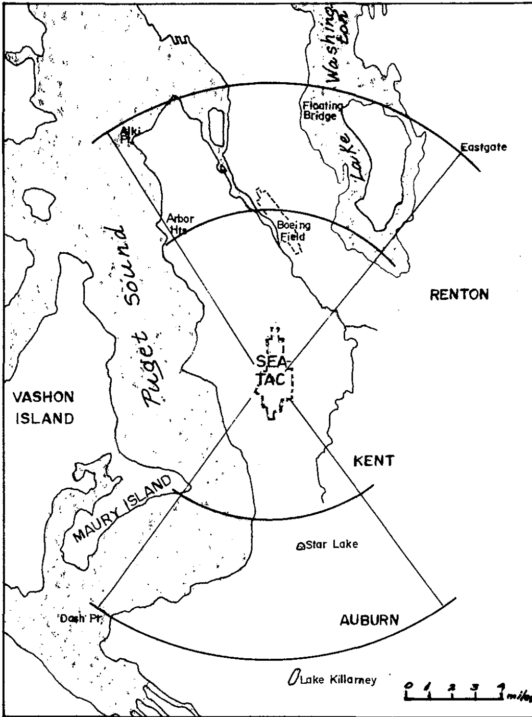
FIGURE 4. MAP OF SEATTLE-TACOMA AIRPORT VICINITY.
