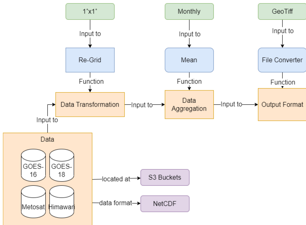
Figure 4.3. Simplified illustration of how knowledge graphs can map actions performed on datasets. This can create greater transparency for NOAA open science goals and better error and uncertainty tracking within processes.
