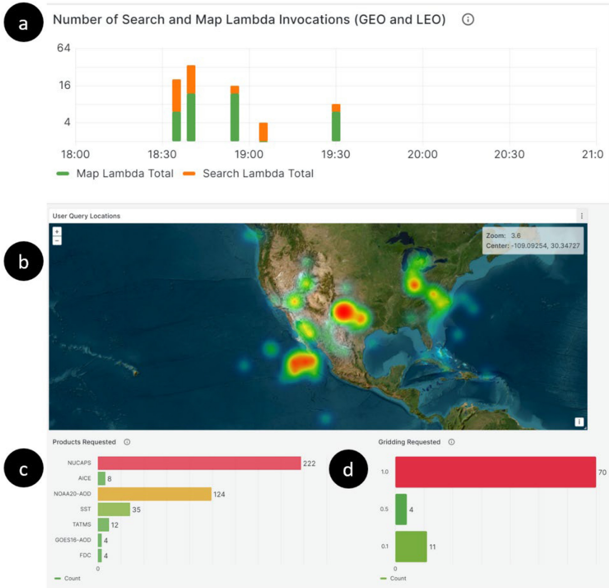
Figure 1.17. Figure 1.17 The dashboard showing analytics of how users interacted with the user interface.
