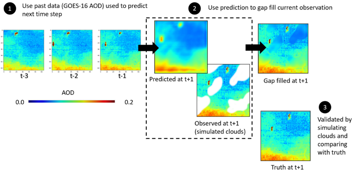
Figure 3.10. Proof of concept for gap filling in an EO-DT. In 1, a convLSTM model predicts the next time step ( t+1 ) using the past three-time steps of AOD ( \sim 1 hour of past data). In 2, the predicted AOD is compared with AOD observed at t+1 , regions observed with simulated missing clouds can be replaced with the predicted values. Results can be validated using the unmodified t+1 observed values, where the clouds have not been removed.
