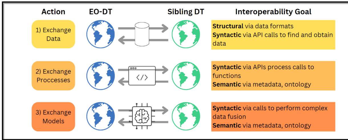
Figure 5.2. Three milestones to better understand structural, syntactic, and semantic interoperability between digital twins. After partnering with a sibling effort, we recommend that NESDIS work toward exchanging data, processes, and models.
