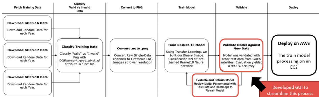
Figure 1.6. The development workflow for the machine learning anomaly detection method tested in our demonstration.
