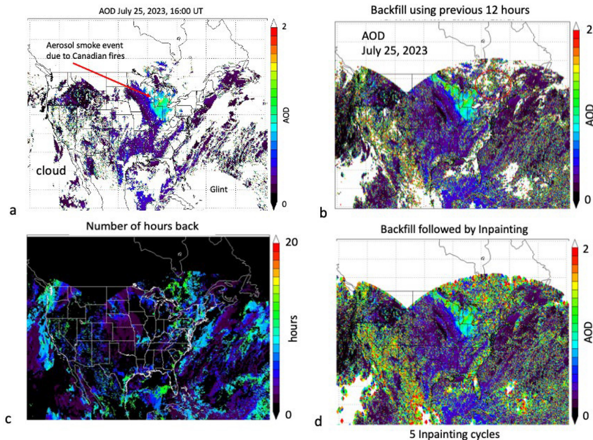
Figure 2.8. Illustration of backfilling using combined GOES-16 and NOAA-18 AOD
