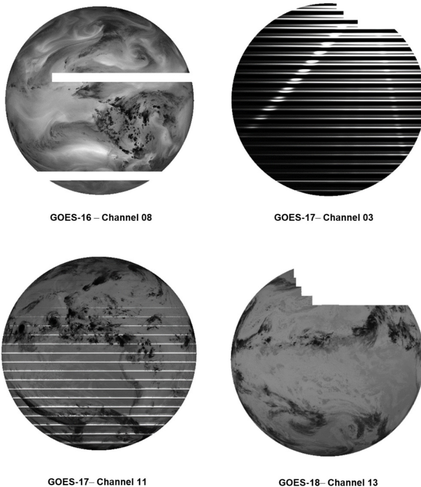
Figure 3.1. Example of anomalies from GOES-R series L1b data showing missing data with various patterns.
