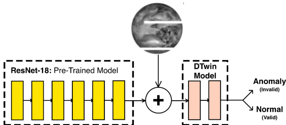
Figure 1.5. Simple overview of how ResNet-18 in operations.
