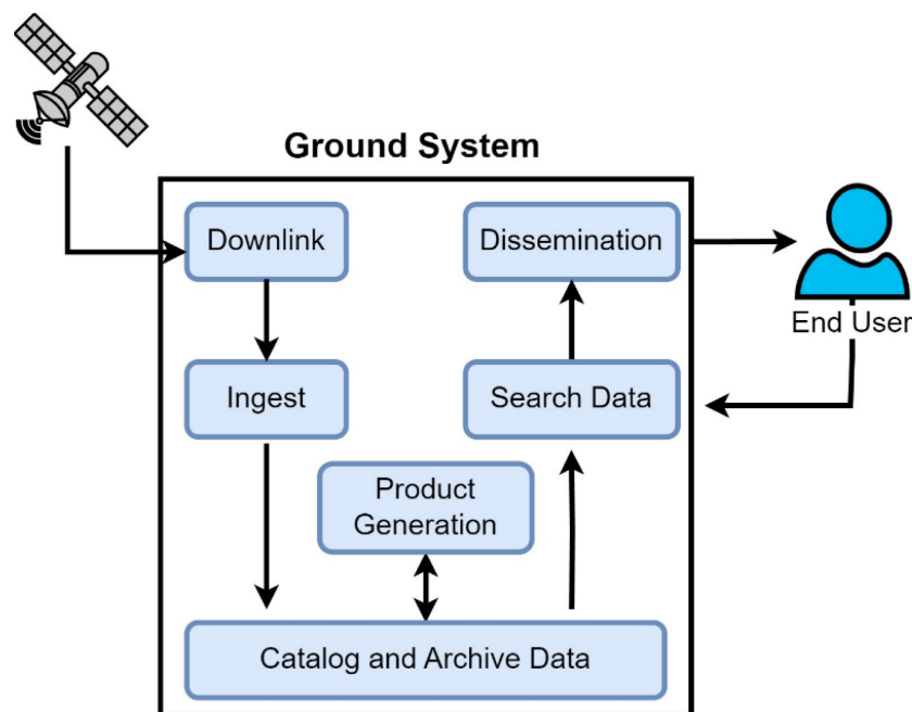
Figure 1.1. Simplified diagram of core processes in the NESDIS ground system. These are the core processes that need to be monitored and scaled to ensure timely data delivery to users.
