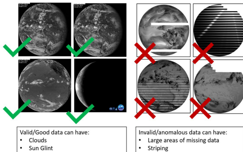
Figure 1.4. Examples of good quality GOES imagery (left) and imagery that has anomalies present (right).
