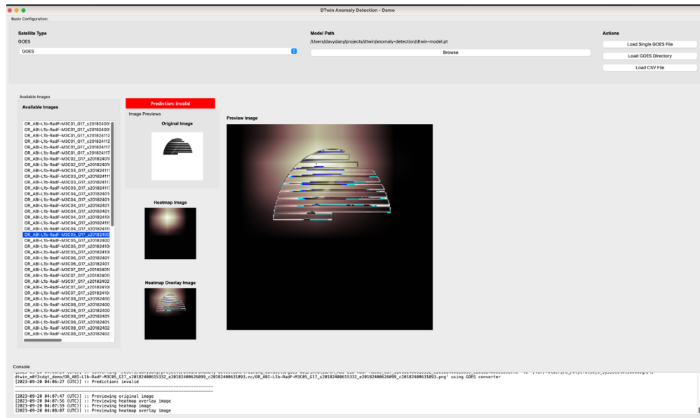
Figure 1.7. Demo #2: ML-based data anomaly detection models
