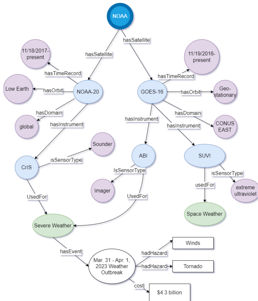
Figure 4.1. Illustration of knowledge graph connecting NOAA satellite assets (“NOAA-20”), their properties (“global”), and the relationships between them (“hasDomain”). Knowledge graphs can improve the searchability and discovery of datasets as well as link to other databases to create a larger, interconnected federation. Consistent metadata formats are a key requirement for success.
