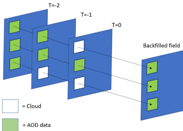
Figure 2.7. technique for AOD. Data is brought forward in time to fill in regions obscured by glint and clouds.
