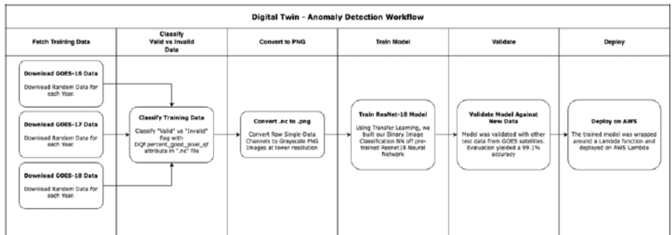
Figure 3.3. Overview of the Anomaly Detection Workflow for GOES data.
