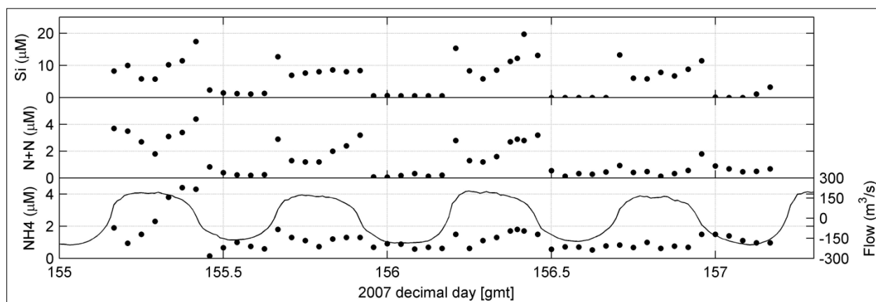
Figure 4a. Concentration data from AOML for the June 2007 intensive versus time (GMT). Analytic concentrations are denoted in the left-most vertical axis. The solid line (bottom panel) represents the flow through the inlet (denoted in the right-hand axis), with positive values being seaward (ebb tide) flow.
