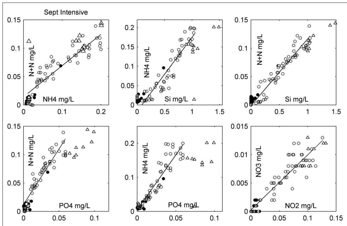
Figure 8. Nutrient concentration data from the September intensive (lower panels). Format is similar to Figure 7a. Regressions for the September flood (●) and high-P (Δ) data are not displayed because of the lack of fit. Regression values (coefficient of determination) for the September ebb tide data (denoted by ○) are as follows: N+N/NH4 R^2=0.708 , NH4/Si R^2=0.878 , N+N/Si R^2=0.917 , N+N/PO4 R^2=0.862 , NH4/PO4 R^2=0.860 , NO3/NO2 R^2=0.819 .
