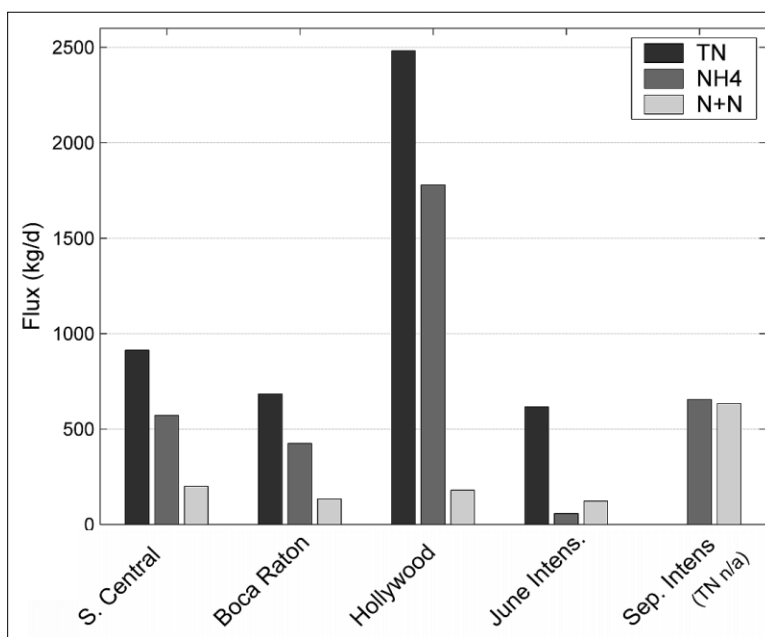
Figure 11. Comparison of nutrient fluxes from three treated-wastewater plant ocean outfalls and the two 48-hour sampling intensives at Boynton Inlet. TN was not measured during the September intensive.
