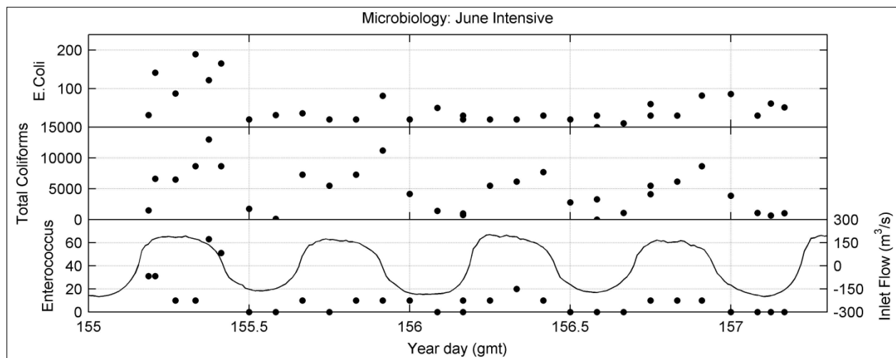
Figure 4c. Microbiology assessments from the June 2007 intensive. Format is similar to Figure 4a. Units for all three measurements are MPN/100ml.
