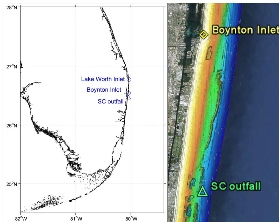
Figure 1. Left: Location of the Boynton and Lake Worth Inlets, which drain the Lake Worth Lagoon, and the South Central treated-wastewater plant ocean outfall. Right: vicinity of the Boynton Inlet and South Central outfall (Google Earth).
