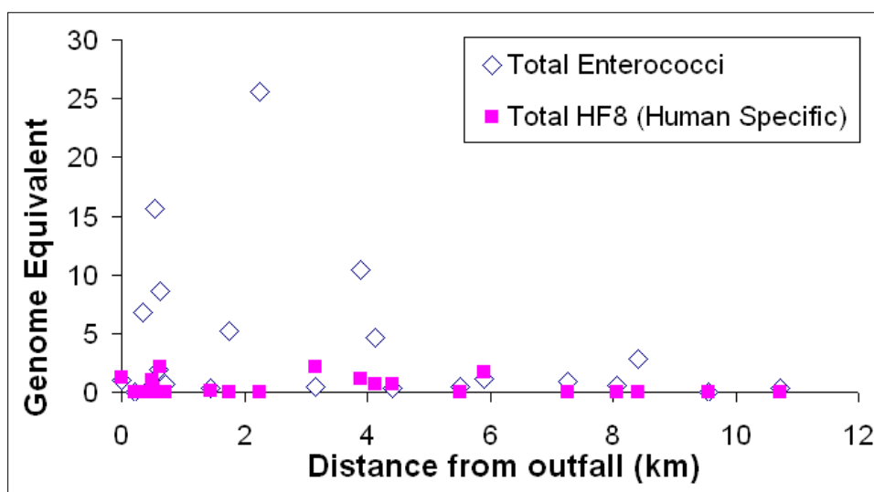
Figure 15. The abundance (genome equivalents) of enterococci and a human-specific Bacteroides (HF8) as measured by qPCR versus distance from the South Central wastewater-treated plant ocean outfall (data from a July 2008 R/V Walton Smith cruise, C. Sinigalliano, personal communication).
