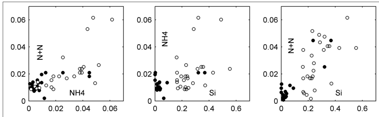
Figure 7. Nutrient concentration data from the June intensive. Open symbols refer to ebb tide measurements while closed symbols indicate flood tide measurements. Regression lines were not drawn because of lack of fit. Concentration units are mg/L.
