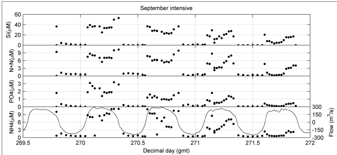
Figure 5. Concentration data for Si, N+N, P, and NH 4 for the September 2007 intensive, all versus time (GMT). Format is similar to Figure 4a. Note the higher flow rates in comparison to the June intensive.
