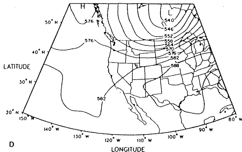
Figure 82. (continued) As in Figure 44.
