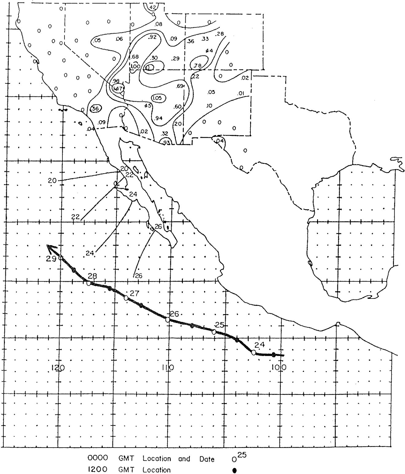
Figure 51. Track of the Tropical Storm of September 23-29, 1951 and associated rainfall in the Southwest. Precipitation totals are in inches and the isohyets are drawn at .01, .25, .50, and 1.00 inches. Sea surface temperatures are in °C.
