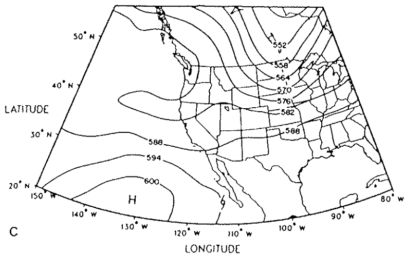
Figure 74. As in Figure 44.
