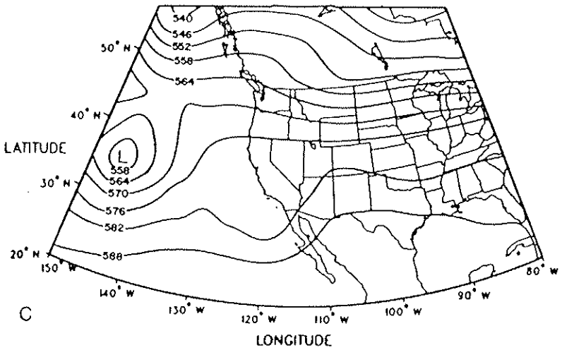
Figure 131. As in Figure 44.
