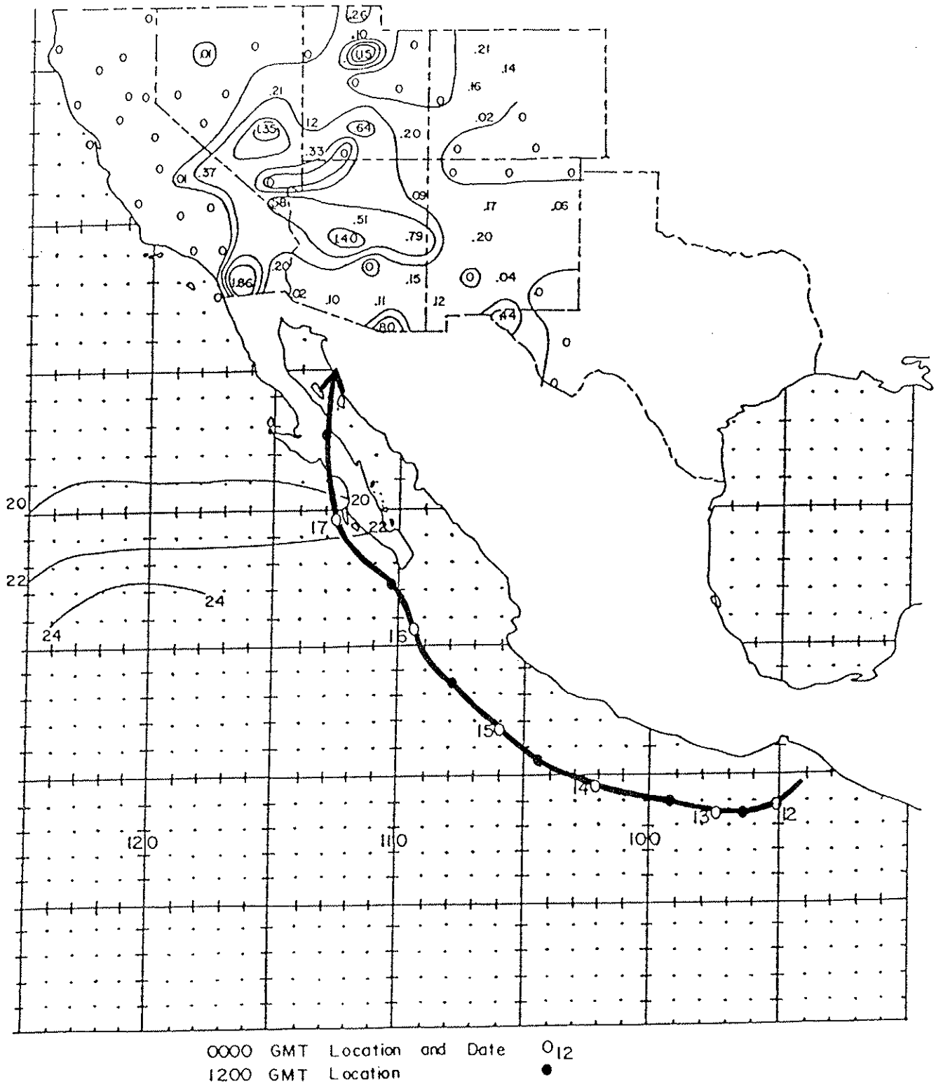
Figure 57. Track of the Hurricane of July 11-17, 1954 and associated rainfall in the Southwest. Precipitation totals are in inches and the isohyets are drawn at .01, .25, .50, and 1.00 inches. Sea surface temperatures are in °C.
