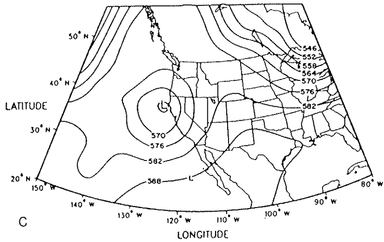
Figure 120. As in Figure 44.
