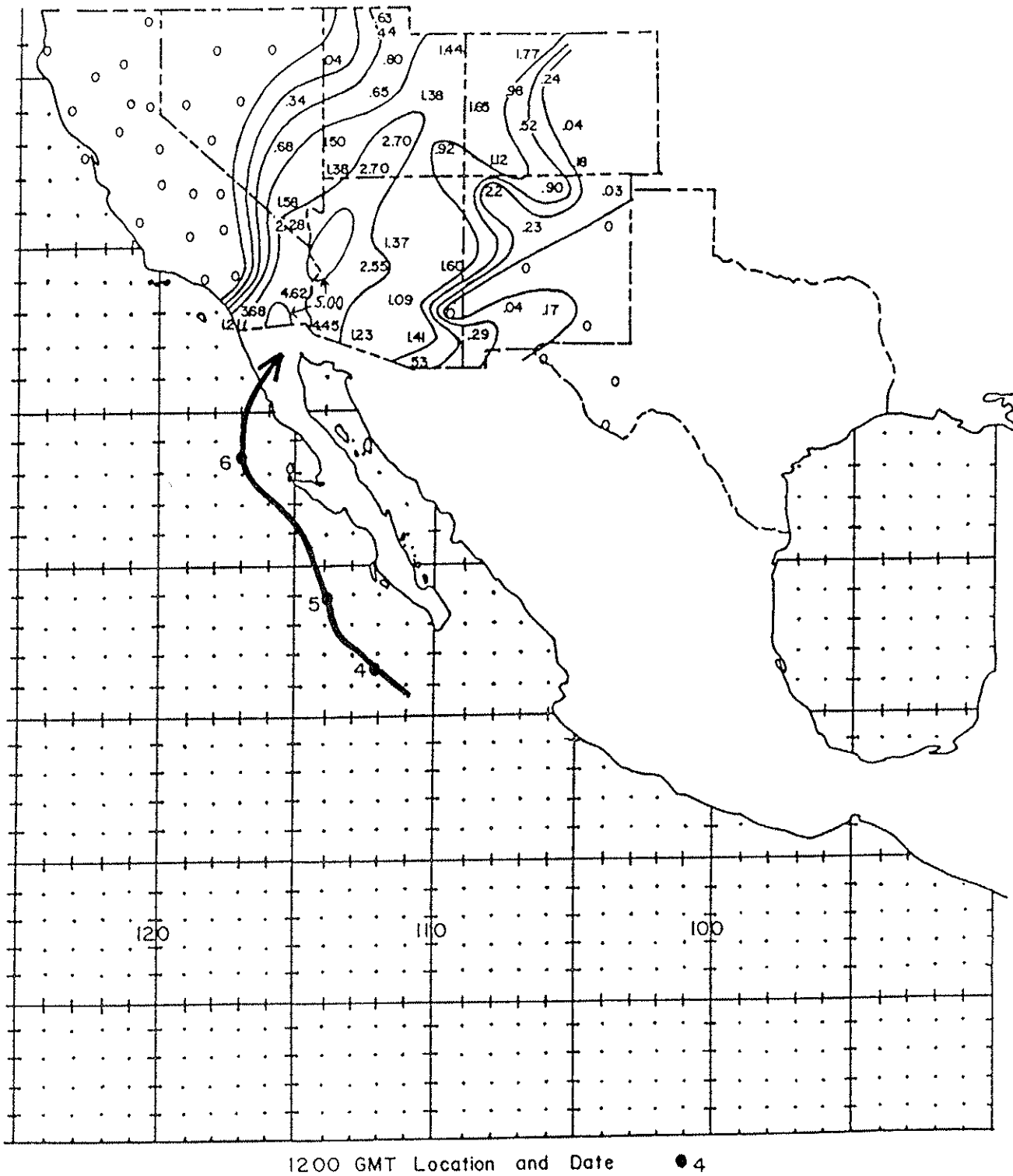
Figure 37. Track of the Tropical Cyclone of September 4-6, 1939 and associated rainfall in the Southwest. Precipitation totals are in inches and the isohyets are drawn at .01, .25, .50, 1.00, 2.00, and 5.00 inches.
