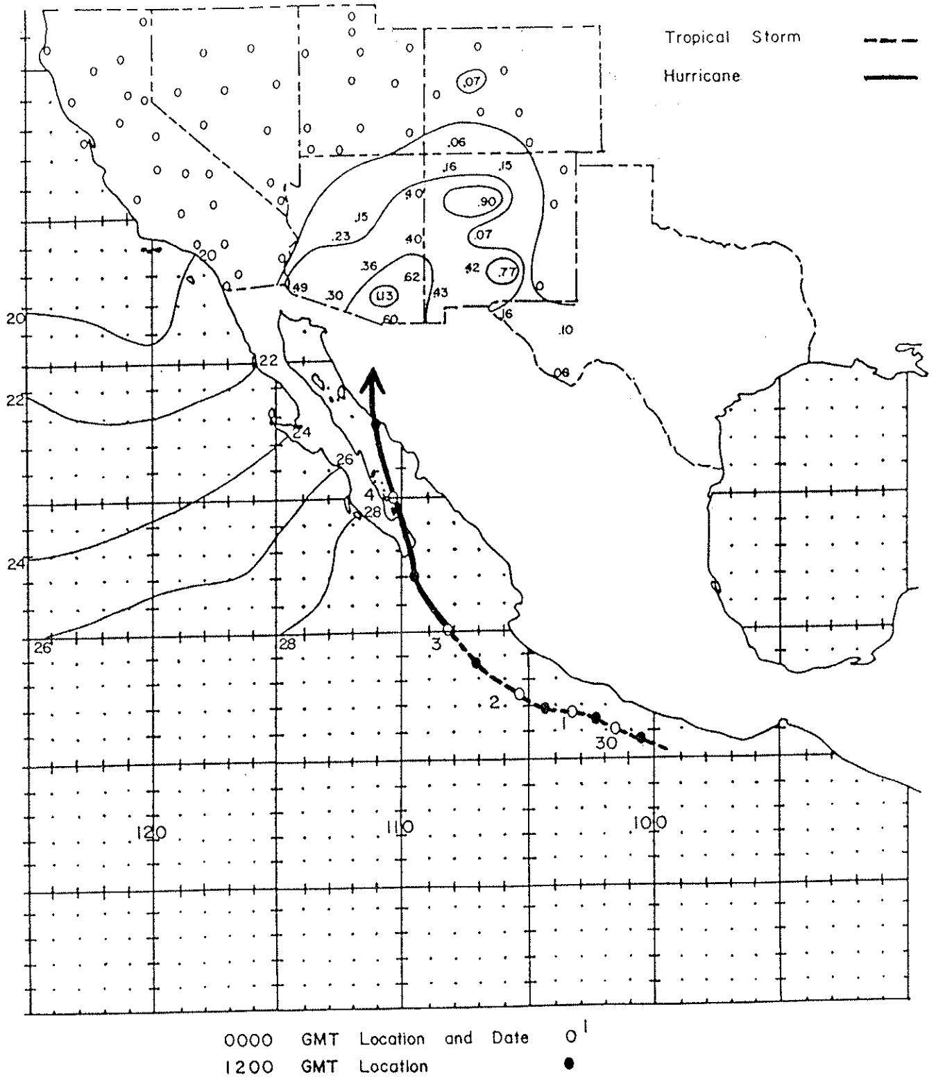
Figure 67. Track of the Hurricane of September 29 - October 4, 1958 and associated rainfall in the Southwest. Precipitation totals are in inches and the isohyets are drawn at .01, .25, .50, and 1.00 inches. Sea surface temperatures are in °C.
