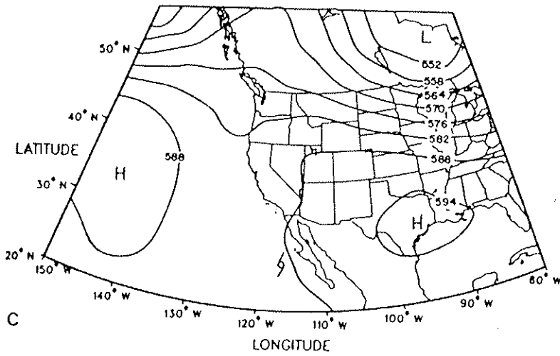
Figure 62. As in Figure 44.
