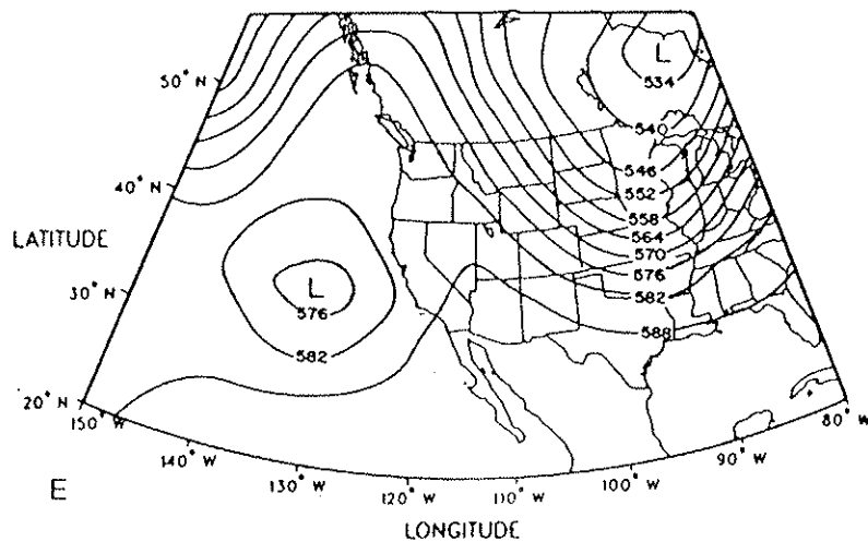
Figure 126. (continued) As in Figure 44.
