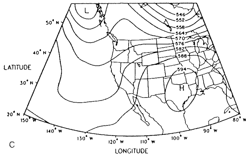
Figure 118. As in Figure 44.
