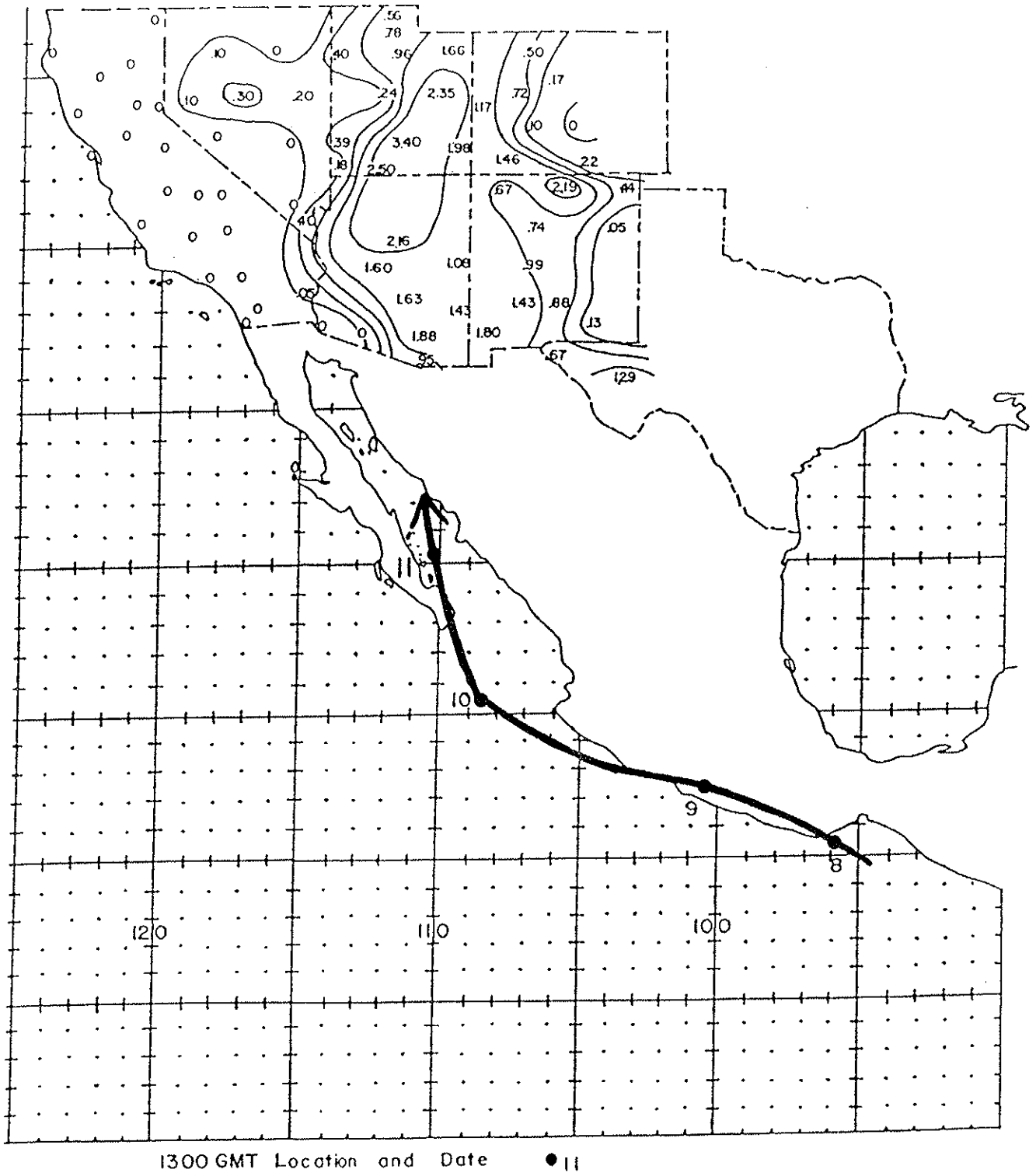
Figure 26. Track of the Hurricane of September 7-12, 1927 and associated rainfall in the Southwest. Precipitation totals are in inches and the isohyets are drawn at .01, .25, .50, 1.00, and 2.00 inches.
