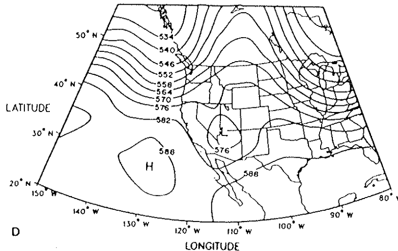
Figure 92. (continued) As in Figure 44.
