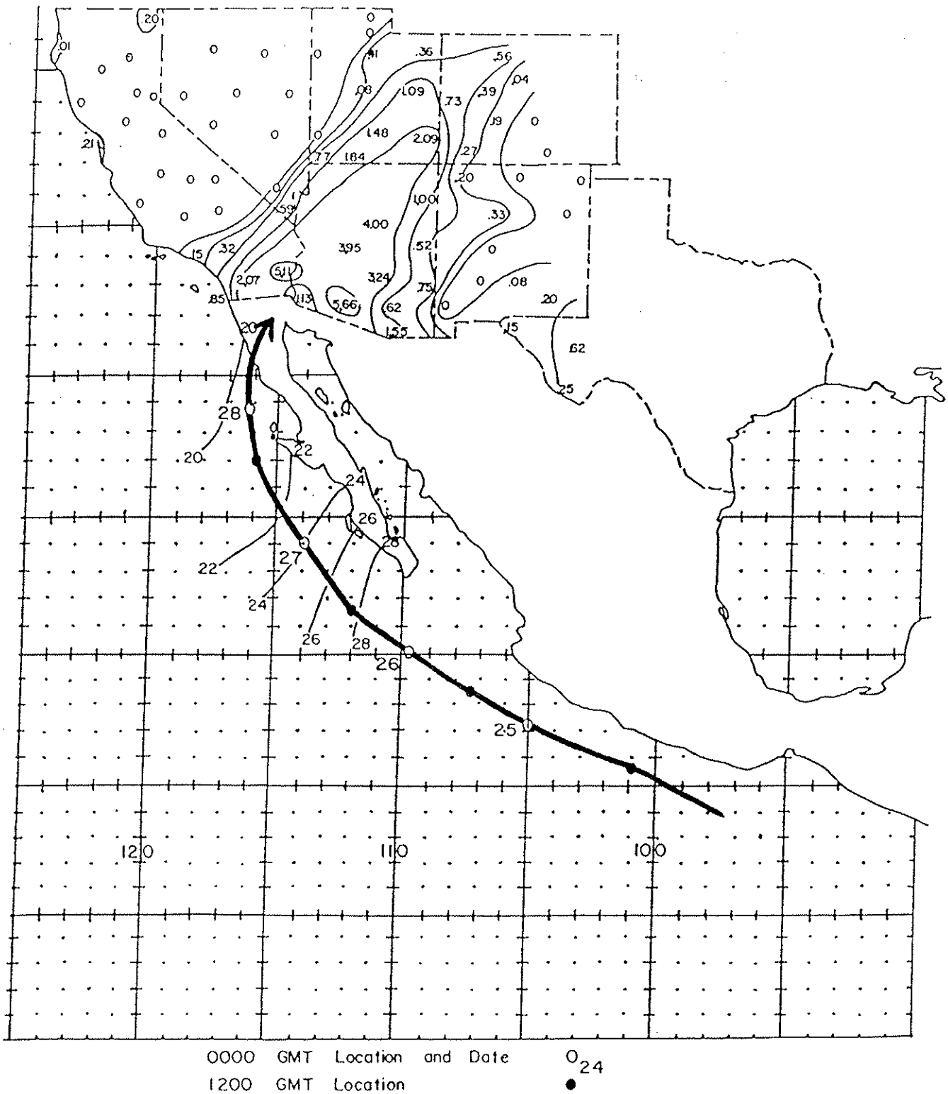
Figure 49. Track of the Hurricane of August 24-28, 1951 and associated rainfall in the Southwest. Precipitation totals are in inches and the isohyets are drawn at .01, .25, .50, 1.00, 2.00, and 5.00 inches. Sea surface temperatures are in °C.
