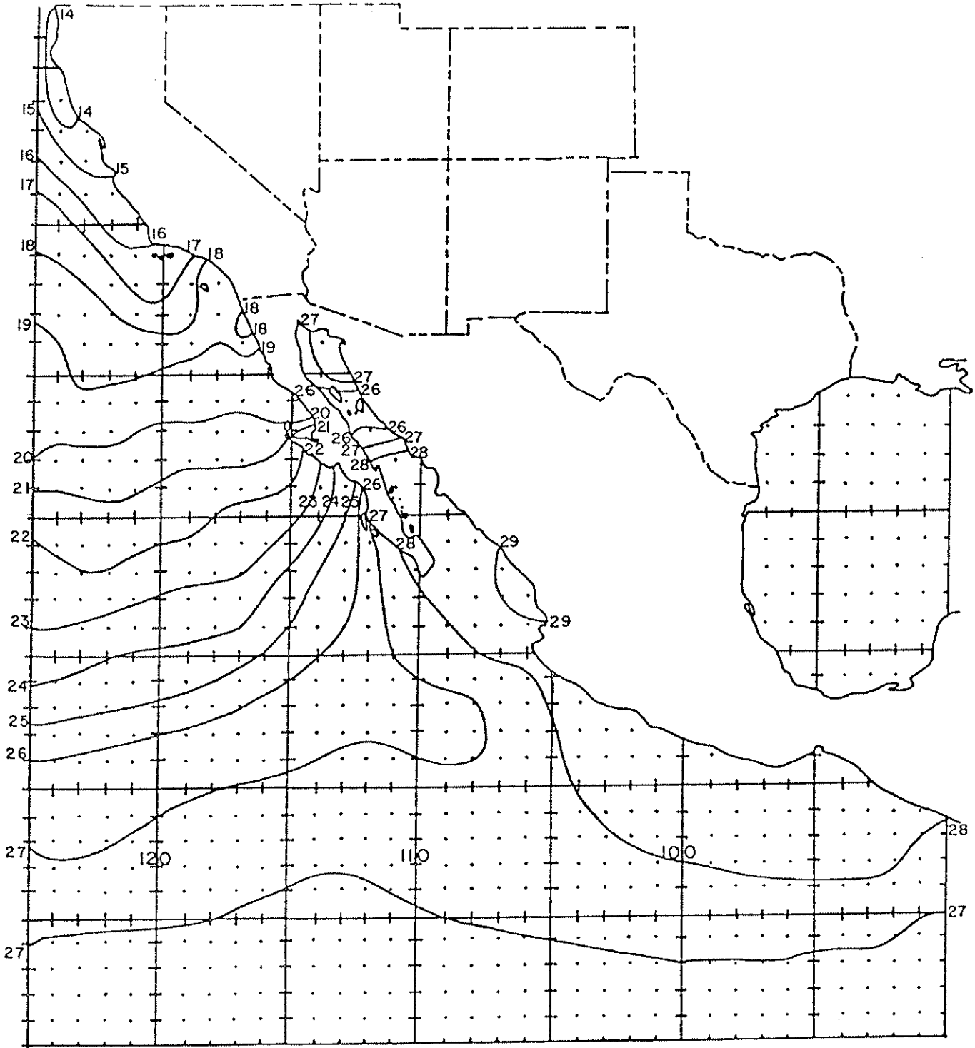
Figure 6. Mean sea surface temperatures for October. Temperature are in °C and the contour interval is 1° (from Oceanographic Monthly Summary Sea Surface Temperature Climatology , April 1982).
