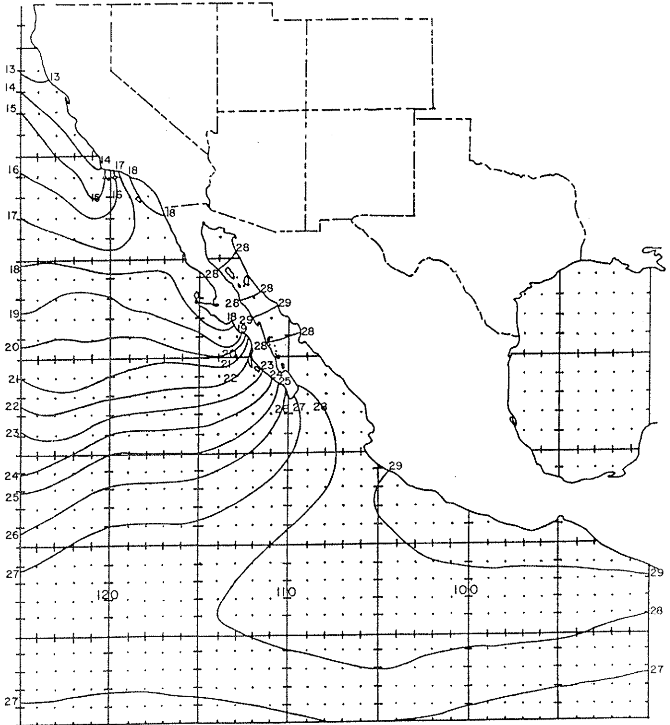
Figure 3. Mean sea surface temperature for July. Temperatures are in °C and the contour interval is 1° (from Oceanographic Monthly Summary Sea Surface Temperature Climatology , April 1982).
