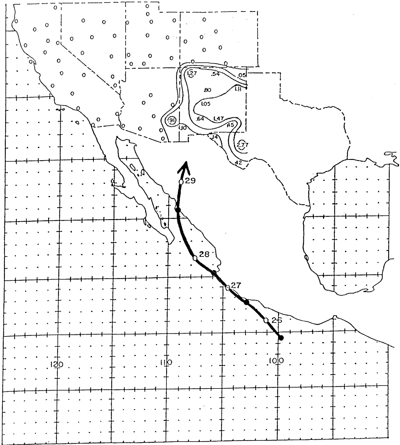
Figure 31. Track (from Court, 1980) of the Tropical Cyclone of August 25-29, 1932 and associated rainfall in the Southwest. Precipitation totals are in inches and the isohyets are drawn at .01, .25, .50, 1.00, and 2.00 inches.
