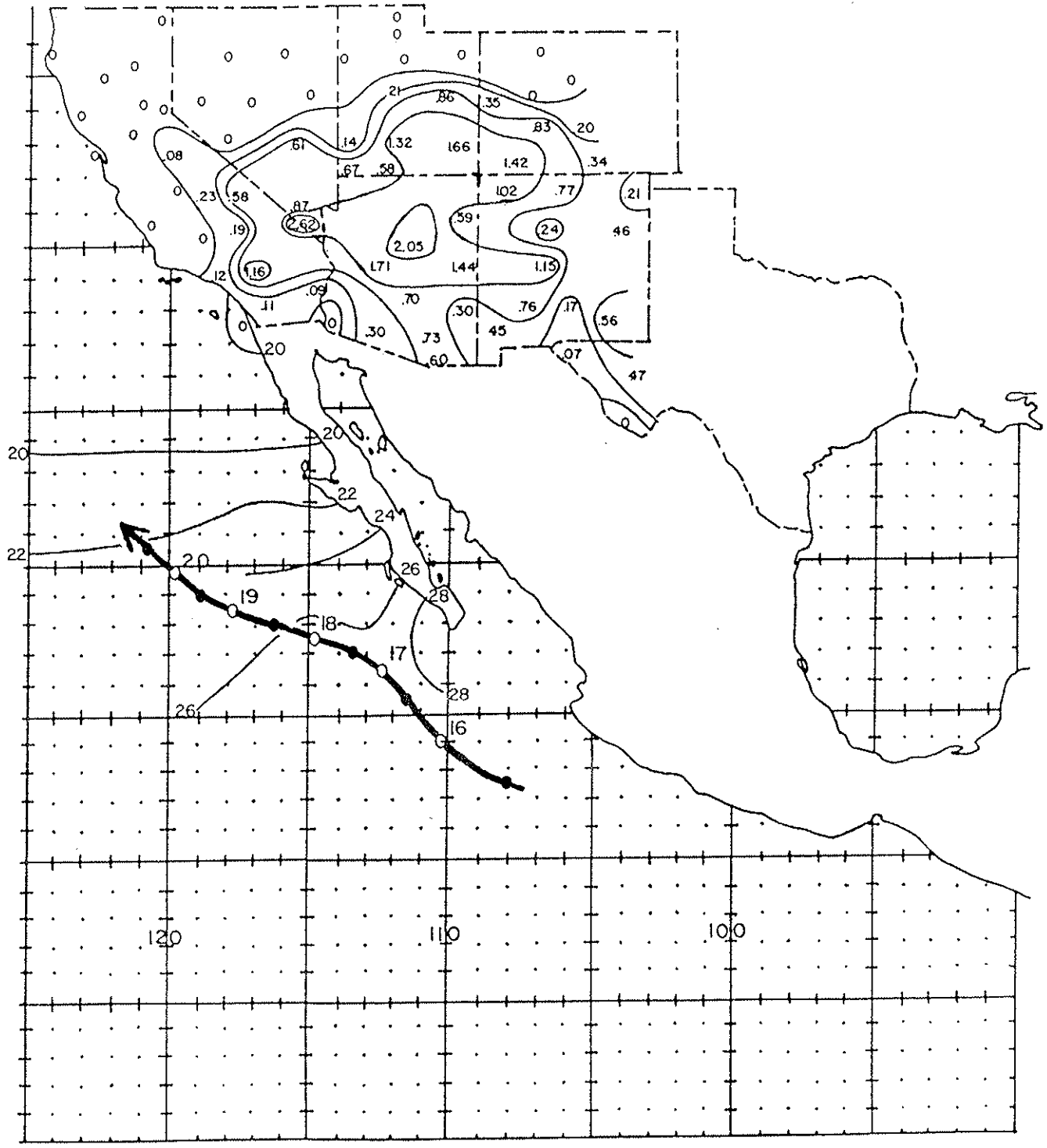
Figure 53. Track of the Tropical Storm of September 15-21, 1952 and associated rainfall in the Southwest. Precipitation totals are in inches and the isohyets are drawn at .01, .25, .50, 1.00, and 2.00 inches. Sea surface temperatures are in °C.
