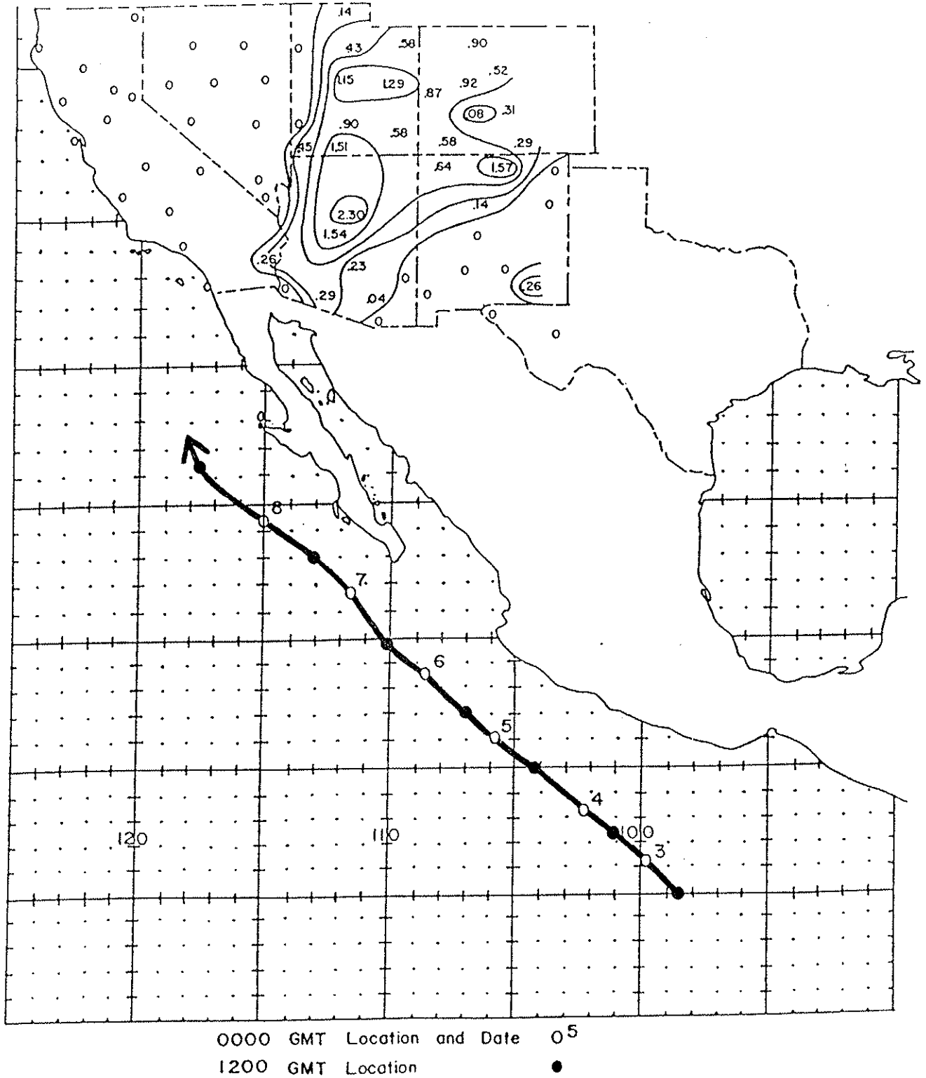
Figure 20. Track (from Court, 1980) of the Tropical Cyclone of September 2-8, 1924 and associated rainfall in the Southwest. Precipitation totals are in inches and the isohyets are drawn at .01, .25, .50, 1.00, and 2.00 inches.
