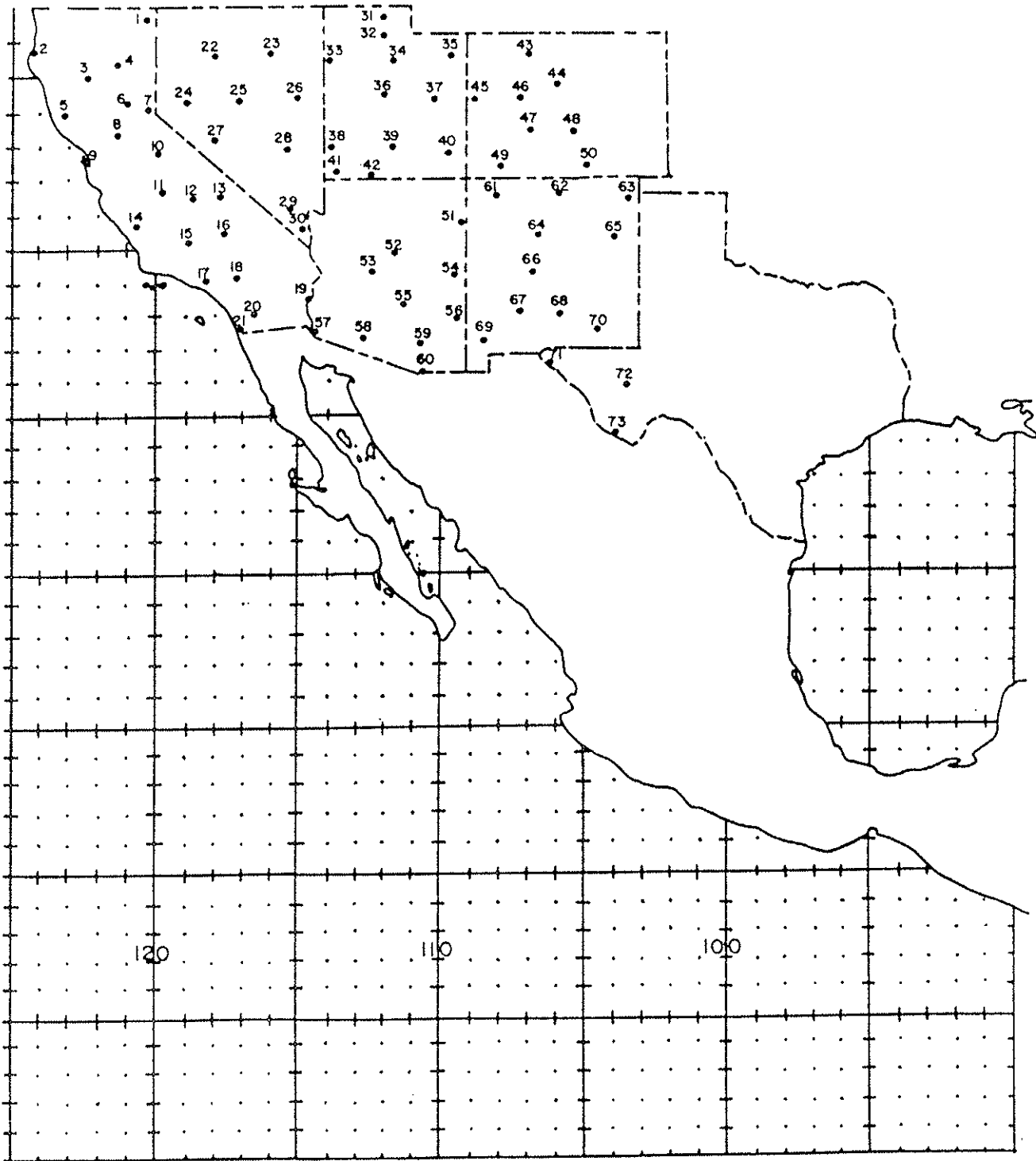
Figure 1. Location of the climatic stations used on the tropical cyclone track and associated rainfall maps. The names which correspond to the numbers are listed in Table 4.
