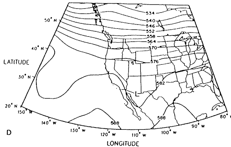
Figure 66. (continued) As in Figure 44.
