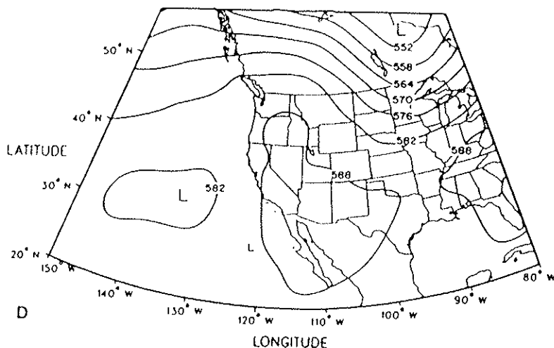
Figure 72. (continued) As in Figure 44.
