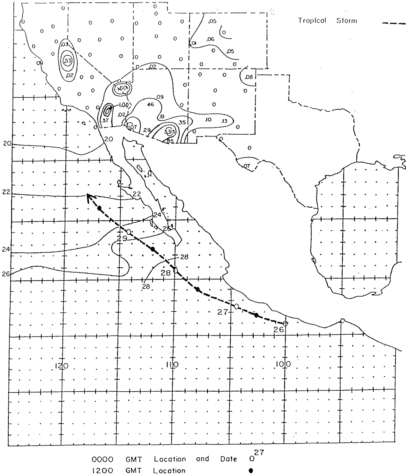
Figure 63. Track of the Tropical Storm of July 26-29, 1958 and associated rainfall in the Southwest. Precipitation totals are in inches and the isohyets are drawn at .01, .25, .50, 1.00, and 2.00 inches. Sea surface temperatures are in °C.
