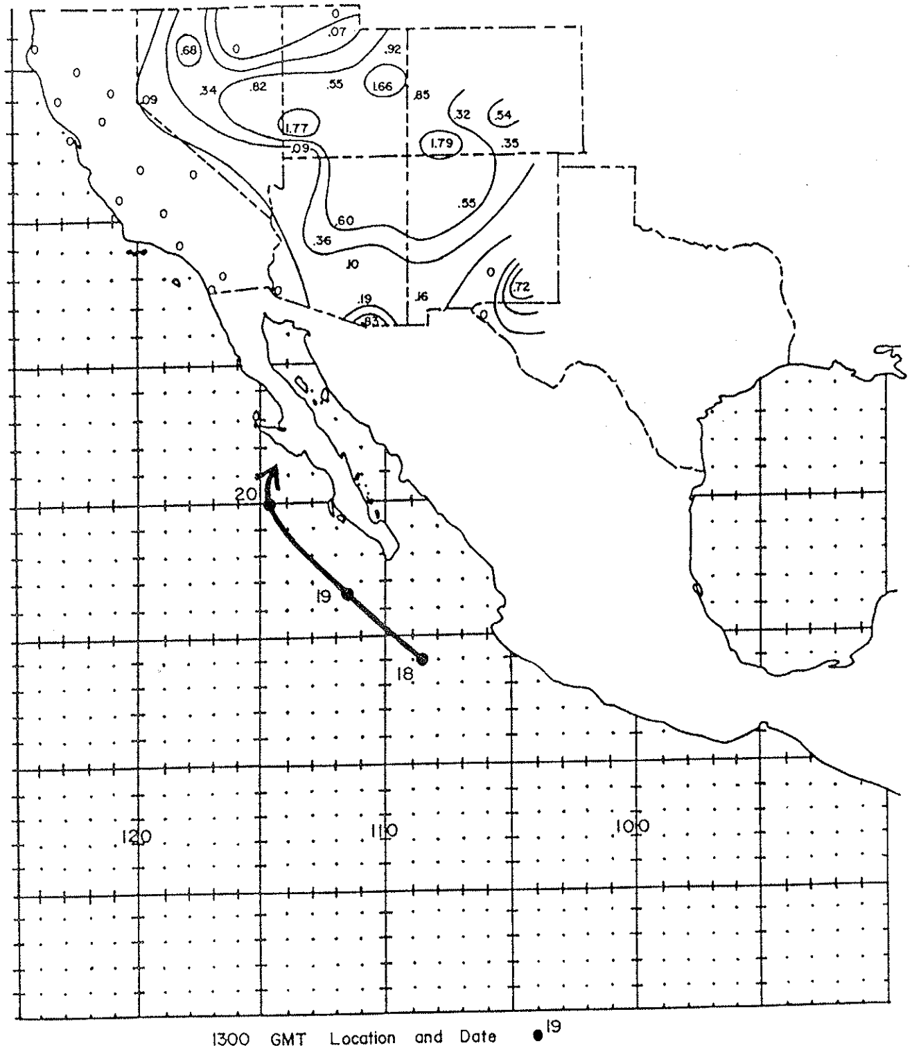
Figure 9. Track of the Tropical Cyclone of September 18-20, 1902 and associated rainfall in the Southwest. Precipitation totals are in inches and the isohyets are drawn at .01, .25, .50, and 1.00 inches.
