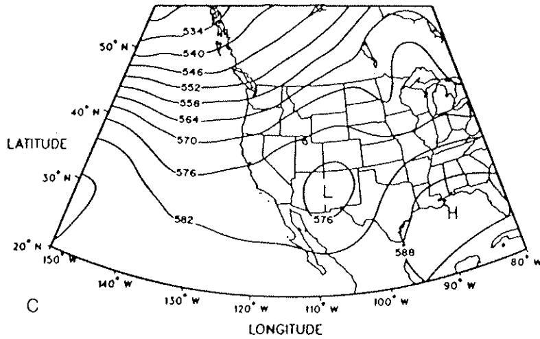
Figure 133. As in Figure 44.
