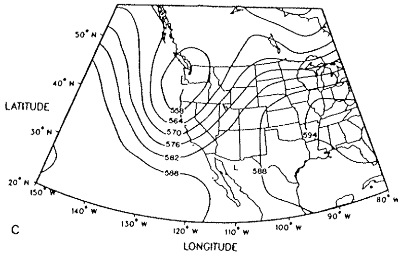
Figure 90. As in Figure 44.
