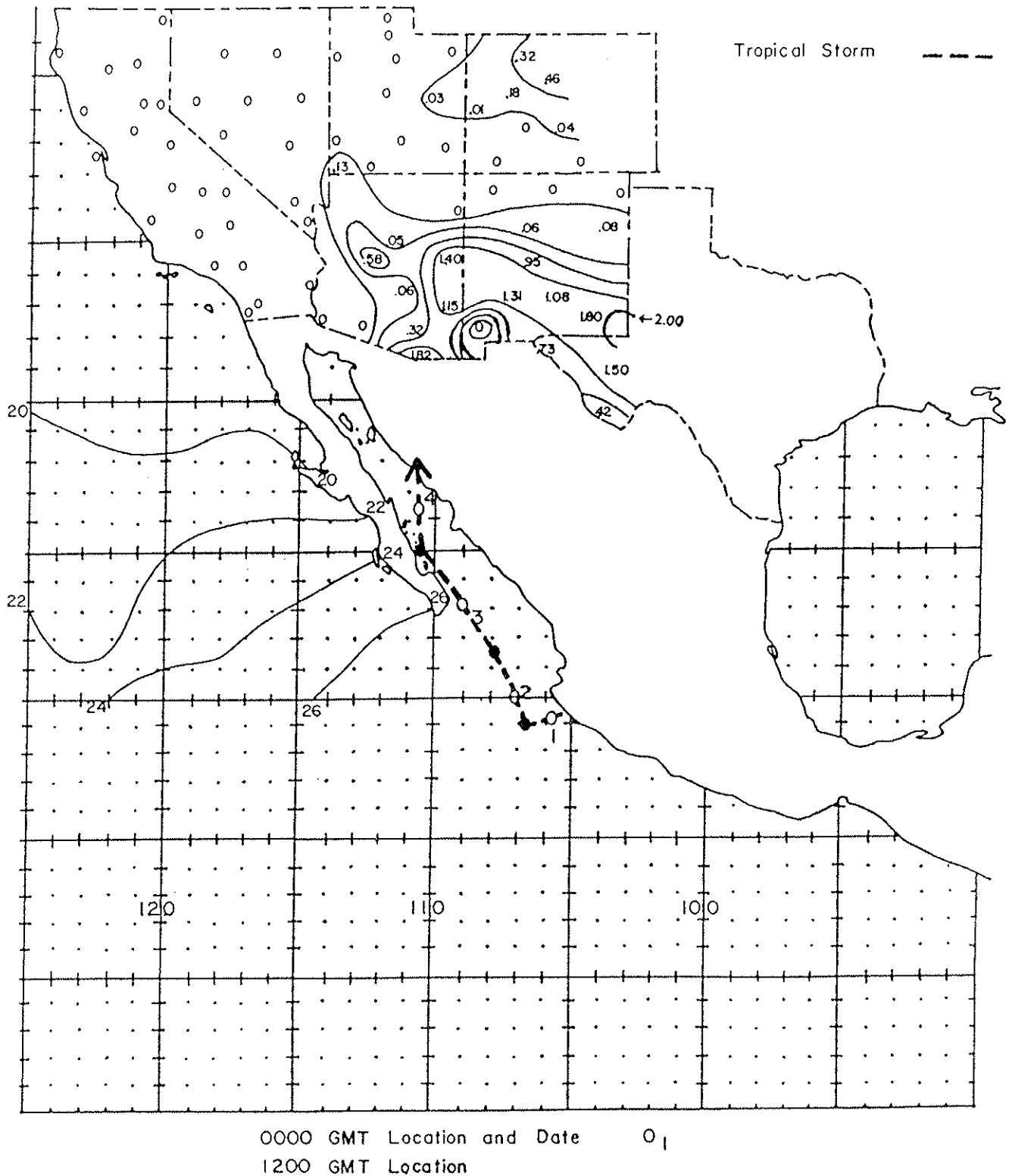
Figure 59. Track of the Tropical Storm of October 1-4, 1955 and associated rainfall in the Southwest. Precipitation totals are in inches and the isohyets are drawn at .01, .25, .50, 1.00, and 2.00 inches. Sea surface temperatures are in °C.
