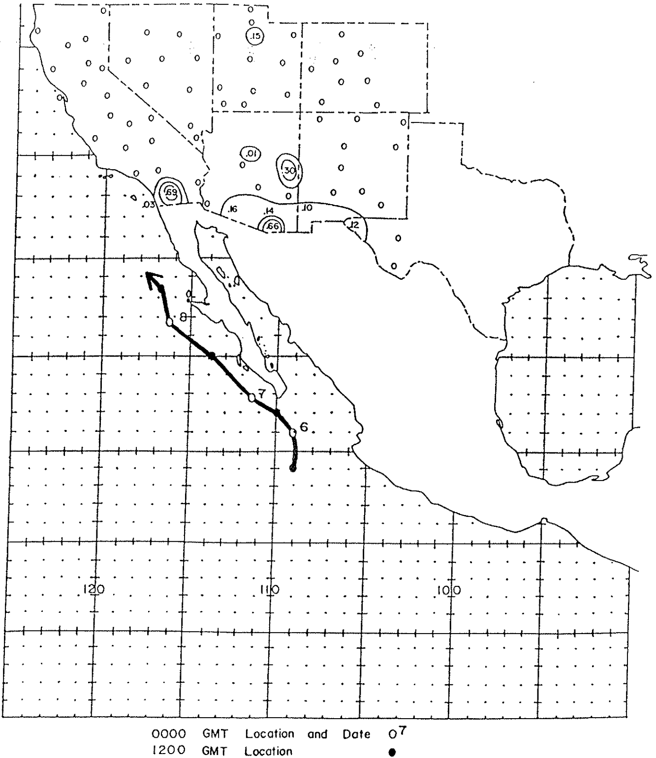
Figure 43. Track of the Tropical Cyclone of September 5-8, 1945 and associated rainfall in the Southwest. Precipitation totals are in inches and the isohyets are drawn at .01, .25, and .50 inches.
