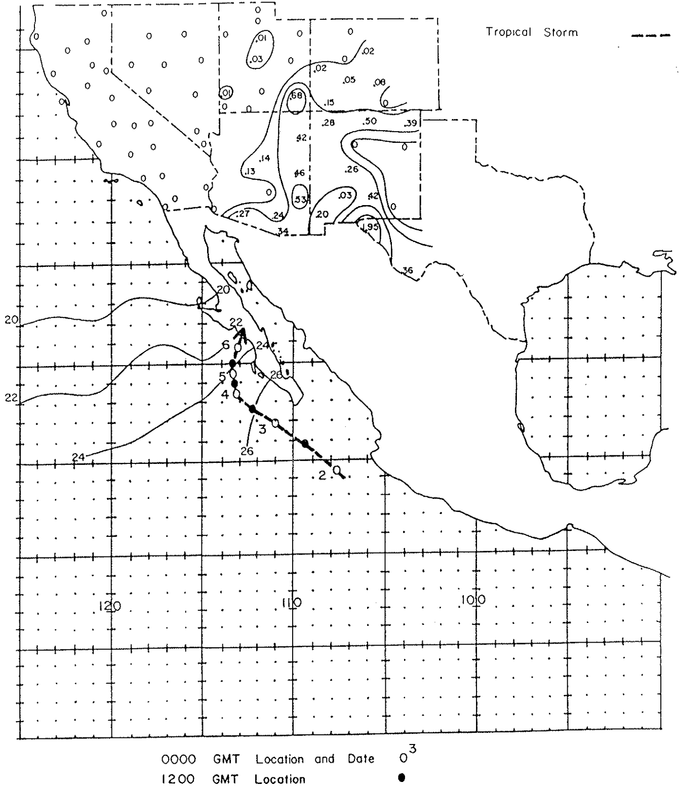
Figure 75. Track of Tropical Storm Bernice; September 1-6, 1962; and associated rainfall in the Southwest. Precipitation totals are in inches and the isohyets are drawn at .01, .25, .50, and 1.00 inches. Sea surface temperatures are in °C.
