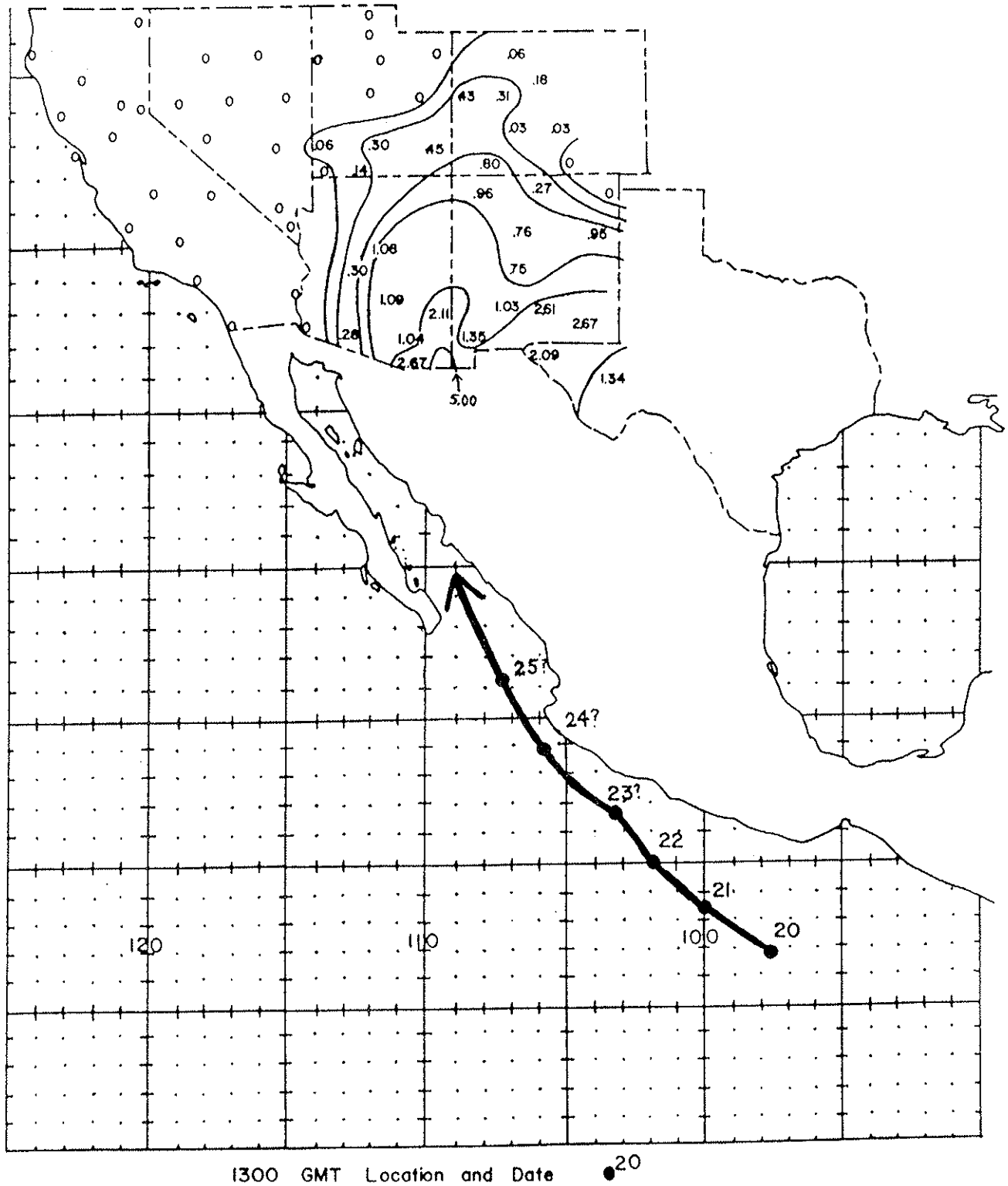
Figure 22. Track of the Tropical Cyclone of September 20-25, 1926 and associated rainfall in the Southwest. Precipitation totals are in inches and the isohyets are drawn at .01, .25, .50, 1.00, 2.00, and 5.00 inches.
