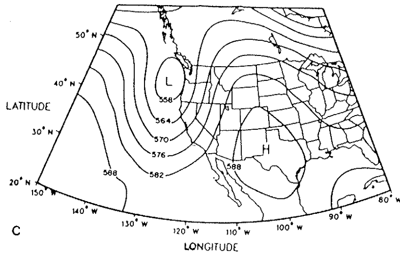
Figure 64. As in Figure 44.
