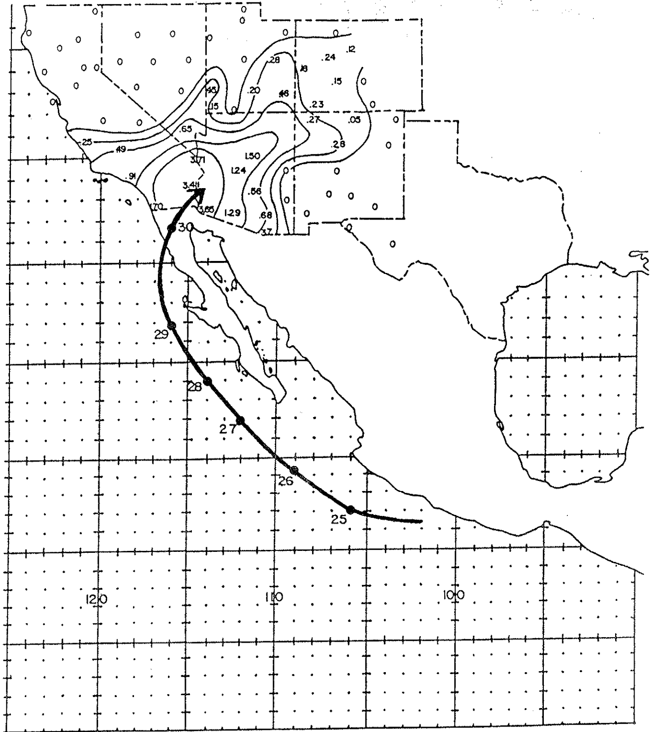
Figure 19. Track of the Tropical Cyclone of September 25-30, 1921 and associated rainfall in the Southwest. Precipitation totals are in inches and the isohyets are drawn at .01, .25, .50, 1.00, and 2.00 inches.
