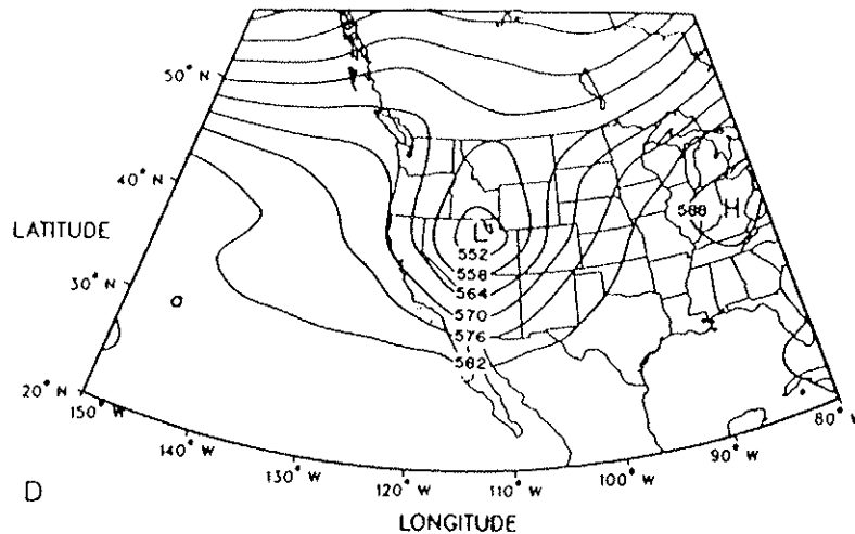
Figure 97. (continued) As in Figure 44.
