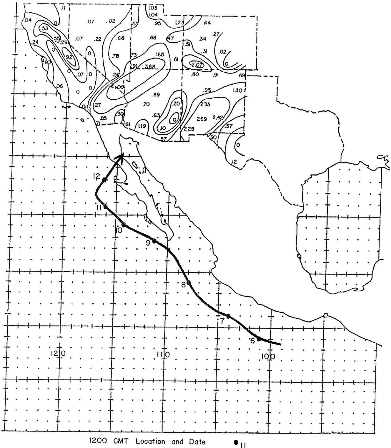
Figure 38. Track of the Tropical Cyclone of September 6-12, 1939 and associated rainfall in the Southwest. Precipitation totals are in inches and the isohyets are drawn at .01, .25, .50, 1.00, and 2.00 inches.
