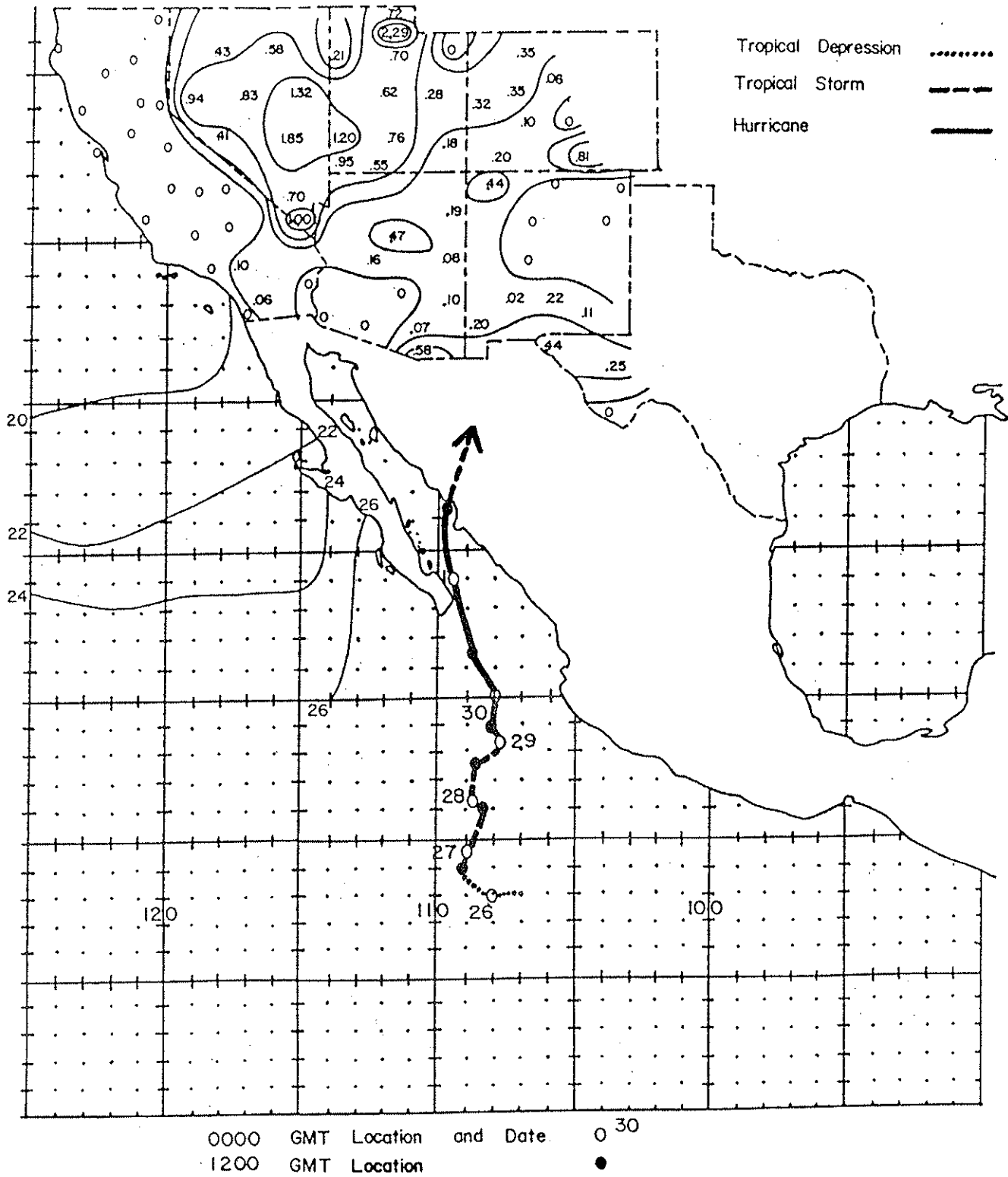
Figure 108. Track of Hurricane Liza; September 25 - October 1, 1976; and associated rainfall in the Southwest. Precipitation totals are in inches and the isohyets are drawn at .01, .25, .50, 1.00, and 2.00 inches. Sea surface temperatures are in °C.
