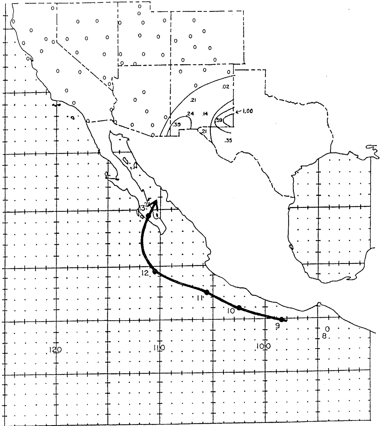
Figure 25. Track of the Tropical Cyclone of October 8-13, 1926 and associated rainfall in the Southwest. Precipitation totals are in inches and the isohyets are drawn at .01, .25, .50, and 1.00 inches.
