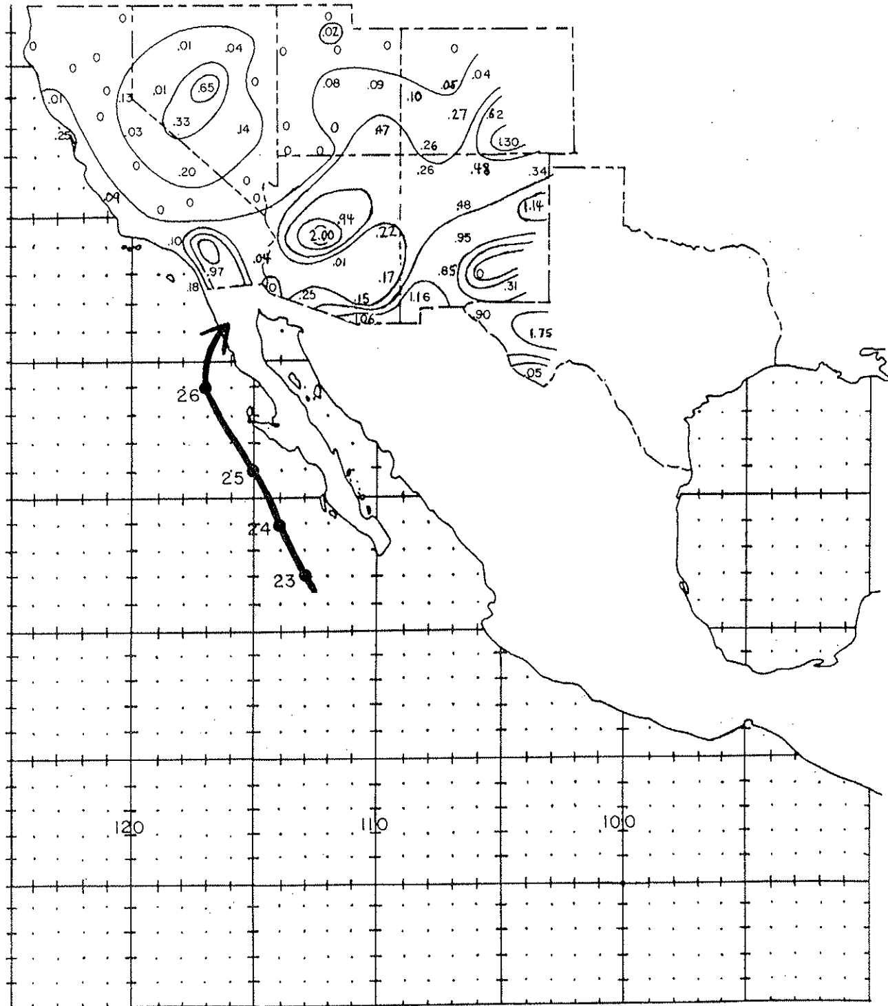
Figure 34. Track of the Tropical Cyclone of August 23-26, 1935 and associated rainfall in the Southwest. Precipitation totals are in inches and the isohyets are drawn at .01, .25, .50, 1.00, and 2.00 inches.
