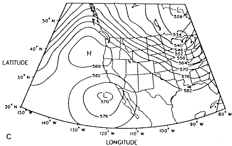
Figure 86. As in Figure 44.
