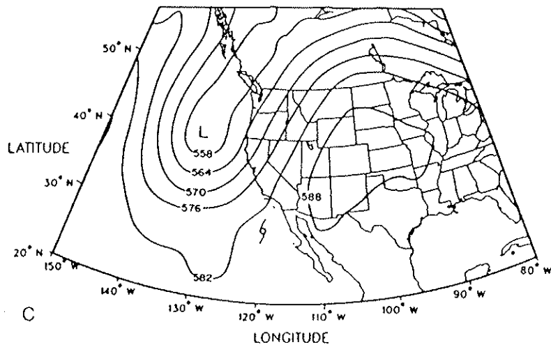
Figure 116. As in Figure 44.
