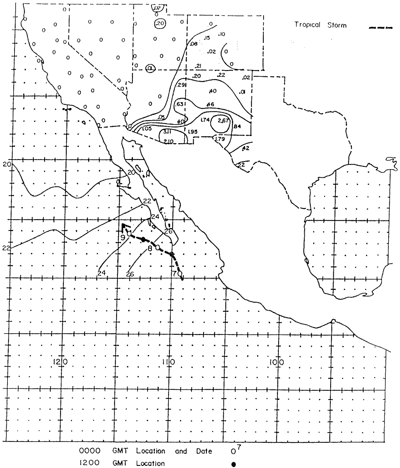
Figure 83. Track of Tropical Storm Tillie; September 7-9, 1964; and associated rainfall in the Southwest. Precipitation totals are in inches and the isohyets are drawn at .01, .25, .50, 1.00, and 2.00 inches. Sea surface temperatures are in °C.
