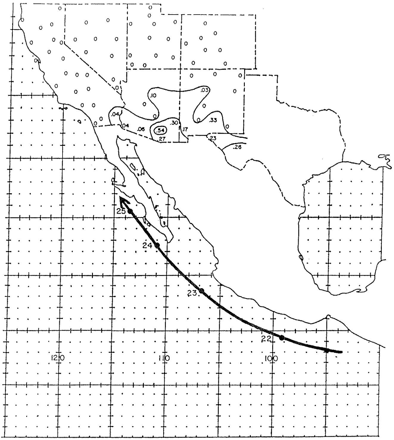
Figure 21. Track of the Tropical Cyclone of October 22-25, 1925 and associated rainfall in the Southwest. Precipitation totals are in inches and the isohyets are drawn at .01, .25, and .50 inches.
