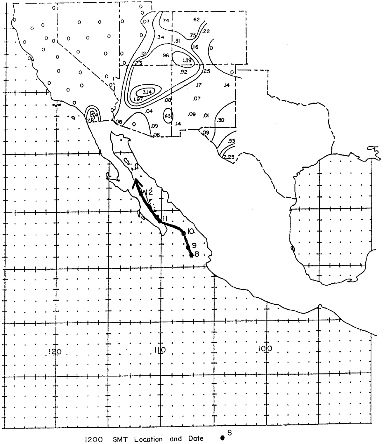
Figure 41. Track of the Hurricane of September 8-12, 1941 and associated rainfall in the Southwest. Precipitation totals are in inches and the isohyets are drawn at .01, .25, .50, 1.00, and 2.00 inches.
