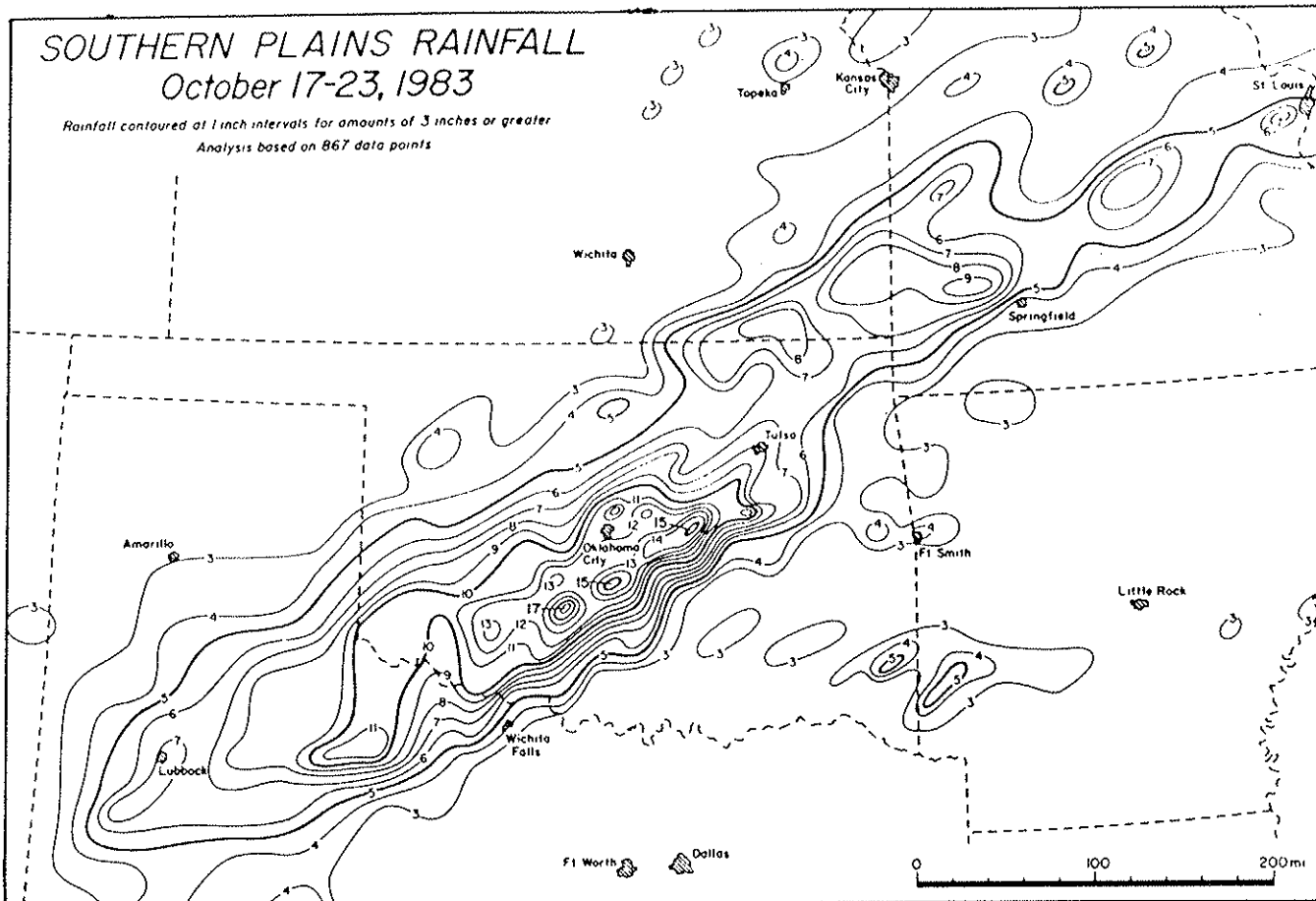
Figure 135. Southern Plains precipitation from October 17-23, 1983 linked to Hurricane Tico; in inches (from Fujita and Stiegler, 1983).
