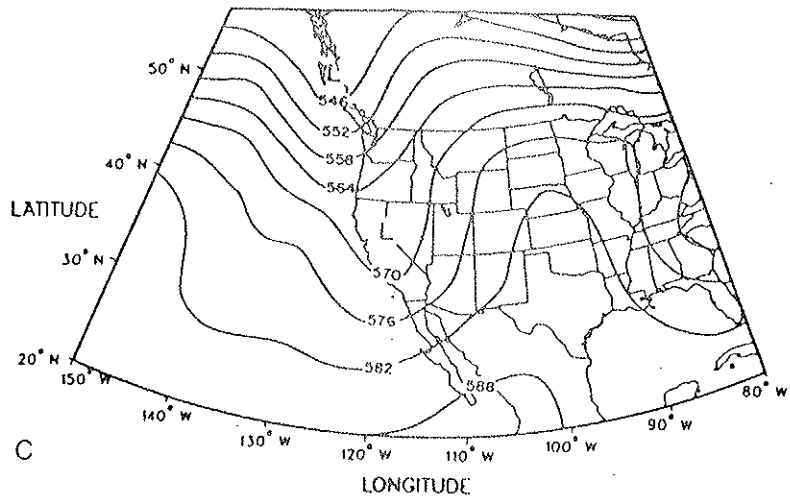
Figure 105. As in Figure 44.
