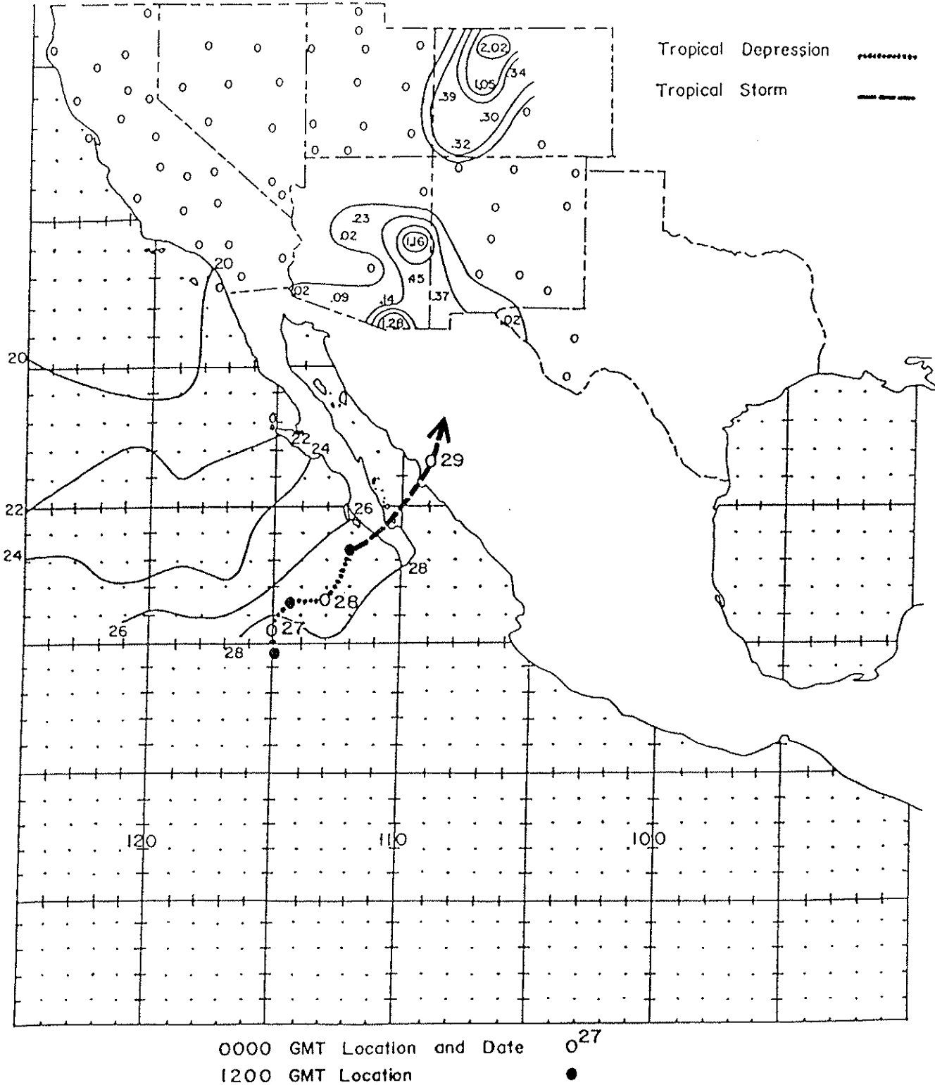
Figure 87. Track of Tropical Storm Kirsten; September 25-29, 1966; and associated rainfall in the Southwest. Precipitation totals are in inches and the isohyets are drawn at .01, .25, .50, 1.00, and 2.00 inches. Sea surface temperatures are in ^{\circ}\text{C} .
