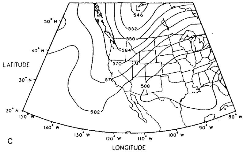
Figure 82. As in Figure 44.
