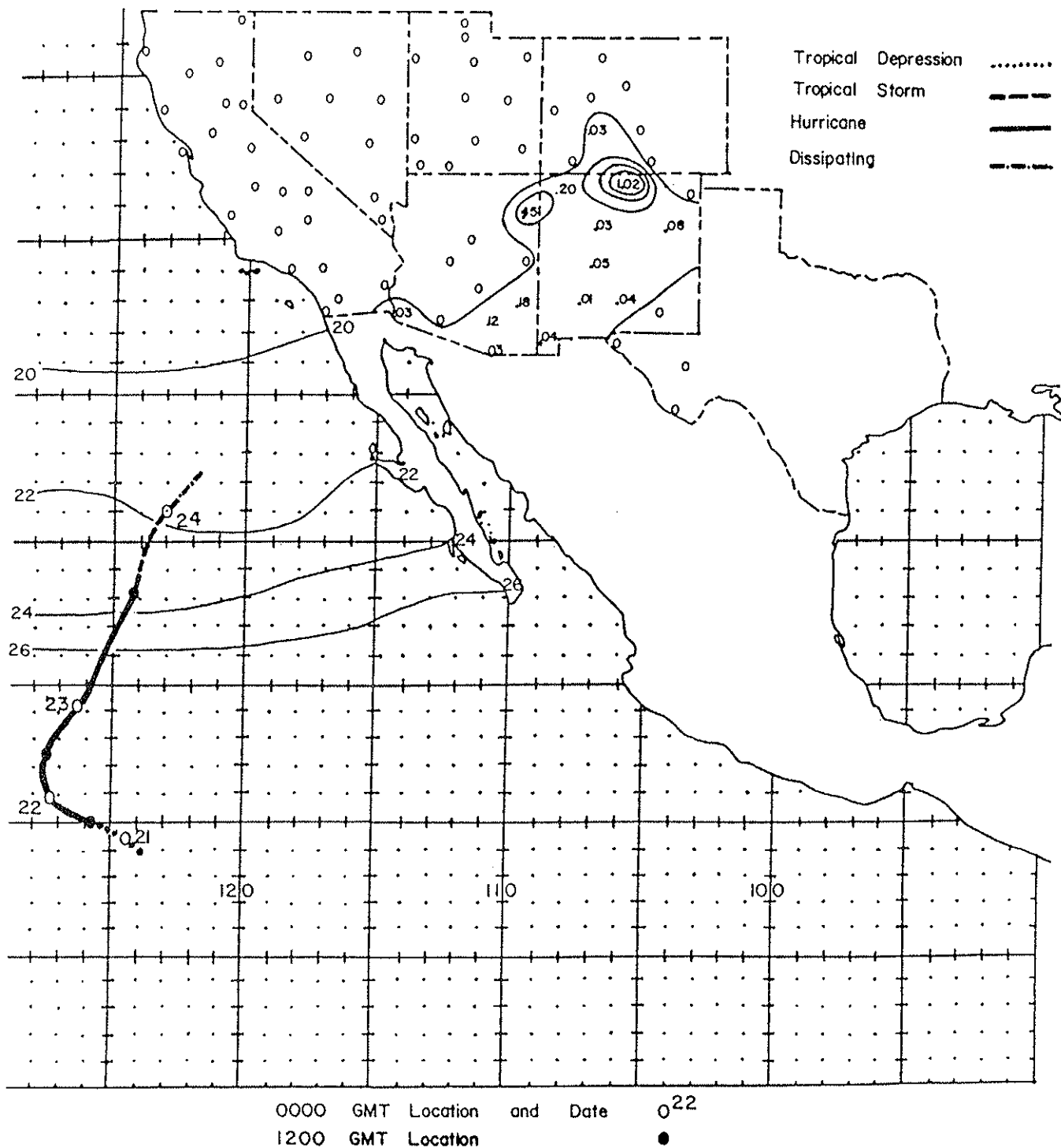
Figure 110. Track of Hurricane Florence; September 20-24, 1977; and associated rainfall in the Southwest. Precipitation totals are in inches and the isohyets are drawn at .01, .25, .50, and 1.00 inches. Sea surface temperatures are in °C.
