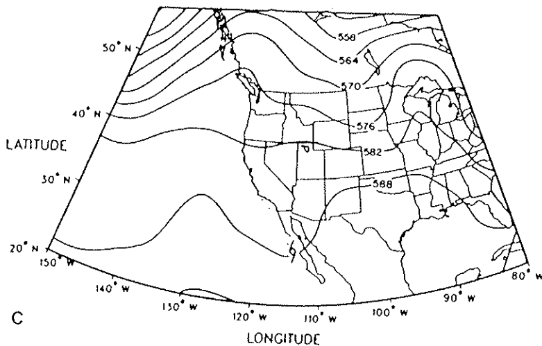
Figure 76. As in Figure 44.
