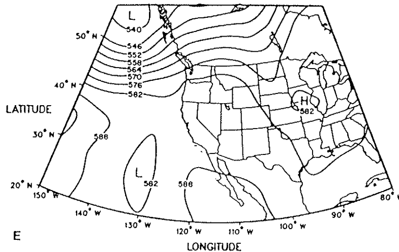
Figure 88. (continued) As in Figure 44.
