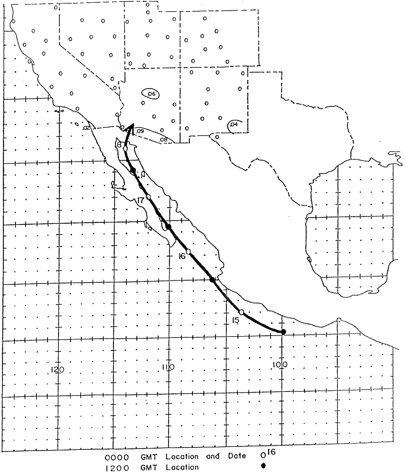
Figure 16. Track (from Court, 1980) of the Hurricane of September 14-18, 1918 and associated rainfall in the Southwest. Precipitation totals are in inches and the isohyet is drawn at .01 inches.
