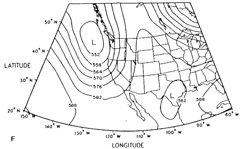
Figure 68. (continued) As in Figure 44.
