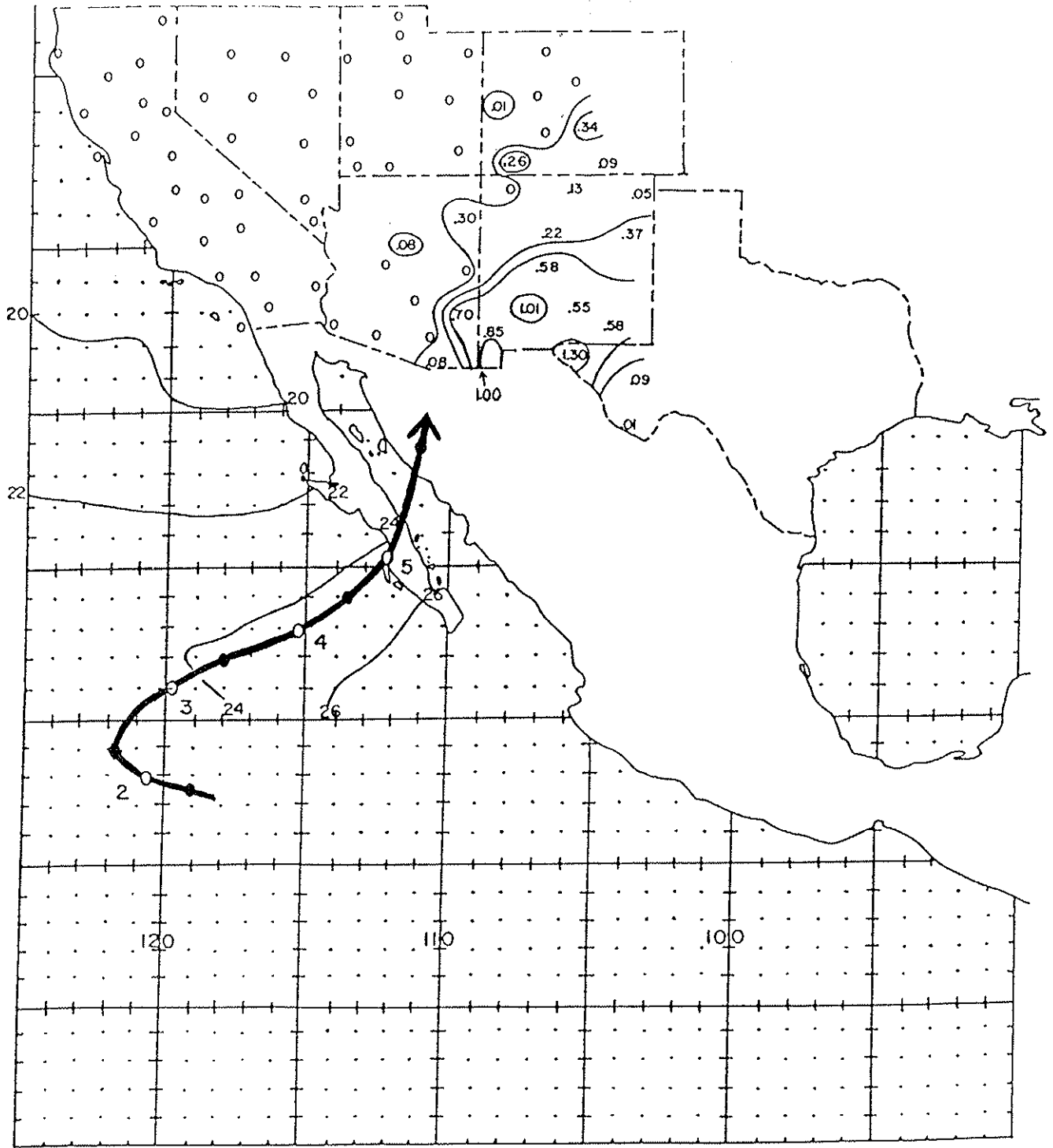
Figure 61. Track of the Hurricane of October 1-5, 1957 and associated rainfall in the Southwest. Precipitation totals are in inches and the isohyets are drawn at .01, .25, .50, and 1.00 inches. Sea surface temperatures are in °C.
