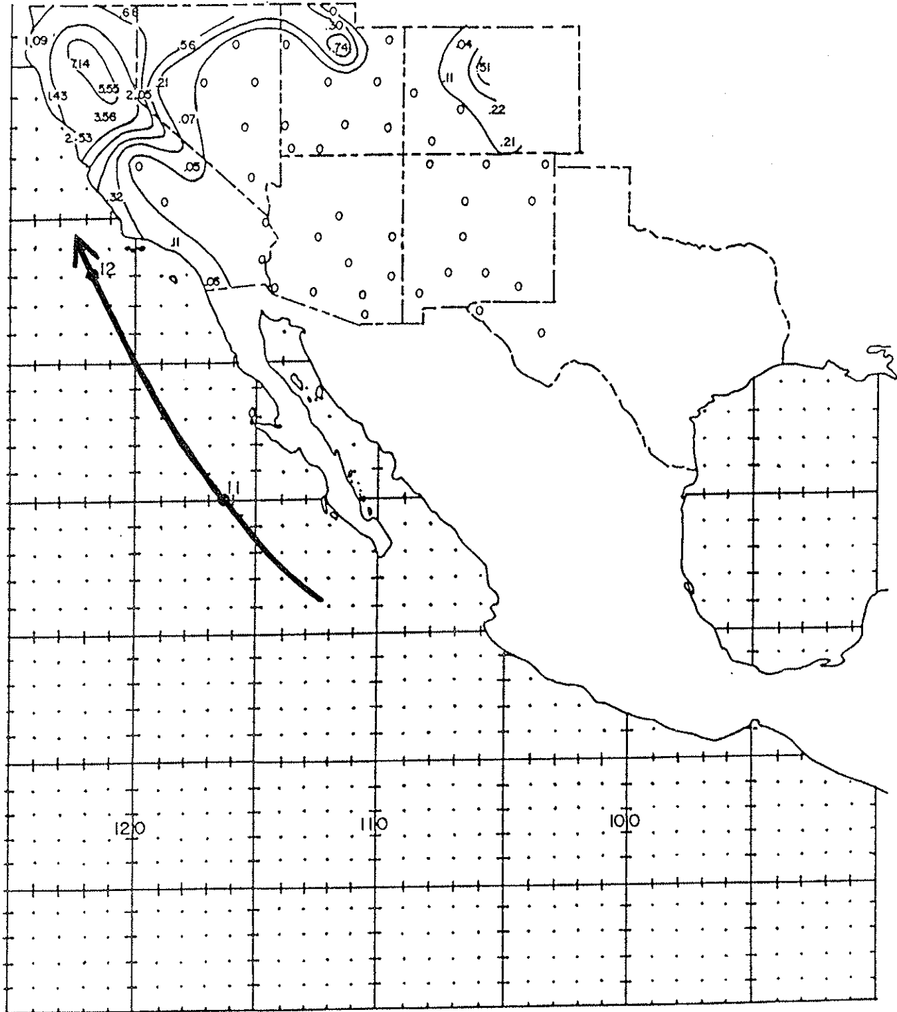
Figure 15. Track of the Tropical Cyclone of September 11-12, 1918 and associated rainfall in the Southwest. Precipitation totals are in inches and the isohyets are drawn at .01, .25, .50, 1.00, 2.00, and 5.00 inches.
