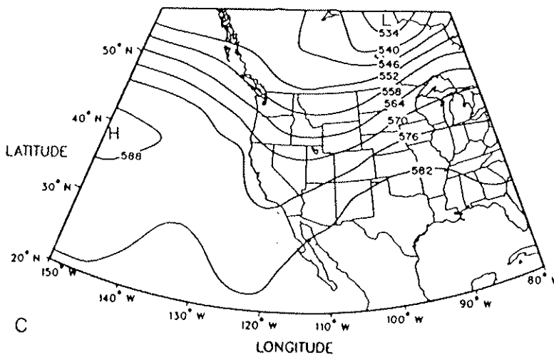
Figure 99. As in Figure 44.
