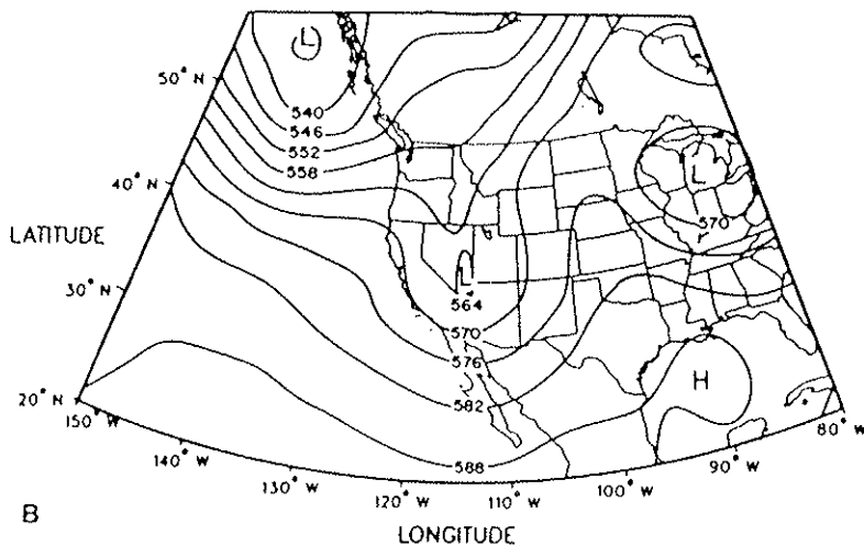
Figure 78. As in Figure 44.
