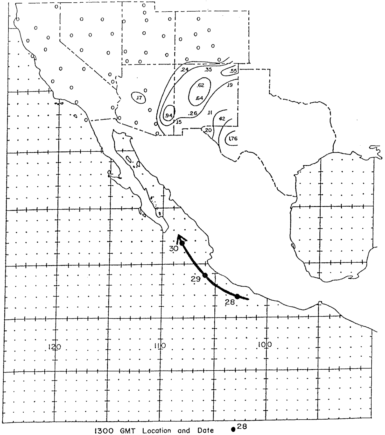
Figure 23. Track of the Tropical Cyclone of September 27-30, 1926 and associated rainfall in the Southwest. Precipitation totals are in inches and the isohyets are drawn at .01, .25, .50, and 1.00 inches.
