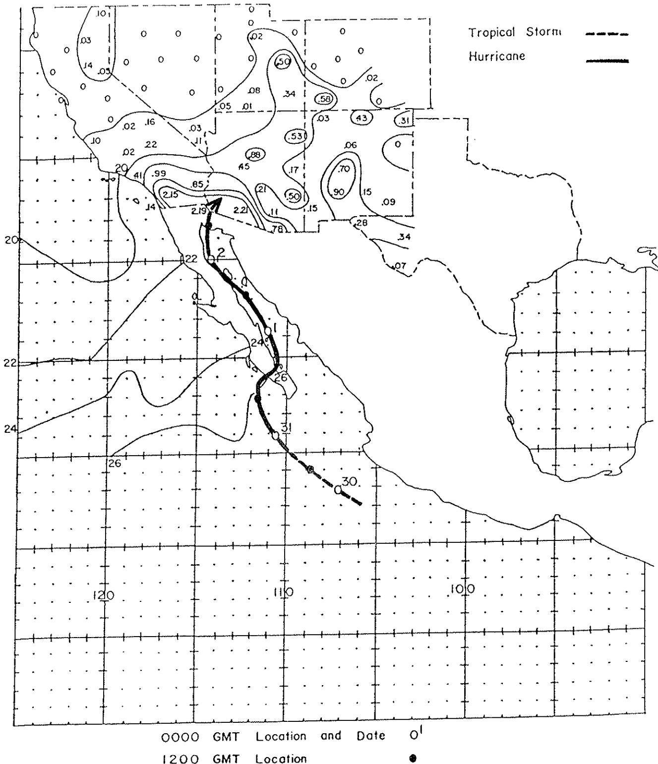
Figure 89. Track of Hurricane Katrina; August 29 - September 2, 1967; and associated rainfall in the Southwest. Precipitation totals are in inches and the isohyets are drawn at .01, .25, .50, 1.00, and 2.00 inches. Sea surface temperatures are in °C.
