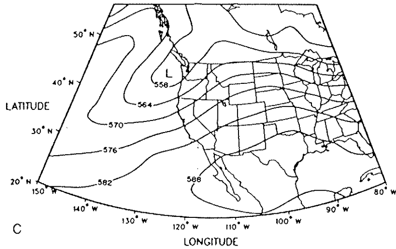
Figure 111. As in Figure 44.
