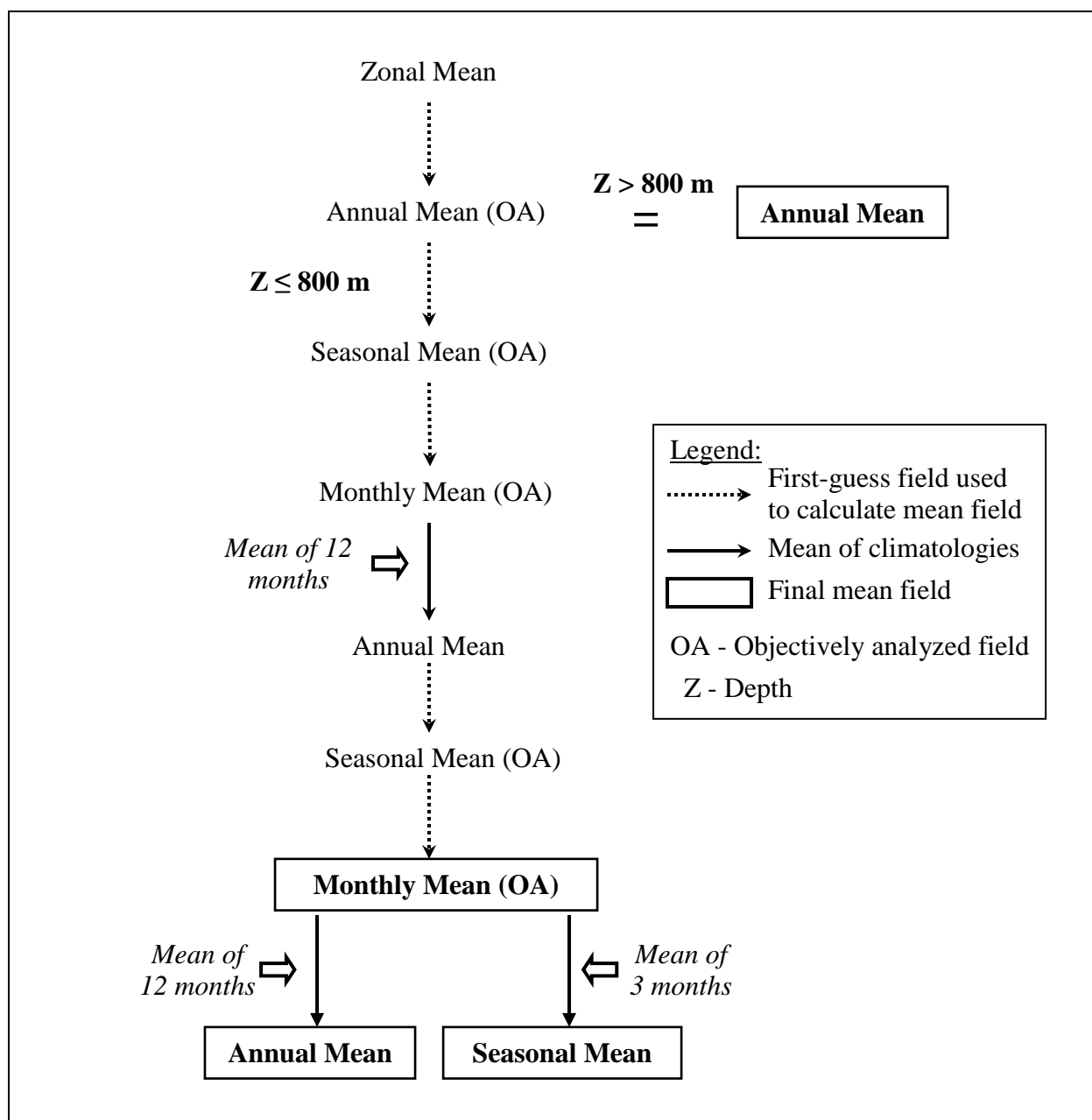
Figure 2. Scheme used in computing annual, seasonal, and monthly objectively analyzed means for phosphate, silicate, and nitrate.
