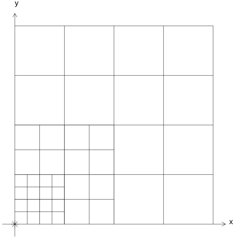
Figure 5. Schematic depiction of the telescoping multigrid structure around map singularity marked by the asterisk. Involutory symmetries that have the singularity as a fixed point imply that it is generally not necessary to completely surround the singularity with grid points; in this depiction one corner of one panel of a square grid is depicted, as might be seen in the cubic or square-dihedron geometries.
