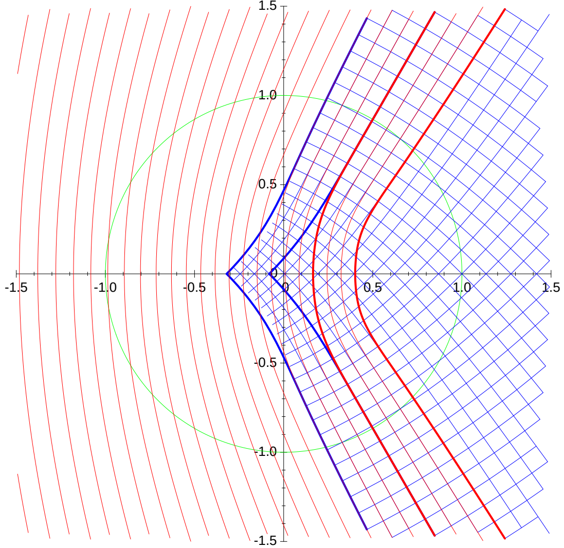
Figure 9. The overset configuration showing both pieces of the modified conformal cubic grid now overlapping within the disc of intervention.
