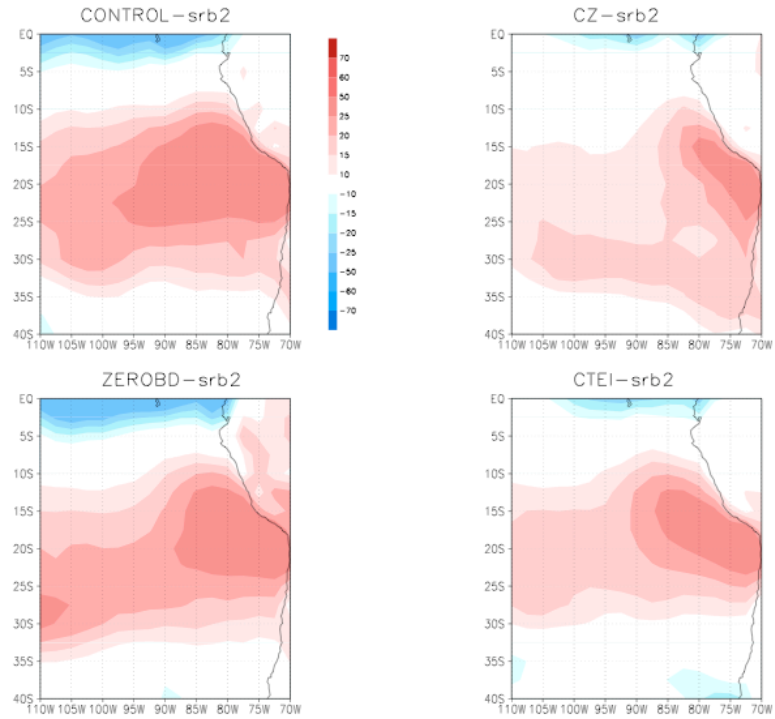
Figure 10. As in Fig.9 except for the longwave radiative flux errors
