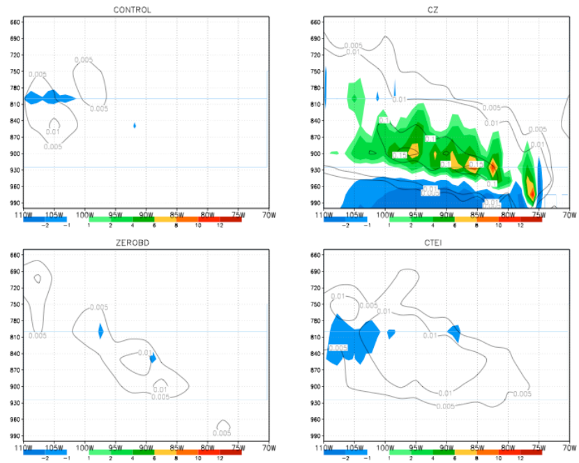
Figure 16. Vertical cross-sections of monthly mean heating rate due to large-scale condensation (K/day) along 20S in shades overlaid with monthly mean cloud water mixing ratios (g/kg) in contours
