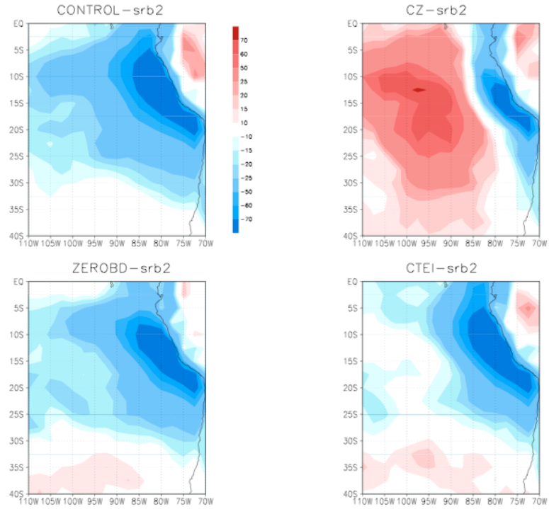
Figure 9. The July 2008 mean upward shortwave radiative flux errors (difference between the simulations and SRB climatology) at the top of the atmosphere in the four experiments.
