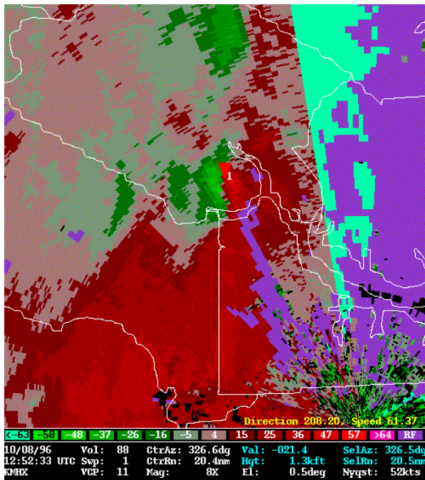
Figure 15. Storm relative velocity from 1252 UTC 8 October 1996 for the KMHX.
