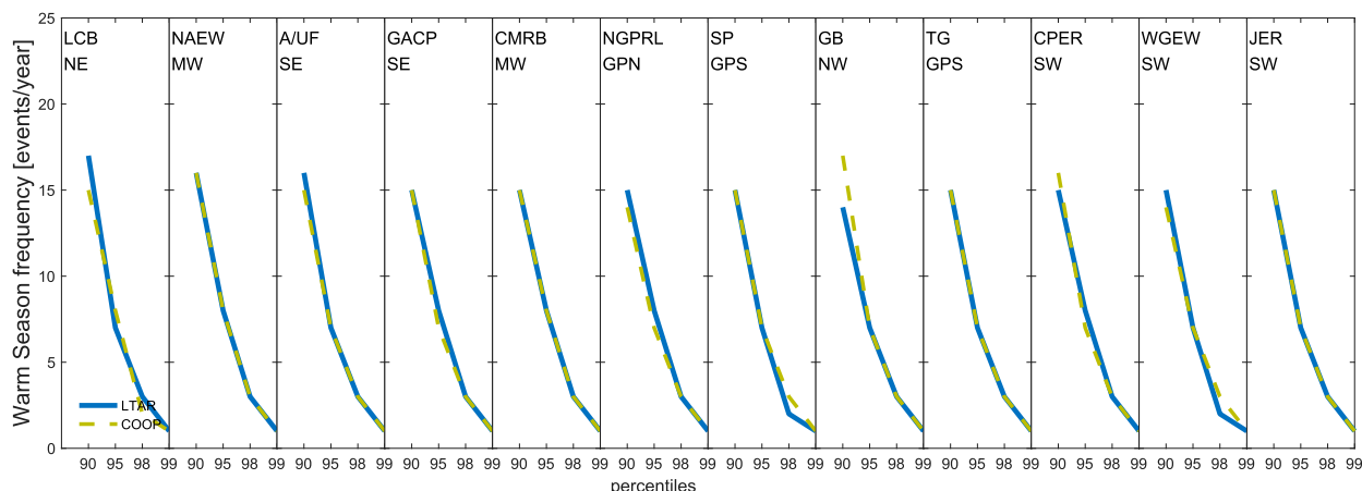
FIG. 8. Frequency of events per year with precipitation exceeding the threshold.
