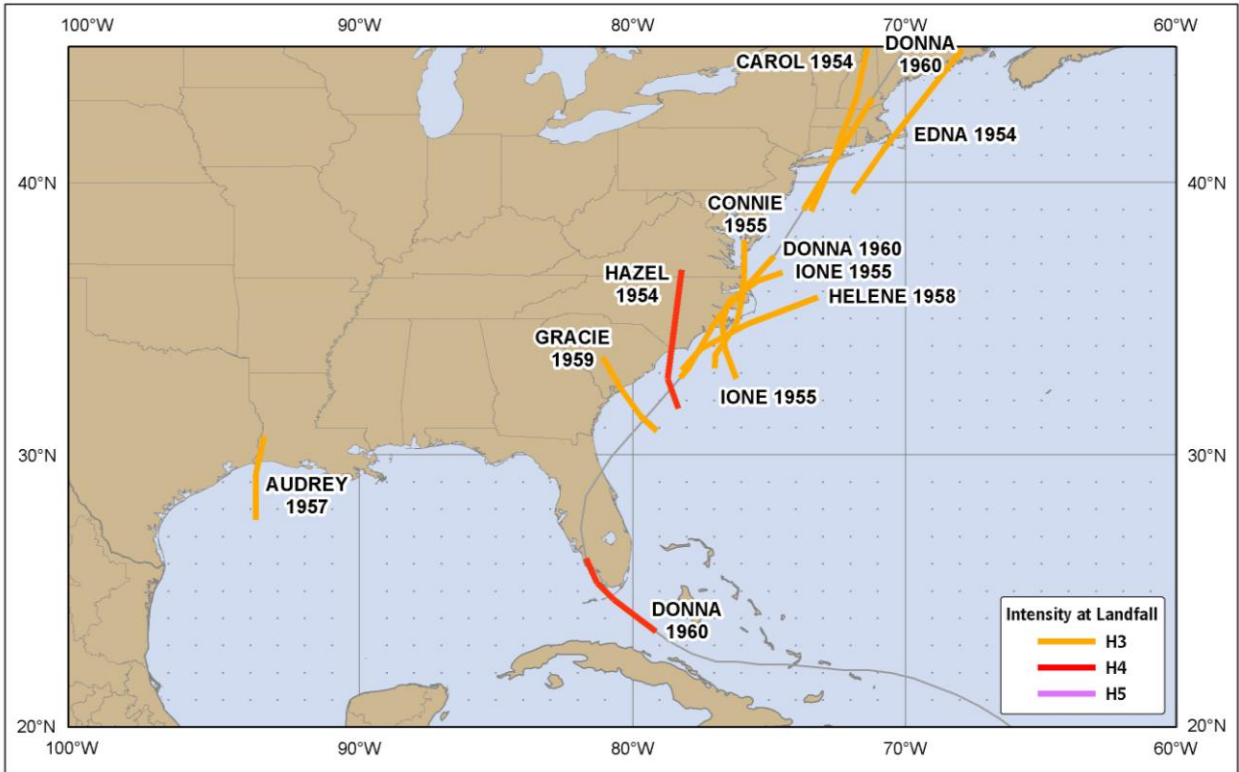
Figure 17. United States major hurricane strikes (category 3 or higher), 1951-1960.
