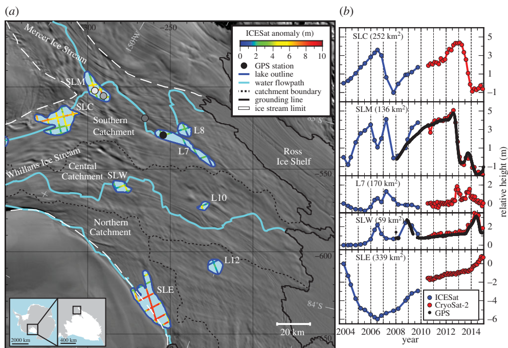
Figure 2. Subglacial water system of the Whillans/Mercer Ice Streams, West Antarctica. (a) Map of the subglacial lakes in the system (blue outlines) annotated with ICESat track segments used to detect them (colour-coded by surface-height change). The lakes are contained within three separate hydrologic systems, and the hydrologic flowpaths and catchment boundaries are shown. (b) Time series of average height change over the four largest lakes from ICESat, CryoSat-2 and GPS. Adapted from Siegfried [23].
