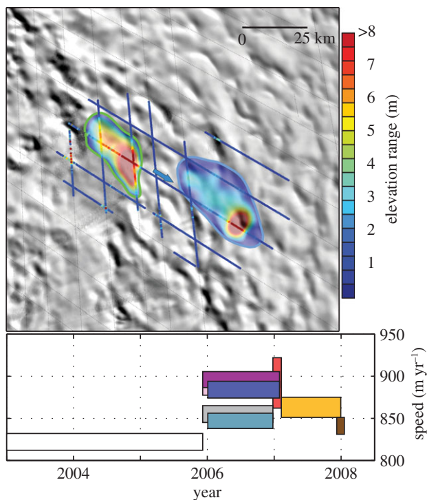
Figure 6. Impact of lake drainage on ice dynamics at Byrd Glacier. Top plot: Map of height ranges for 500 m sections of ICESat tracks, interpreted lake boundaries (green, blue outlines) and height ranges for gridded surface displacements, overlaid on a MODIS mosaic of Antarctica [31]. Surface heights track 0263 decreased over the upper lake and increased over the lower lake between November 2003 and November 2007, which was interpreted as the upper lake draining. Bottom plot: Ice speed at the grounding line from 2003 to 2008. The horizontal bars indicate start and end dates for each pair of observations and the height of each bar represents its associated error. Adapted from Stearns et al. [28].
