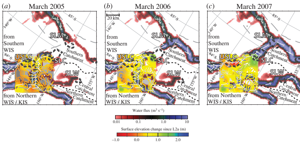
Figure 9. Flow switching on Whillans Ice Stream. Evolution of subglacial water flow routing from (a) March 2005 through (b) March 2006 to (c) March 2007 resulting from a localized thickening of approximately 2 m near lake USLC. Adapted from Carter et al. [45].
