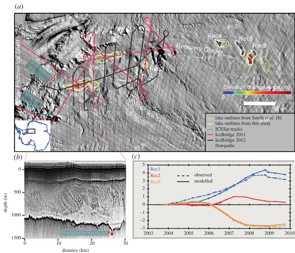
Figure 4. Active lakes of the Recovery Ice Stream, East Antarctica, from ICESat and IceBridge. (a) Map of the six subglacial lakes of lower Recovery Ice Stream (white outlines) annotated with ICESat track segments used to detect them (colour-coded by surface-height change). (b) IceBridge radargram for a track segment across the Shackleton flowpath downstream of Rec1 (see a for location, solid red line) showing features that are not parallel to the bed that may indicate accretion of basal water formed as water travels up and over the saddle in Shackleton Range. (c) ICESat-derived and modelled volume change time series for the three largest Recovery lakes. Adapted from Fricker et al. [11].
