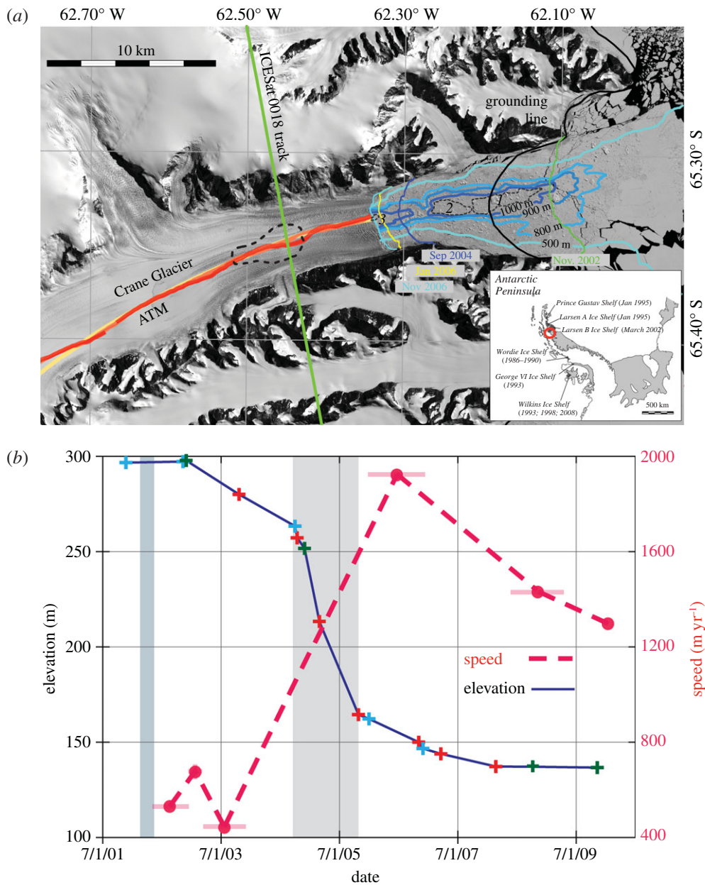
Figure 7. Drainage of Crane Glacier lake on the eastern Antarctic Peninsula. (a) Satellite image map of lower Crane Glacier and fjord. Image is from SPOT-5 high-resolution stereo (HRS) sensor, acquired 25 November 2006. Recent airborne laser altimetry tracks (ATM: 2002, 2004 and 2008 in yellow, orange and red, respectively) and satellite laser altimetry tracks (ICESat: 2003–09, straight green line) showed anomalously large height changes on the glacier. Numbers in the fjord (1, 2 and 3) and dashed outlines represent flat sediment-filled basins interpreted as past subglacial lake deposits, and bathymetry contours are also shown. Grounding line of 1998–2002 is from SAR interferometry [30]. Ice-front locations for floating (November 2002) and grounded ice fronts are shown; since November 2006 the ice-front position has been essentially unchanged. Inset: Locator map of Crane Glacier, within the Larsen B embayment, Antarctic Peninsula. (b) ICESat-derived height for track 0018 across Crane Lake (left-hand scale), and flow speed (right-hand scale). Adapted from Scambos et al. [29].
