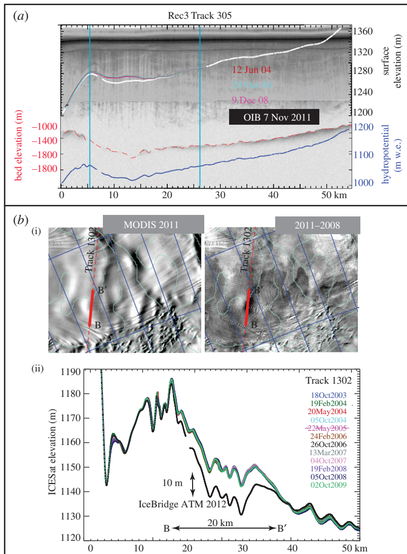
Figure 5. (a) IceBridge radargram acquired along ICESat track 305 on Rec3. The coloured lines towards the top are the surface-height profiles from the ICESat repeats (repeat dates in corresponding colours); white line is the IceBridge ATM surface height. The central line (dashed red) is the bed height picked from the radargram, and the bottom line (solid blue) is the hydropotential. Adapted from Fricker et al. [11]. (b) (i) MODIS image from 2011 and difference image (2011–2008) showing surface deformation along ICESat track 1302, downstream of Rec3. (ii) Repeat ICESat height profiles along track 1302 (colours) and heights derived from the OIB ATM in 2012 showing approximately 10 m surface deformation along a 20 km track segment.
