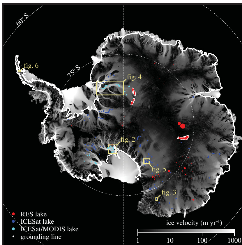
Figure 1. Known subglacial lakes in Antarctica. Locations of Antarctic subglacial lakes, showing lakes studied via RES (red [7]), ICESat (blue [8]), and ICESat and MODIS (cyan [9–11]). Outlines of upper Recovery Glacier lakes from Bell et al. [12] and subglacial Lake Vostok from Studinger et al. [13]; all other RES lakes are represented by circles, with size scaled to lake length [7]. Yellow boxes indicate locations of figures 2–6. Background is InSAR-derived ice velocity [14]. Adapted from Smith et al. [8].
