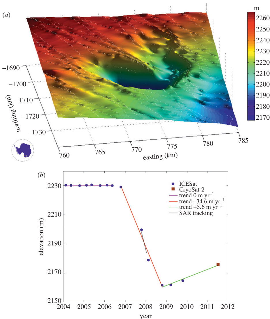
Figure 3. ICESat/CryoSat data over Cook E2 lake in East Antarctica. (a) Surface expression of the drained Cook E2 subglacial lake, mapped by CryoSat-2 SARIn mode data (white dots) from January to November 2011. The shaded surface is a minimum curvature interpolation of the CryoSat-2 data, and illuminated from the east. (b) Evolution of ice surface height above the Cook E2 subglacial lake, from ICESat (2003–2009) and CryoSat-2 (2011) observations. An independent estimate of height change derived from SAR feature tracking is also shown. Adapted from McMillan et al. [19].
