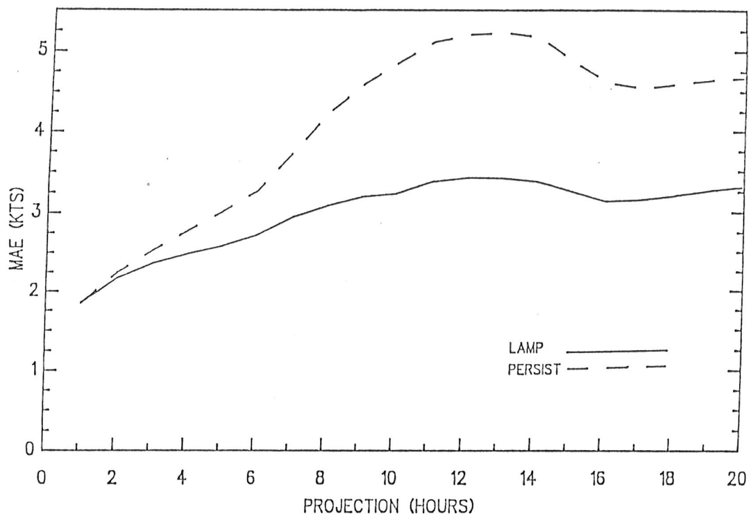
Figure 4. Mean Absolute Error (MAE) for wind speed forecasts from LAMP and Persistence (PERSIST).
