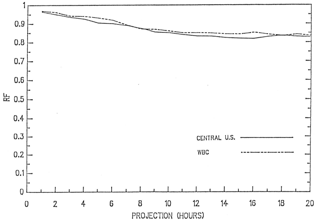
Figure 7. Same as Fig. 6 except for relative frequency for wind direction within 30^\circ when the verifying wind speed was \geq 10 kts.
